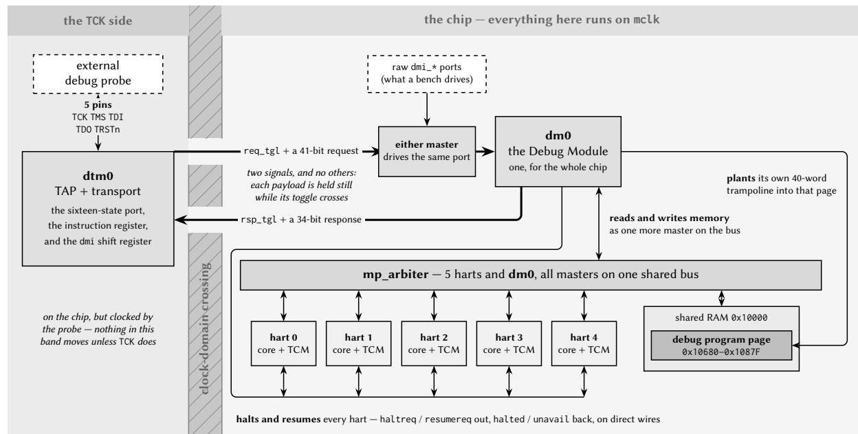
Figure 8: The debug path, from the probe to a hart, in a configuration built with debug support. The transport and the Debug Module sit in different clock domains , and the wall between them is crossed by exactly two signals — one toggle each way, each carrying a payload that is held still while its toggle is in flight. Everything to the right of that wall is ordinary chip fabric, and the one Debug Module reaches it in three ways: it halts and resumes the harts over direct wires, it reads and writes memory as one more master on the same arbiter the harts use, and it plants its own trampoline into the debug program page. The count of hart tiles follows this configuration.
