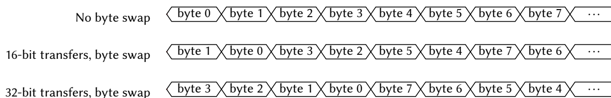
Figure 47: SPI Byte Ordering
