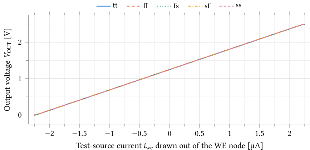
Figure 43: Output voltage against the swept test-source current over the five corners, at R_f = 560 kΩ with the electrode held at v_{cm} = 1.25 V. The bench source draws current out of the WE node, so i_{we} = -I_{WE} against Equation (1) and the slope is +R_f . The corners overlay to the line width because that slope is the feedback resistor, ideal in this bench.
