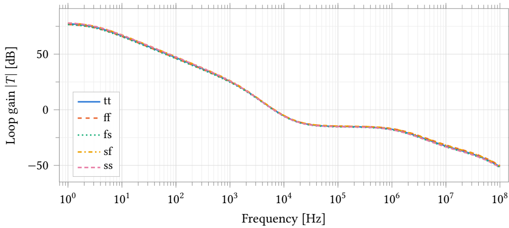
Figure 40: Transimpedance loop gain at maximum gain, by stb through the IPRB_F probe, over the five process corners. R_f = 560 \text{ k}\Omega , C_f = 22 \text{ pF} , electrode randles_cell with R_s = 100 \text{ }\Omega , R_{ct} = 1 \text{ M}\Omega , C_{dl} = 100 \text{ nF} , 25^\circ\text{C} . DC loop gain is 76.5 dB to 78.0 dB and crossover 6.3 kHz to 6.7 kHz. The electrode's solution resistance bounds the noise gain at 1 + R_f/R_s , so the loop closes at 20 dB per decade rather than the 40 dB of the earlier bare-capacitor bench (Section 7.4.3).
