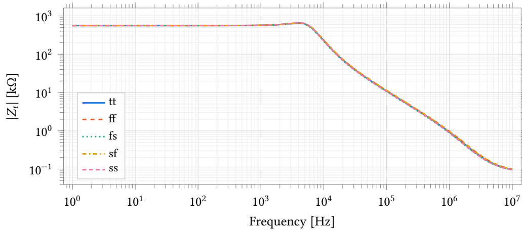
Figure 42: Closed-loop transimpedance magnitude, five corners, conditions as Figure 40. Peaking is 1.2 dB to 1.5 dB at 3.98 kHz and the -3 dB bandwidth 7.2 kHz to 7.5 kHz. Both are set by C_f ; at C_f = 5 pF the same cell peaks 3.0 dB to 3.7 dB with 41.7^\circ to 46.4^\circ of margin.
