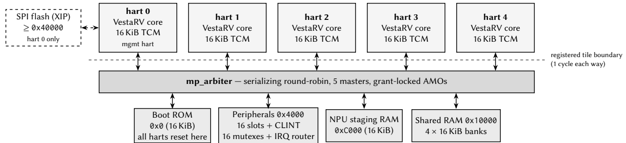
Figure 1: Castalia top-level block diagram (generated from this configuration: 5 harts, 64 KiB shared RAM). Every hart tile couples an unmodified VestaRV core with its private TCM; everything else is reached through the serializing round-robin arbiter.
