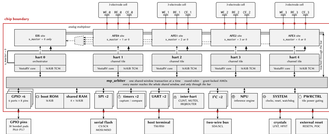
Figure 3: Castalia whole-chip diagram, flat companion to Figure 2: the same generated content on one bus bar and one rank. Every master taps the mp_arbiter bar from above and every peripheral taps it from below, straight up, so there is one bus in this drawing and no second segment of it. A hart box is split into the two things the tile is built from — the VestaRV core and its private TCM. Each of those TCMs is also windowed read-only into the shared map (Section 3), which is why the rank carries no aperture box of its own. Peripheral boxes carry a name and one line only; the addresses are in Section 3, and a \times N in a title — with the offset squares stacked behind the box — is N instances of one peripheral, not one block. Every off-chip partner hangs on a straight vertical wire dropped from the tap above it, entering the partner's top edge off-centre where the partner had to be nudged aside. Each analog site is drawn as a hat on the hart that owns it, with a thin arrow between the two: that arrow is the ownership gate printed inside the site (a comparison against the arbiter's granted-master index), not a wire of its own. The analog IP is not integrated, and no site is reached except through the bar — the grey strip running the length of the row, behind the sites it serves, is that one bus drop. Hart 0's heavy rail under the row is the same comparison from the other side, reaching every site at once. Each channel brings its own three-electrode cell straight up across the boundary on unbroken wires. The dashed trapezoid in the air beside hart 0's site is the analog multiplexer : the shared EIS sweep engine measures through one channel's electrodes at a time, so the four channels' analog paths are its four inputs — each running behind the site boxes at its own height and visible only in the air between them — and its one output goes to the site that carries the engine's registers. It is dashed because that IP is not integrated either, and it is a different kind of thing from hart 0's heavy rail below the row: the rail is digital register access, arbitrated through the bar; the multiplexer is the analog path to the electrodes. Everything drawn is generated from this configuration.
