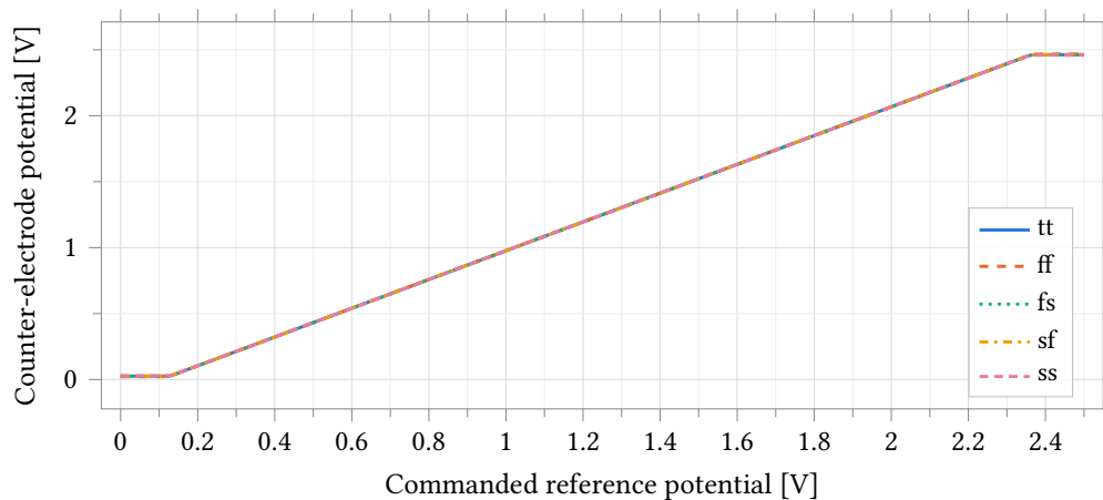
Figure 38: Counter-electrode potential against commanded reference potential over five process corners, cell-drive bench (Figure 37). The amplifier drives a Randles cell with R_{CE} = 1 \text{ k}\Omega , R_u = 1 \text{ k}\Omega , R_{ct} = 10 \text{ k}\Omega , C_{dl} = 1 \mu\text{F} with the working electrode held at 1.25 V, C_L = 5 \text{ pF} , C_c = 500 \text{ fF} , 2.5 V supply; the typical point is at 37 °C and the four skew corners at 25 °C. The central segment rises with slope 12/11, the divider between the 1 k \Omega counter-electrode branch and the 11 k \Omega remainder of the cell; the flat ends are the amplifier against its rails, and their heights are the compliance limits tabulated in Table 41. Over the whole central segment the cell current is set by the cell resistance and the commanded potential, not by the amplifier.
