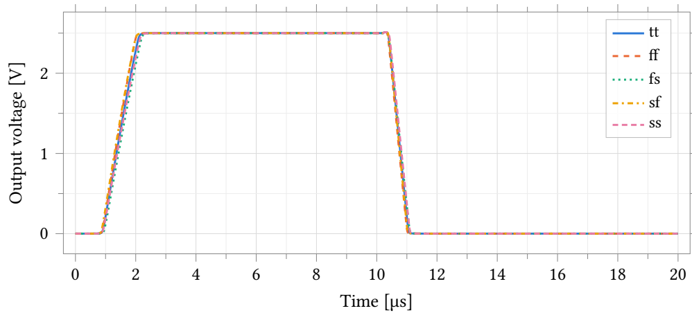
Figure 28: Large-signal response with the amplifier open-loop, driven by a rail-to-rail input pulse into 5 pF, over the five process corners. The falling edge is 1.7 times faster than the rising edge for the same reason the drive is asymmetric: the second stage is class A, and M12 sinks the load with a device eight times wider than the fixed current source M5 that has to source it.
