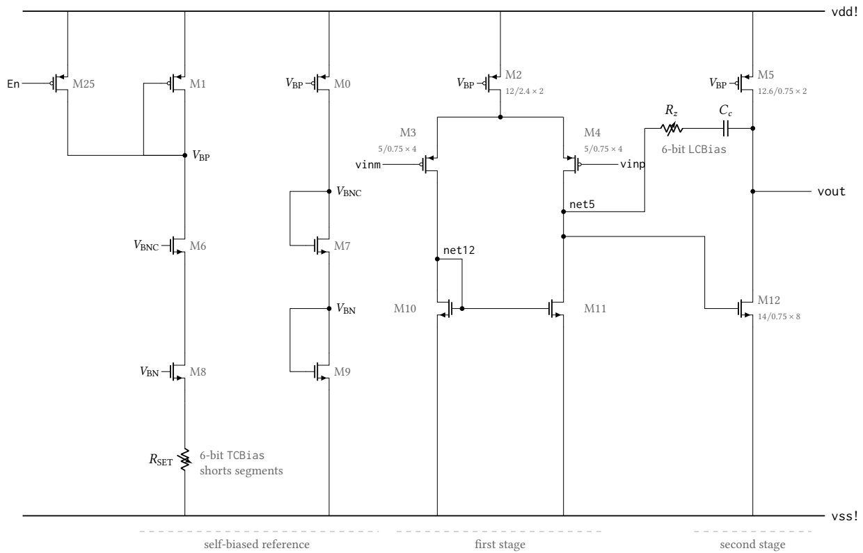
Figure 25: Simplified core of the transimpedance amplifier anatop_tiaamp , drawn from its netlist. It is a two-stage Miller-compensated operational amplifier: a PMOS input pair M3/M4 on tail source M2 with NMOS current-mirror load M10/M11, followed by common-source driver M12 with PMOS current-source load M5, compensated by C_c (a 22.1\text{ }\mu\text{m} square MIM) in series with the nulling resistor R_z from the first-stage output net5 to vout . Device sizes are given as W/L in \mu\text{m} times the multiplicity. The second stage is class A, so its sourcing capability is the fixed current in M5 while its sinking capability is whatever M12 can pull — the asymmetry reported in Table 25. The self-biased reference on the left sets every bias rail from R_{SET} ; M25 pulls V_{BP} to vdd to power the amplifier down. Both resistor strings are drawn as single trimmable resistors: each is a segmented poly ladder with one NMOS shunt switch per trim bit.
