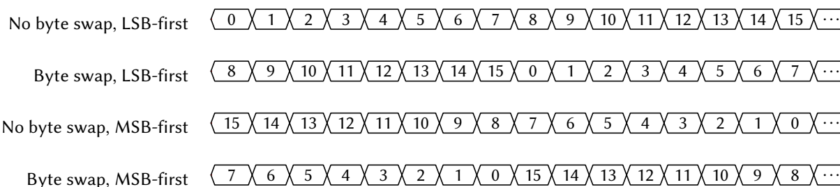
Figure 36: SPI Bit Ordering (16-bit transfer)
