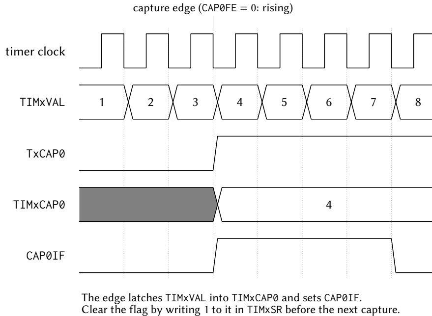
Figure 42: Input capture. The selected edge on TxCAP0 latches the live TIMxVAL into TIMxCAP0 and sets CAP0IF; the flag must be cleared by writing 1 to it in TIMxSR before the next capture event.
