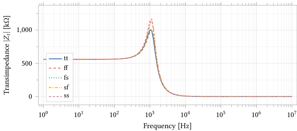
Figure 30: Transimpedance |Z_t| = |V_{OUT}/I_{WE}| of the closed transimpedance stage against frequency, over the five process corners, at the maximum gain setting ( R_f = 560 \text{ k}\Omega ) with 1 \mu\text{F} of double-layer capacitance at the working electrode. The response is flat at 560 \text{ k}\Omega to about 200 \text{ Hz} , then peaks to 1.00 \text{ M}\Omega to 1.17 \text{ M}\Omega near 1 \text{ kHz} before rolling off. That peak is a marginally stable loop rather than a design intent, and it is caused by the electrode capacitance and not by the amplifier: C_{dl} rolls the feedback factor off from 0.28 \text{ Hz} , so the loop closes at roughly 40 \text{ dB} per decade.
