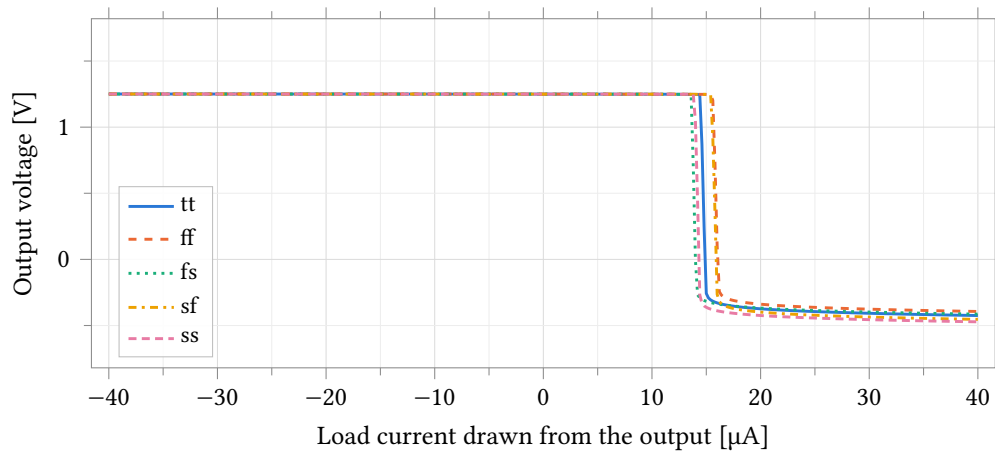
Figure 27: Output voltage of the amplifier in unity feedback as a DC load current is drawn from its output, over the five process corners. Positive current is drawn out of the output node, so the amplifier must source it; the collapse at 13.6 \mu\text{A} to 15.6 \mu\text{A} is the class-A second stage running out of the fixed current in M5. In the sinking direction the output holds within 0.8 mV of v_{cm} all the way to the -40 \mu\text{A} end of the sweep, so the sinking capability is bounded below by the sweep and not measured.
