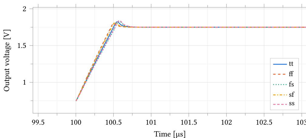
Figure 29: Rising edge of a 1 V step ( v_{cm} \pm 0.5 V) in unity feedback into 5 pF, over the five process corners. The window is 3.5 \mu s around the edge at 100 \mu s; the falling edge at 1.1 ms is outside it. The output slews for about 0.4 \mu s, overshoots once by 5.0 % to 9.0 % of the step and recovers without ringing — the excursion is slow recovery, not small-signal ringing, which is what the 88° phase margin of Table 22 predicts.
