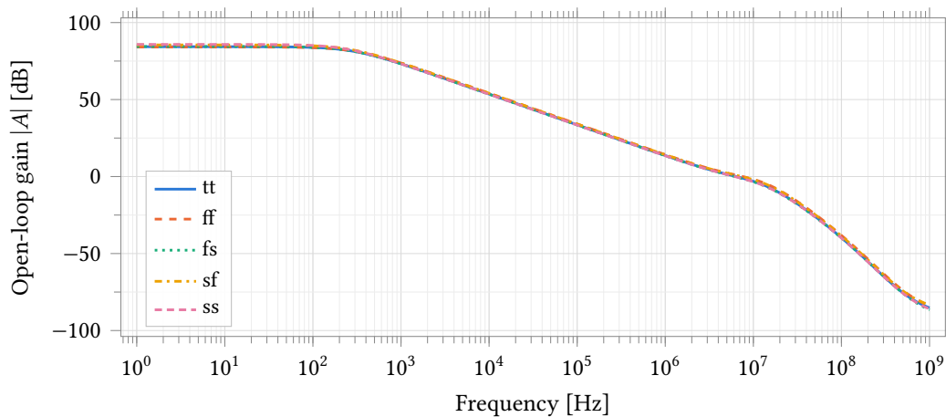
Figure 26: Open-loop gain of the transimpedance amplifier over the five process corners, by stb analysis through the feedback probe with the amplifier in unity feedback and a 5 pF load. Miller compensation places the dominant pole near 200 Hz and gives a single-pole roll-off to a 6.2 MHz to 7.6 MHz crossover; the corners overlay to within 1.7 dB of DC gain. This is the amplifier’s own response. The loop that closes around the electrode is a different loop, and it is not this well behaved — see Figure 30.
