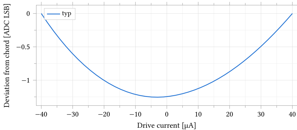
Figure 33.49: Drive nonlinearity of the bottom code ( N = 0 , R \approx 19.6 \text{ k}\Omega ): voltage deviation from the endpoint chord over \pm 90\% of full scale ( \pm 40 \mu\text{A} ), typical corner, expressed in 1.592 \text{ mV ADC LSB} . All ten bypass gates are closed at this code and carry the full signal current; their on-resistance rises with the terminal's excursion from V_{\text{CM}} , so the chord, pinned at the sweep endpoints where that excursion is largest, overestimates the mid-range voltage by up to 1.25 \text{ LSB} , and the deviation is bowl-shaped with a slight skew from the gates' voltage asymmetry. The same measurement at N = 63 and N = 319 , where the ladder dominates and current is 20\text{--}100\times smaller, stays below 0.004 \text{ LSB} and is tabulated, not plotted.
