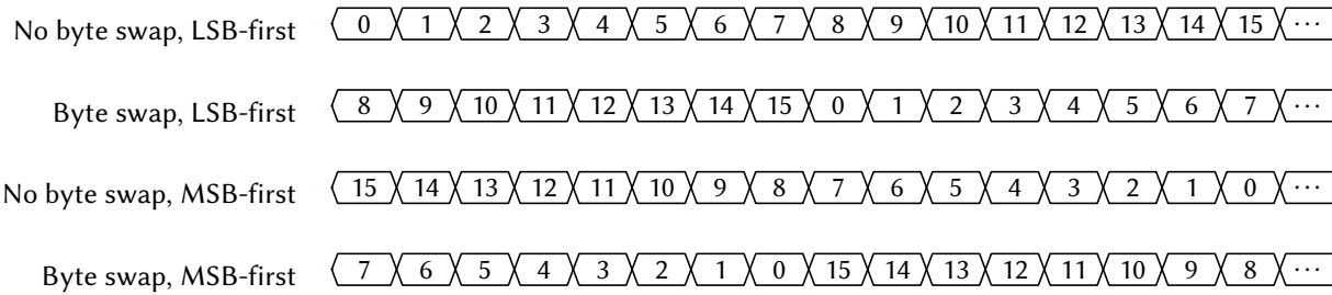
Figure 15: SPI Bit Ordering (16-bit transfer)
