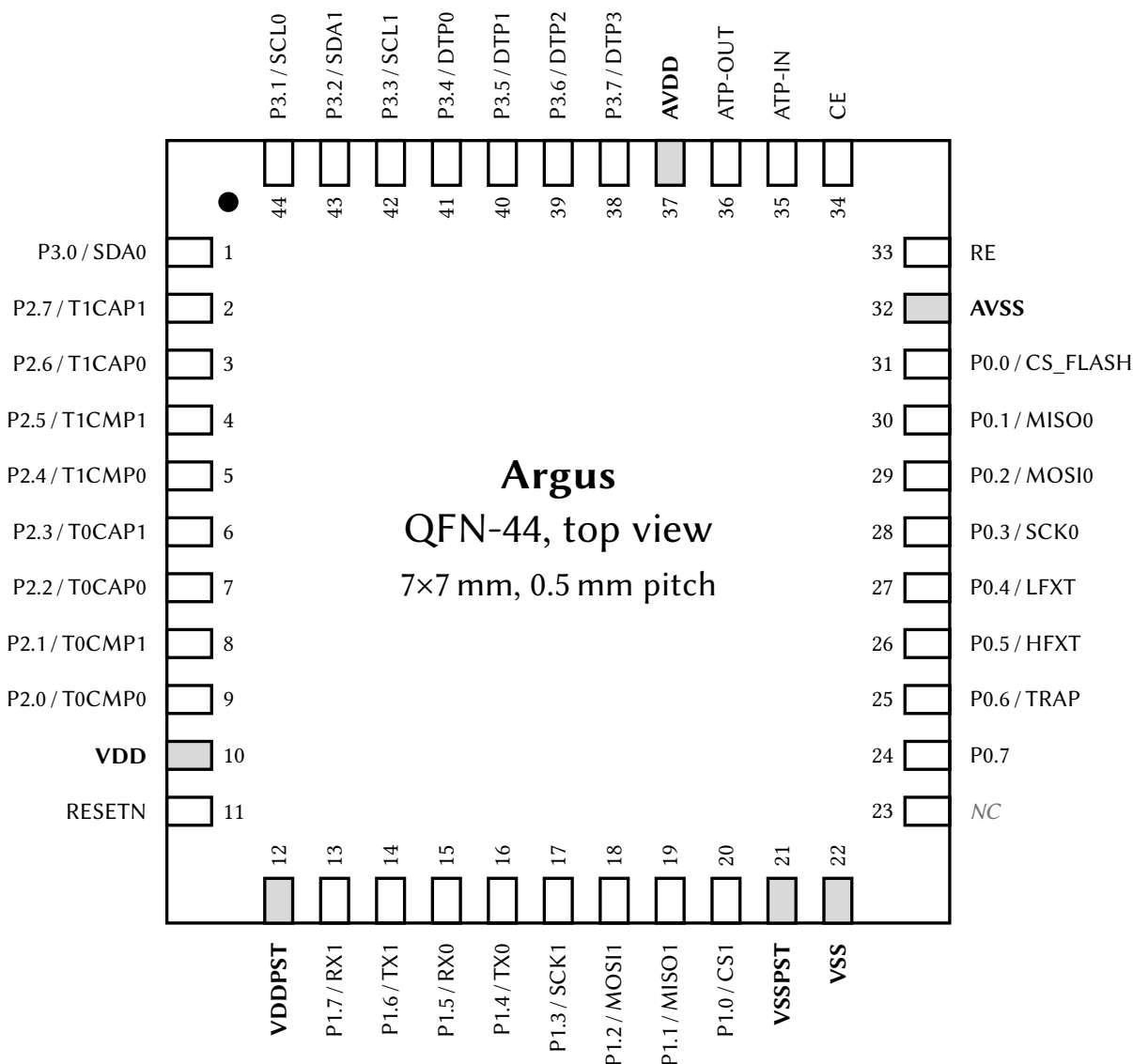
Figure 3: QFN-44 pinout, top view (7 × 7 mm, 0.5 mm pitch). Each pin is labeled with its pad name and, for GPIO pins, its AF0 (reset-selected) alternate function; power-rail pins are shaded and bold. The full per-pin alternate-function matrix is in Table 5.
