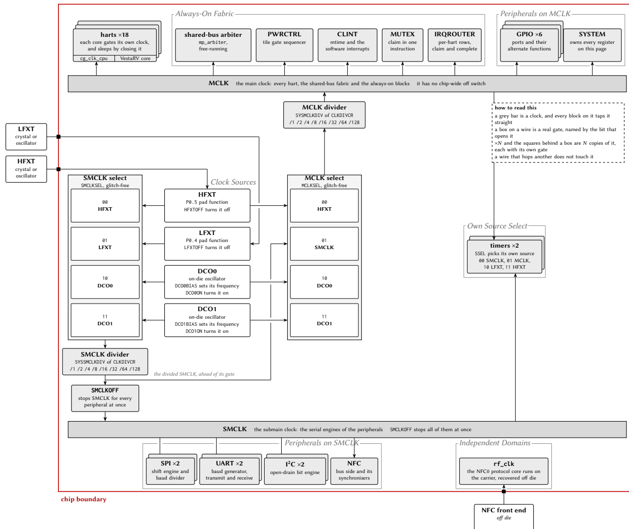
Figure 22: The MCU clock system, generated from this configuration. The layout is a mirror: the sources stand in one column, in the order SMCLKSEL enumerates them, the SMCLK chain runs left out of that column and down into its own bar, and the MCLK chain runs right out of it and up into its own, so every source leg is a straight horizontal at its own row. Each select box prints every code it has, with the name of what that code picks, and those rows are built from the register model itself rather than drawn by hand. One code is not a source: MCLKSEL 01 takes SMCLK, tapped after the SMCLK divider and before the SMCLKOFF gate, which is why stopping SMCLK never stops MCLK; it is the one wire in the drawing that has to leave its row, and it hops the legs it crosses rather than touching them. A source that either select is using stays enabled whatever its own bit says. Every block on a bar taps it straight up or straight down; the sleep gate is drawn where the hardware puts it, inside each core, so the stack of 18 harts is a stack of 18 gates. A block with a select of its own names every code it has and taps the two bars it can reach, so the crystal sources it may also pick are named in its box rather than drawn as two more wires across the page. The blocks under Independent Domains are on neither bar: they are clocked from outside this tree entirely, and SYSCLKCR does not reach them. The register interface of every peripheral is clocked from MCLK even where its engine runs on SMCLK, which is why a peripheral stays readable with SMCLK stopped.
