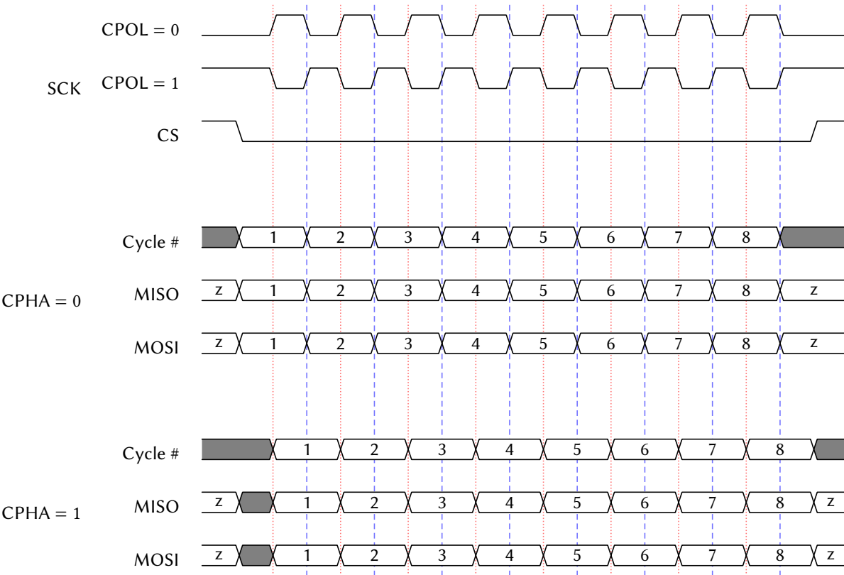
Figure 13: SPI Timing Diagram
