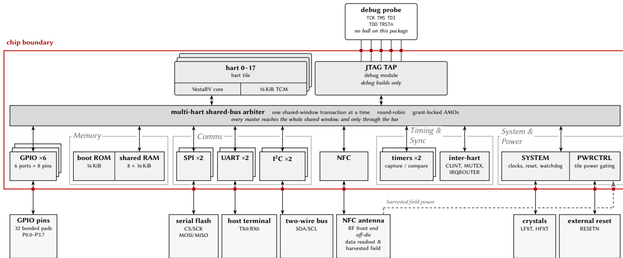
Figure 2: Argus whole-chip diagram, flat companion to Figure 1: the same generated content on one bus bar and one rank. The bar is the mp_arbiter entity of the RTL. Every master taps it from above and every peripheral taps it from below, straight up, so there is one bus in this drawing and no second segment of it. A hart box is split into the two things the tile is built from – the VestaRV core and its private TCM. Peripheral boxes carry a name and one line only; the addresses are in Section 3, and a \times N in a title – with the offset squares stacked behind the box – is N instances of one peripheral, not one block. The rank is grouped by type: the grey headings, and the thin outlines round every type that has more than one box or compartment, are organisation only – every block under them is an arbiter slave in its own right, tapping the bar on its own wire. Every off-chip partner hangs on a straight vertical wire dropped from the tap above it, entering the partner’s top edge off-centre where the partner had to be nudged aside. The JTAG/debug column and the NFC block are drawn solid in every build, whether or not this configuration contains them: what a given build actually has is the debug.enable and peripherals.nfc knobs of Table 1, and the JTAG column prints debug builds only in the box where this build has no debug module in it. The one stroke in the drawing that still changes with the configuration is the harvested-supply rail, drawn dashed where this build does not run the chip off the field. The Debug Module is one more master on the bar, reached over five JTAG pins from an off-chip probe, and is present in debug-enabled builds only. NFC has two roles and this view draws both: its digital core reads the tag through the bar like any peripheral – the RF front end is off-die – and on a field-powered board the harvested field is the chip’s supply , which is the heavy grey rail running along the off-chip band into PWRCTRL’s PGOOD and boot-strap taps, whose boot gate holds every hart in reset until that supply is good. Everything drawn is generated from this configuration.
