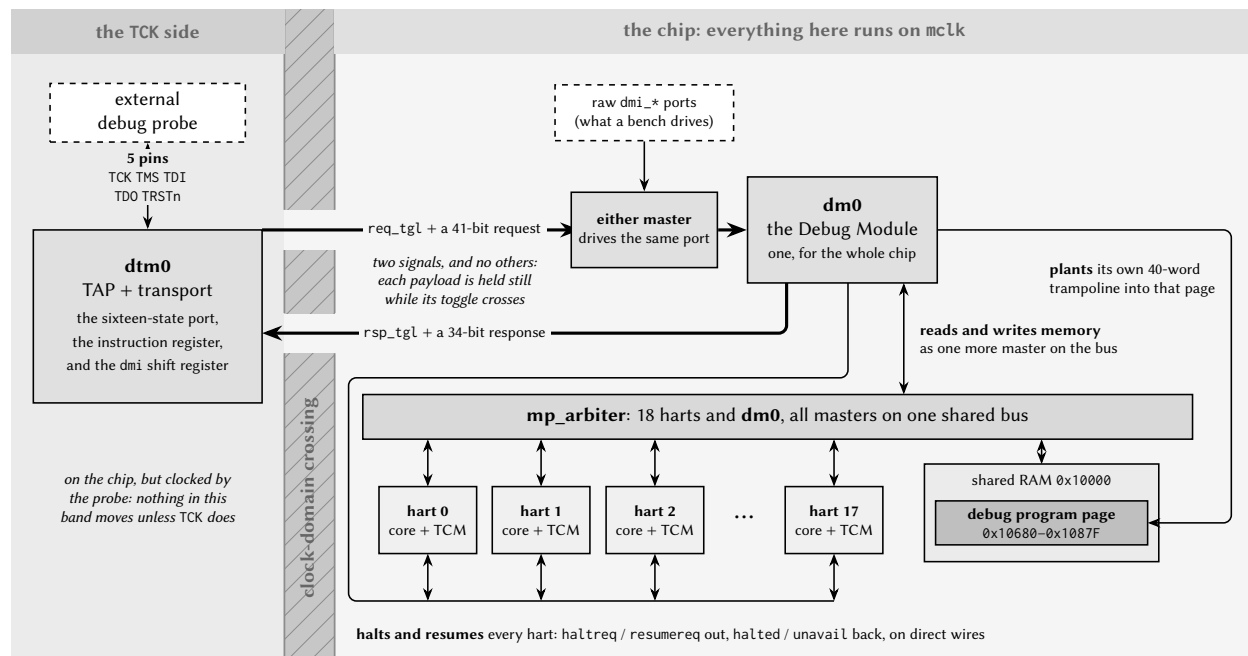
Figure 10: The debug path, from the probe to a hart, in a configuration built with debug support. The transport and the Debug Module sit in different clock domains , and the wall between them is crossed by exactly two signals: one toggle each way, each carrying a payload that is held still while its toggle is in flight. Everything to the right of that wall is ordinary chip fabric, and the one Debug Module reaches it in three ways: it halts and resumes the harts over direct wires, it reads and writes memory as one more master on the same arbiter the harts use, and it plants its own trampoline into the debug program page. The count of hart tiles follows this configuration.
