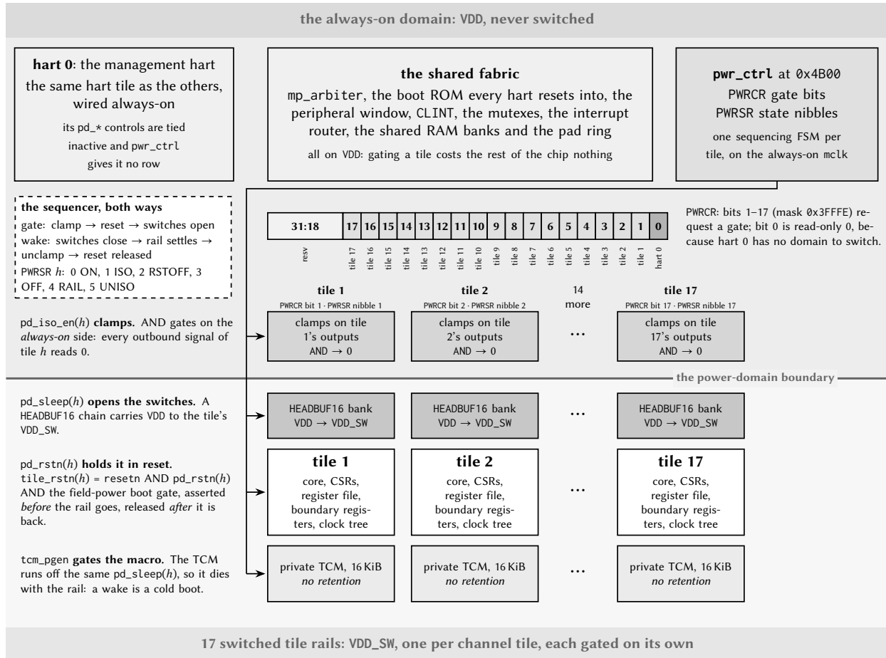
Figure 23: The chip's power domains. Everything the rest of the chip needs (the arbiter, the boot ROM, the peripherals, the shared RAM, the pad ring and hart 0) sits on the unswitched VDD rail; each channel tile has a rail of its own. Setting PWRCR bit h walks the four layers of tile h downwards: the clamps assert on the always-on side of the boundary, the tile is held in reset, and only then do the header switches open. Clearing the bit walks them back up, and because nothing in the tile retains state, what comes back up is a cold boot.
