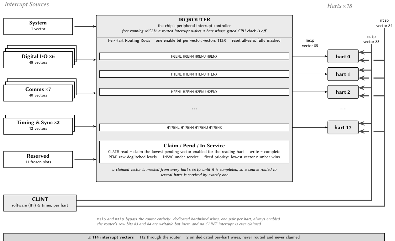
Figure 11: Argus interrupt fabric. Every one of this configuration's 114 interrupt vectors is on this page: the left column collapses Table 8's source population into types, each with the number of blocks that feed it and the number of vectors it owns, and the reserved slots are counted with the rest because the vector numbering is frozen — a dropped or not-yet-built block keeps its slot rather than shifting the ones above it. All of those terminate in the IRQROUTER, which holds one routing row per hart — one enable bit per vector, all zero out of reset — and one claim/complete stage; each row is drawn at the height of the hart it belongs to, so a row's meip wire runs straight across into that hart. The two heavy rails are the point of the figure: the CLINT's msip and mtip are per-hart hardwired levels that run under the router, up the far margin, and into each hart from the opposite side. They are never enabled, never pending, never claimed and never completed; the router's row bits at those two vector numbers are writable but inert, and its CLAIM never returns them. A hart's interrupt service routine clears an msip by writing its MSIP register and an mtip by advancing its MTIMECMP, not by completing a claim (Section 20). Both blocks run on the free-running MCLK, which is what lets an interrupt wake a hart whose gated CPU clock is off. The register layout behind all of it is Section 23's; no address appears here. Everything drawn is generated from this configuration.
