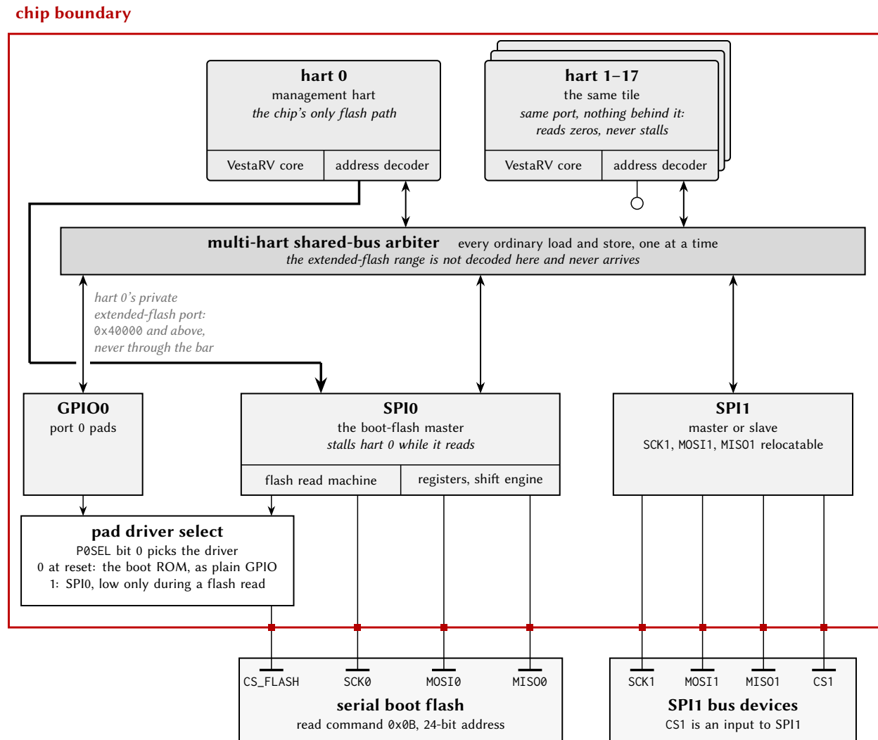
Figure 12: SPI connection diagram: SPI0 and the boot flash. Everything drawn is generated from this configuration. SPI0's registers are an ordinary arbiter slave, so every hart reaches them the same way, through the bar. The flash is different: hart 0's own address decoder claims every address at or above 0x40000 — the strict complement of the shared window — and takes it out of the tile on a private port that never reaches the bar and is never arbitrated, which is what makes execute-in-place possible (Section 14.10). SPI0 turns each such access into a flash read, sending the command byte and then (\text{CPU address} + \text{SPI0FOS}) \bmod 2^{24} , and stalls hart 0 until the word comes back. Every other hart has the same decoder and the same port with nothing behind it, so its accesses in that range read zeros and do not stall. CS_FLASH has two drivers and the pad's PxSEL bit chooses between them: it resets to 0, a plain GPIO output driven high, which is how the boot ROM clocks the flash before any of this is set up. SPI1, in configurations that include it, is a separate block with its own pins and no flash path of any kind.
