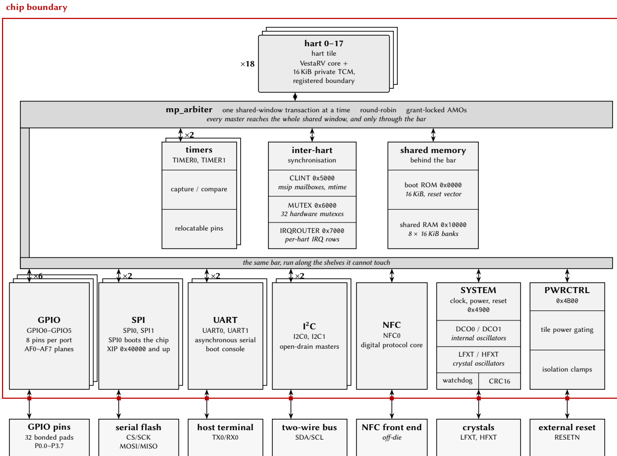
Figure 1: Argus whole-chip diagram: the bus and the peripherals. One serializing shared-window bus reaches everything on the die, so the mp_arbiter is drawn as the grey bar every block taps — run down the margin and along the lower shelves, because one bar cannot touch three shelves without a tap crossing a box. Masters on top; the pin-facing shelf against the red package boundary, its outside world beyond it; an \times N badge is N instances of one peripheral, not one block. Everything drawn is generated from this configuration.
