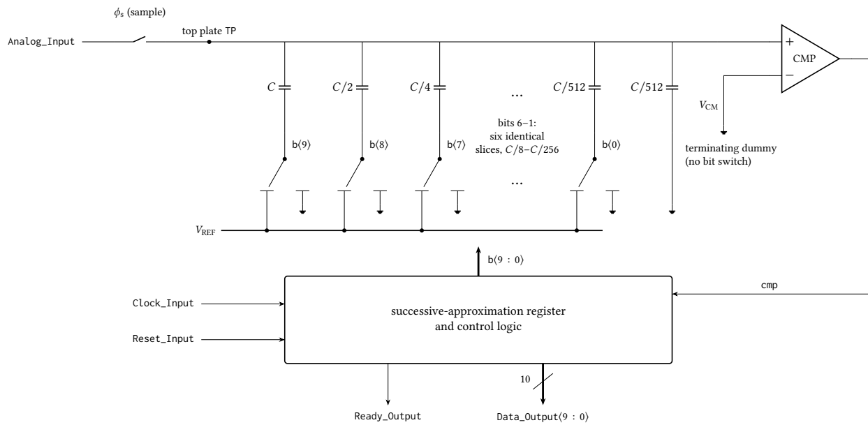
Figure 54: Generic single-ended charge-redistribution SAR ADC, drawn to explain the architecture of the 10-bit converter rather than to reproduce its implemented transistor-level schematic. The input is sampled through \phi_s onto the top plate of a binary-weighted array; the logic then switches each bottom plate from V_{REF} to ground one bit at a time, most significant first, and keeps or discards the trial from the comparator decision, so the conversion takes ten comparator cycles and the top plate converges to V_{CM} . Bits 6–1 are elided: six further slices identical to those drawn sit between C/4 and C/512 , and the terminating dummy C/512 carries no bit switch, which makes the total array 2C and the LSB weight C/512 . Only the external port names are those of the implemented block; the sampling network, comparator topology, clock generation and reset behaviour are representative, and no device dimensions are stated.
