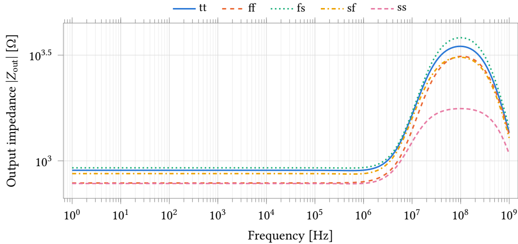
Figure 73: Magnitude of the supply block's output impedance against frequency over five process corners, 27 °C at point 1 and 25 °C at points 2–5. The AC load source carries unit magnitude, so |V_{DDDAC}| is the impedance in ohms. It is flat at 781 Ω to 927 Ω from 1 Hz to 100 kHz and peaks at 1.8 kΩ to 3.8 kΩ near 100 MHz. This is the small-signal impedance at zero load; the large-signal chord over the 0 μA to 100 μA sweep is 18 % to 51 % higher (Table 73).
