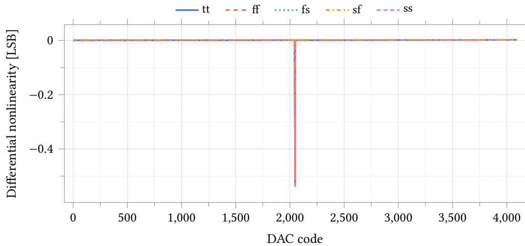
Figure 66: Ratiometric differential nonlinearity against code over five process corners: each code's output is divided by the reference measured at that code before the LSB and the first difference are taken, so the reference droop divides out and the ladder alone is measured. Conditions as Figure 65; the 4095-point curve is stride-decimated for the plot as in Figure 62. The major-carry hierarchy is the ideal-rail one — -0.53 at code 2048, then -0.28 at 1024, -0.24 at 3072, -0.14 at 512 and -0.13 LSB at 2560 — and the worst step matches Figure 62 to within 0.03 LSB. Raw DNL on the same bench is -9.8 to -18.4 LSB (Table 68); the difference is the reference step between adjacent codes and nothing else.
