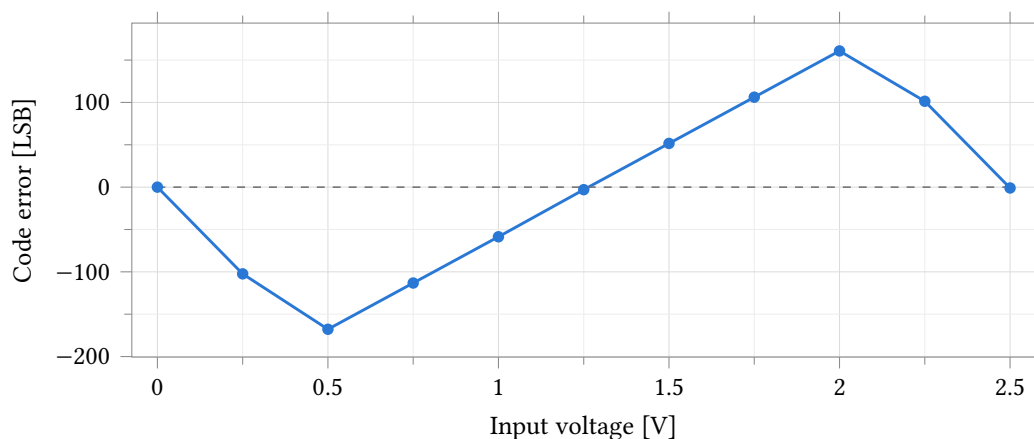
Figure 57: Code error against input voltage — measured code minus the ideal 409.6 codes/V line — from the same run as Figure 56. The error is the 1.535 slope ratio, not nonlinearity: it reaches -167.8 LSB at 0.5 V and 160.8 LSB at 2.0 V, crossing zero near the 1.25 V common mode where the measured and ideal lines intersect. It also returns near zero at 0 V and 2.5 V, where the clipped output coincides with the ideal endpoints; those two points are not accuracy. Referred to the fitted line instead, the residual over 0.5 V to 2.0 V is at most 0.52 LSB.
