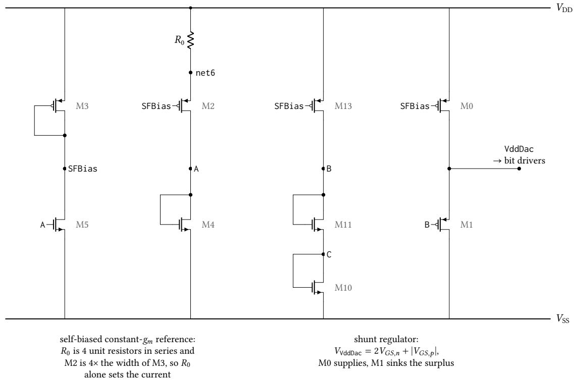
Figure 63: Core of anatop_pixel_dac_psu , the shunt regulator that generates the V_{ddDac} rail the ladder uses as its reference, transcribed from the LoadRegTB netlist. The self-biased constant- g_m reference on the left sets SFBias ; M13 drives that current through the stacked diodes M11 and M10 to hold B two gate-source voltages above V_{SS} , and M1 sinks whatever of M0 's current the ladder leaves, clamping V_{ddDac} one PMOS gate-source voltage above B : 2.177 V unloaded from a 2.5 V rail. There is no error amplifier, so load regulation is set by M1 's g_m alone. The five start-up and enable devices — the weak pull-up and its two kick devices on SU , the shutdown pull-up on SFBias and the En inverter — are omitted; none carries current once the loop is running. Device dimensions are proprietary and are not stated.
