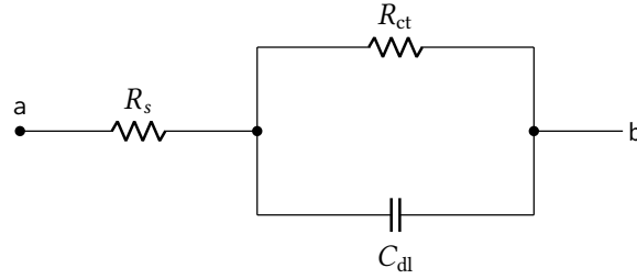
Figure 20: Single electrode–electrolyte interface, randles_electrode : a series solution resistance R_s ahead of the same charge-transfer and double-layer pair as Figure 19, presented as a two-terminal element. Values are given in Table 12; they describe a much smaller double layer and a much larger charge-transfer resistance than the three-electrode cell. None of the benches reported in this chapter uses it.
