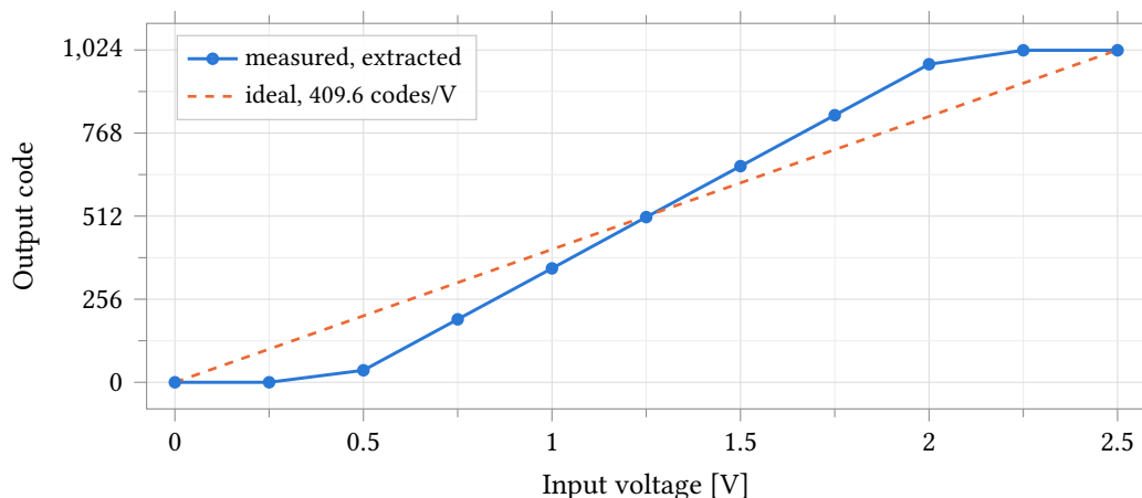
Figure 56: Output code against input voltage for the extracted anatop_pixel_adc , nominal corner, 37 °C, 2.5 V analog and 1.0 V digital supplies, with the ideal 409.6 codes/V line overlaid. The transfer is monotonic and reaches both code limits, but its slope is 628.64 codes/V – 1.535 times ideal – so the flat segments below 0.44 V and above 2.07 V are the code limits, not the ends of the sweep. Markers are the eleven simulated points; the 0.25 V step is 157 codes, so the curve between them is interpolation and carries no linearity information.
