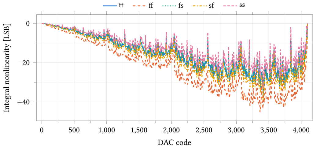
Figure 65: Integral nonlinearity against code over five process corners with the ladder referenced to V_{ddDac} from the supply block, zero external load, 25 °C. Endpoint-line INL as in Figure 61; the vertical scale is tens of LSB, not tenths. The bow reaches -37.1 LSB at tt (code 3413) and -45.1 LSB at ff (code 3365) and tracks the reference droop of Figure 64 scaled by code. Dividing each code's output by the reference measured at that code removes it and leaves 0.43 to 0.45 LSB (Table 68), so the ladder is unchanged from the ideal-rail case.
