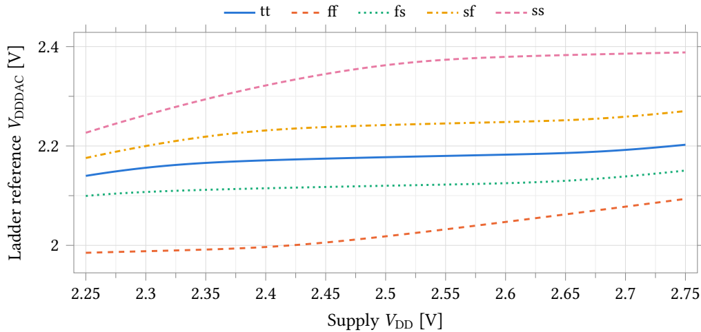
Figure 72: V_{DDDAC} against the supply, swept 2.25 V to 2.75 V, over five process corners at zero external load, 27 °C at point 1 and 25 °C at points 2–5. The slope is the line regulation tabulated in Table 75; it is not constant across the sweep, so the tabulated value is the chord between the two endpoints. The corner spread of the reference itself, 344 mV at nominal supply, is larger than anything the supply sweep produces.
