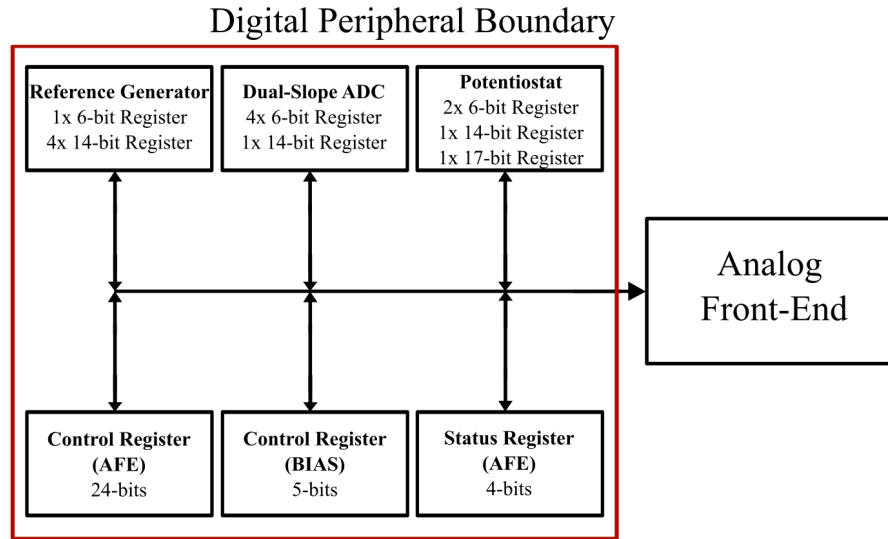
Figure 18: AFE digital peripheral block. Inside the peripheral boundary the memory-mapped register file splits into the reference-generator, DSADC and potentiostat trim groups (top) and the AFE_CR, BIAS_CR and AFE_SR registers (bottom); every group drives the analog front end over the same control bus. Widths are the implemented register widths, not the memory-map word size.
