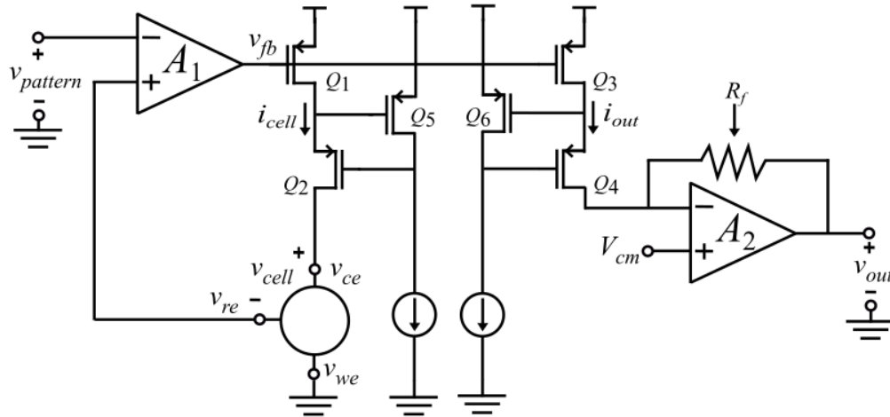
Figure 15: Potentiostat front-end schematic. A_1 (folded-cascode) is the control amplifier; Q_1 – Q_6 form the regulated cascode current mirror with unity gain; A_2 with R_f implements the transimpedance amplifier. The excitation voltage v_{\text{pattern}} is generated by the BIAS_REV_POT DAC.
