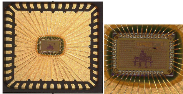
Figure 2: Myshkin MCU Bonding Image (1.5 mm × 1.0 mm)
