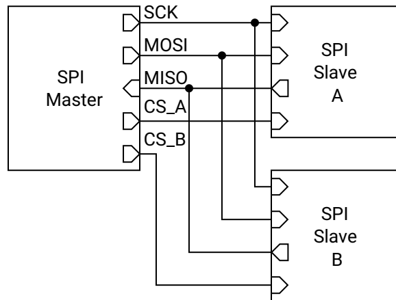
Figure 4: SPI Connection Diagram
