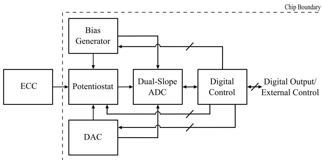
Figure 14: AFE system block diagram. The potentiostat front end (left) conditions the electrode current; the dual-slope ADC (centre) digitises the result; the digital peripheral (right) exposes both subsystems through memory-mapped registers.
