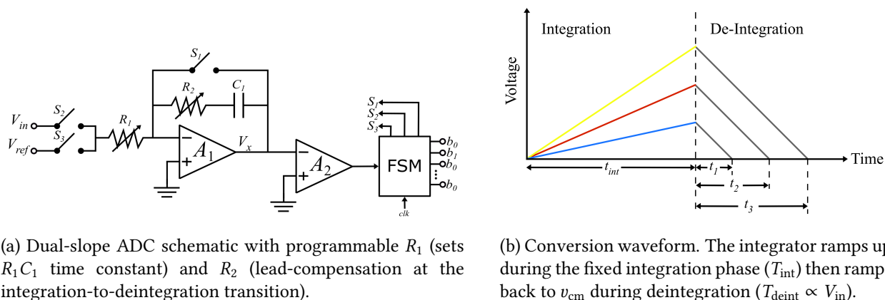
Figure 16: Dual-slope ADC circuit and conversion waveform.
