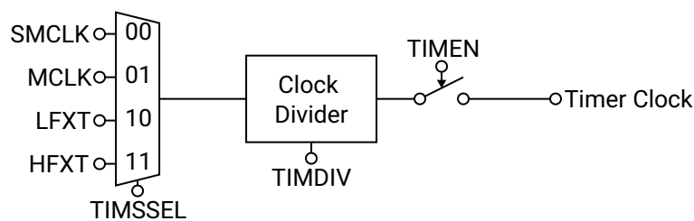
Figure 10: TIMERx Clock Diagram
