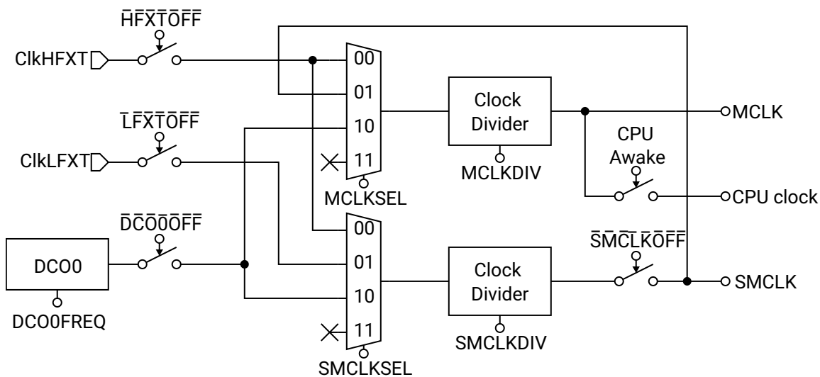
Figure 13: MCU Clock System
