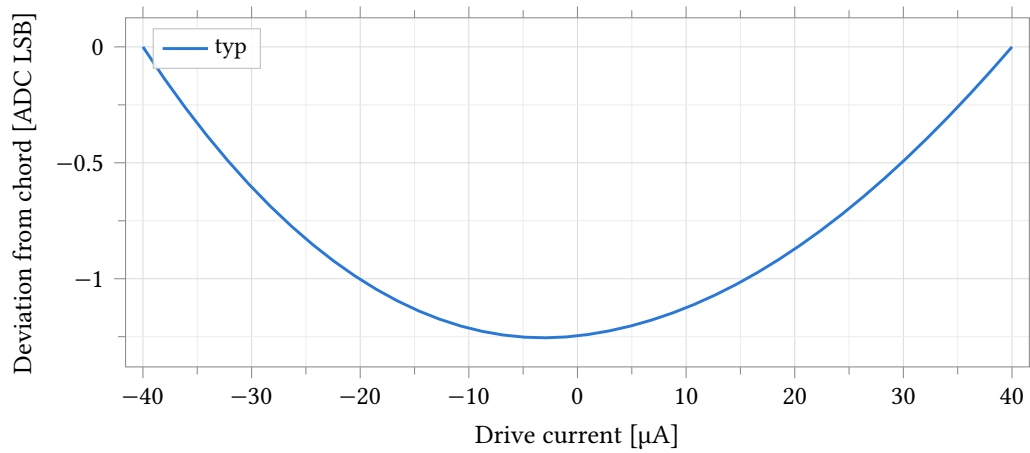
Figure 70: Drive nonlinearity of the bottom code ( N = 0 , R \approx 19.6 \text{ k}\Omega ): voltage deviation from the endpoint chord over \pm 90\% of full scale ( \pm 40 \mu\text{A} ), typical corner, expressed in 1.592 \text{ mV ADC LSB} . All ten bypass gates are closed at this code and carry the full signal current; their on-resistance rises with the terminal's excursion from V_{\text{CM}} , so the chord — pinned at the sweep endpoints where that excursion is largest — overestimates the mid-range voltage by up to 1.25 \text{ LSB} , and the deviation is bowl-shaped with a slight skew from the gates' voltage asymmetry. The same measurement at N = 63 and N = 319 , where the ladder dominates and current is 20\text{--}100\times smaller, stays below 0.004 \text{ LSB} and is tabulated, not plotted.
