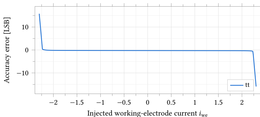
Figure 51: Accuracy error at the operational max-gain point, R_f = 560 \text{ k}\Omega into R_{ct} = 1 \text{ M}\Omega , typical process point, 37^\circ\text{C} . The truth current sweep is \pm 2.3 \text{ }\mu\text{A} , just beyond the 2.06 \text{ }\mu\text{A} full-scale current at this gain tap; the crossing at zero is smooth, with no kink, over the full swept range shown.
