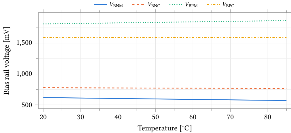
Figure 27: The four local bias rails against temperature at the typical corner. V_{BNM} and V_{BNC} are referred to vss! ; V_{BPM} and V_{BPC} sit near the supply.
