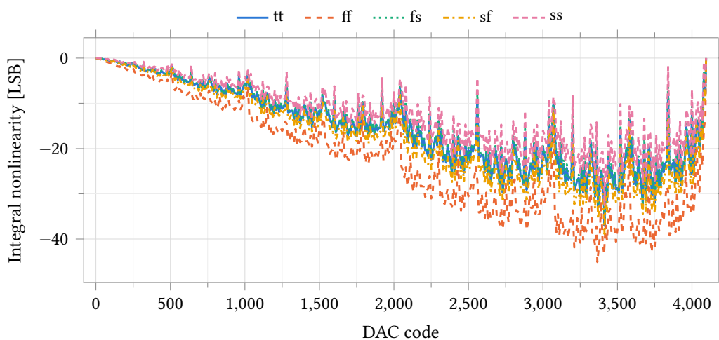
Figure 76: Integral nonlinearity against code over five process corners with the ladder referenced to VddDac from the supply block, zero external load, 25 °C. Endpoint-line INL as in Figure 72; the vertical scale is tens of LSB, not tenths. The bow reaches -37.1 LSB at tt (code 3413) and -45.1 LSB at ff (code 3365) and tracks the reference droop of Figure 75 scaled by code. Dividing each code's output by the reference measured at that code removes it and leaves 0.43 to 0.45 LSB (Table 77), so the ladder is unchanged from the ideal-rail case.
