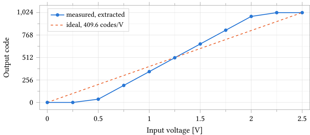
Figure 62: Output code against input voltage for the extracted anatop_pixel_adc , nominal corner, 37 °C, 2.5 V analog and 1.0 V digital supplies, with the ideal 409.6 codes/V line overlaid. The transfer is monotonic and reaches both code limits, but its slope is 628.64 codes/V — 1.535 times ideal — so the flat segments below 0.44 V and above 2.07 V are the code limits, not the ends of the sweep. Markers are the eleven simulated points; the 0.25 V step is 157 codes, so the curve between them is interpolation and carries no linearity information.
