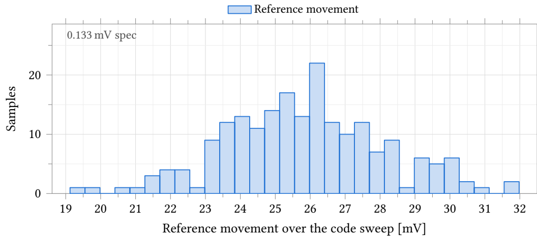
Figure 80: Peak-to-peak movement of the DAC reference VddDac across the 4096-code sweep, with the ladder referenced to the on-chip supply block instead of an ideal rail. Process and mismatch , castalia_pm_25, 200 samples, 25 °C, no external load on VddDac. The quarter-LSB budget of 133 \mu V entered on the test sits about 200 times below the data, so it is annotated at the left axis edge rather than drawn and the distribution is not compressed into a single bar; the closest sample misses it by a factor of 144. Meeting it needs the supply’s output impedance down by a factor of 193, to about 5 \Omega , against 894 \Omega small-signal (Table 87) and 1133 \Omega as a 0 \mu A to 100 \mu A chord (Table 83).
