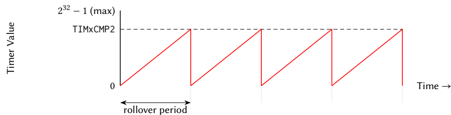
Figure 13: Timer Rollover Operation
