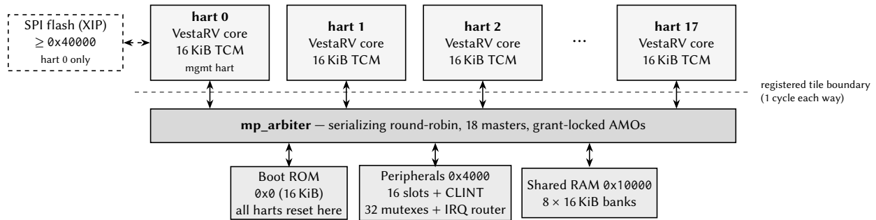
Figure 1: Argus top-level block diagram (generated from this configuration: 18 harts, 128 KiB shared RAM). Every hart tile couples an unmodified VestaRV core with its private TCM; everything else is reached through the serializing round-robin arbiter.
