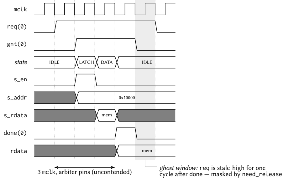
Figure 3: One uncontended shared-window read, at the mp_arbiter pins. The arbiter walks IDLE → LATCH → DATA : the transaction is presented to the slave for one cycle, the synchronous slave returns data the following cycle, and done and rdata are registered together at the edge leaving DATA — three mclk from an observed req . The hart itself sees about two cycles more, one in each direction across the registered tile boundary. In the shaded cycle the master's req is still high although its transaction is over; the arbiter masks that stale request until it is observed low, which is what stops a completed access from being served twice.
