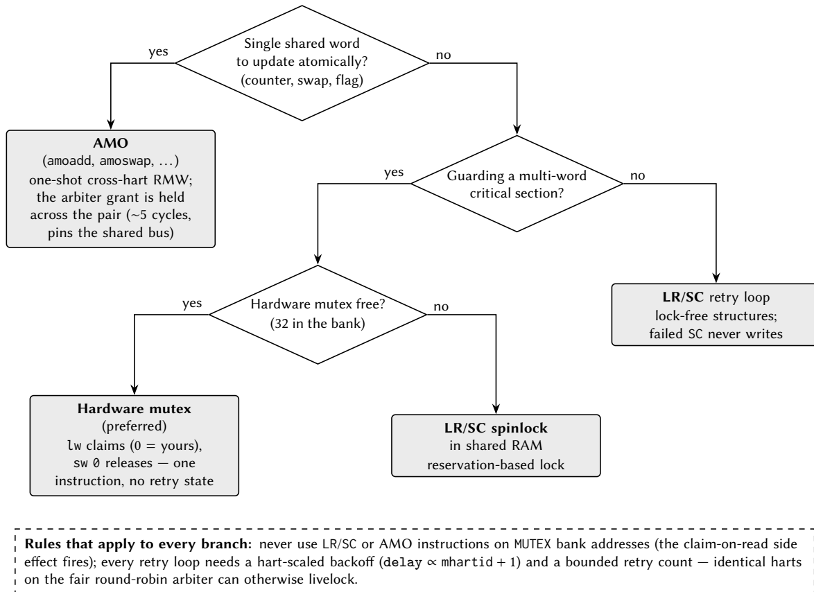
Figure 5: Choosing a synchronization primitive. The dashed box lists the two rules that apply to every branch.
