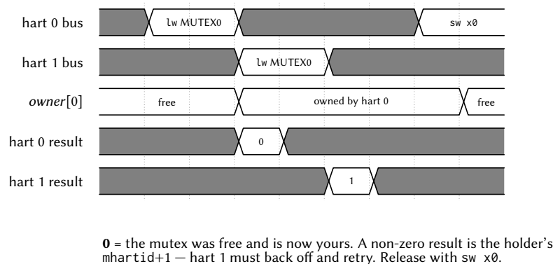
Figure 18: Two harts racing for the same mutex. The arbiter serializes the two claim reads, so the return-old-and-claim happens atomically with no retry loop: hart 0 reads 0 and thereby owns the mutex, and hart 1 reads hart 0's marker and must back off.
