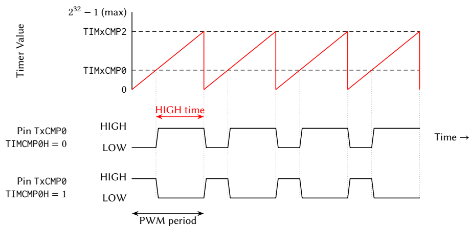
Figure 14: Timer Output Compare and PWM Operation
