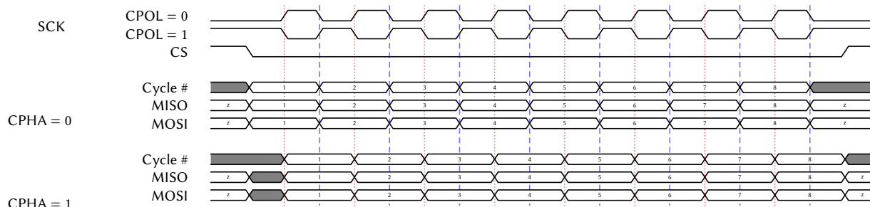
Figure 7: SPI Timing Diagram
