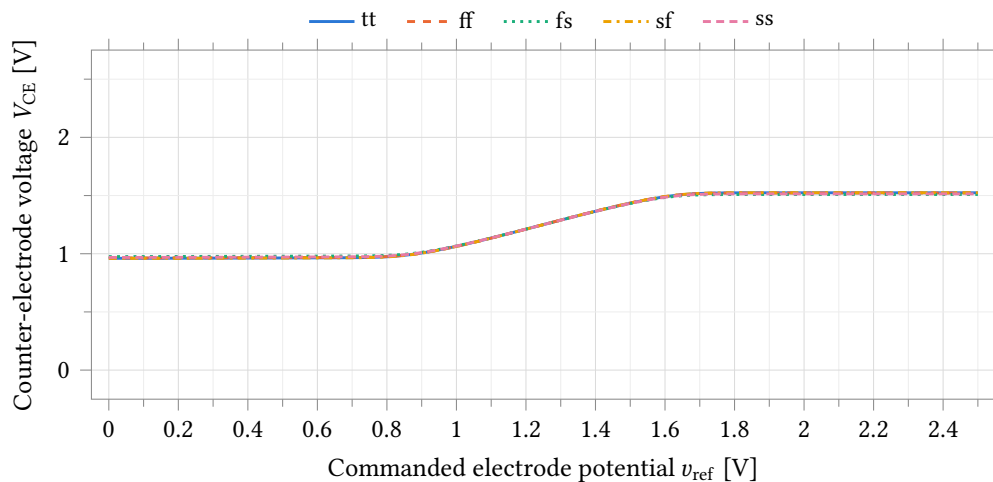
Figure 21: Counter-electrode voltage over the same sweep, against the full supply range. V_{\text{CE}} stops about 1 V short of each rail because the amplifier reaches its current limit before its voltage limit, so the drive shortfall in Table 15 is a current-budget problem rather than a compliance one.
