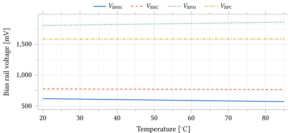
Figure 10: The four local bias rails against temperature at the typical corner. V_{\text{BNM}} and V_{\text{BNC}} are referred to vss!; V_{\text{BPM}} and V_{\text{BPC}} sit near the supply.
