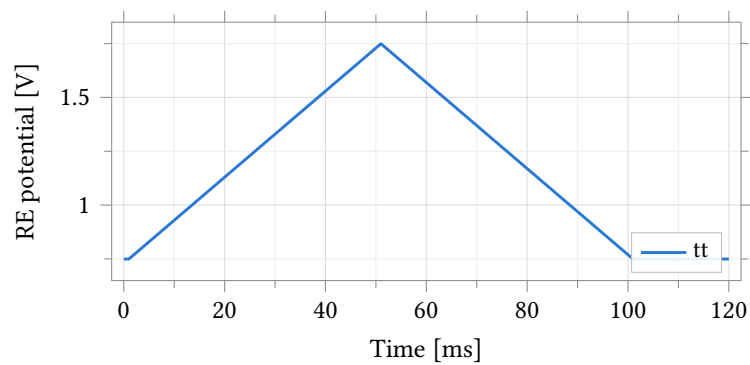
Figure 33.36: Commanded reference-electrode potential against time for the triangular voltammetry sweep, typical process point, 37 °C, R_f = 35 \text{ k}\Omega , R_{ct} = 1 \text{ M}\Omega electrode. Paired with the current response of Figure 33.35.
