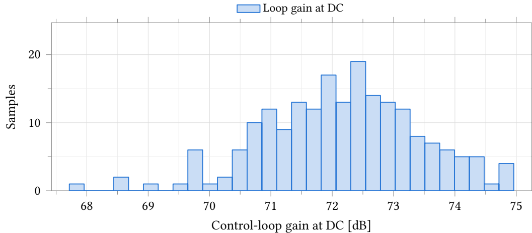
Figure 24.30: DC gain of the control loop closed around an electrochemical cell. Process and mismatch , 37 °C, 200 samples, cell-drive bench (Figure 24.28) with a Randles cell of R_{CE} = 1\text{ k}\Omega , R_u = 1\text{ k}\Omega , R_{ct} = 10\text{ k}\Omega , C_{dl} = 1\text{ }\mu\text{F} , working electrode at 1.25 V, C_L = 5\text{ pF} , C_c = 500\text{ fF} , 2.5 V supply. The loop is measured through the reference-electrode sense wire and therefore includes the cell, whose 12 k \Omega loads an open-loop output resistance of about 25 k \Omega and is 10 dB below the unity-feedback gain of Table 24.20. The spread is 7 dB peak to peak and no sample falls below 67 dB. No limit was entered on this output.
