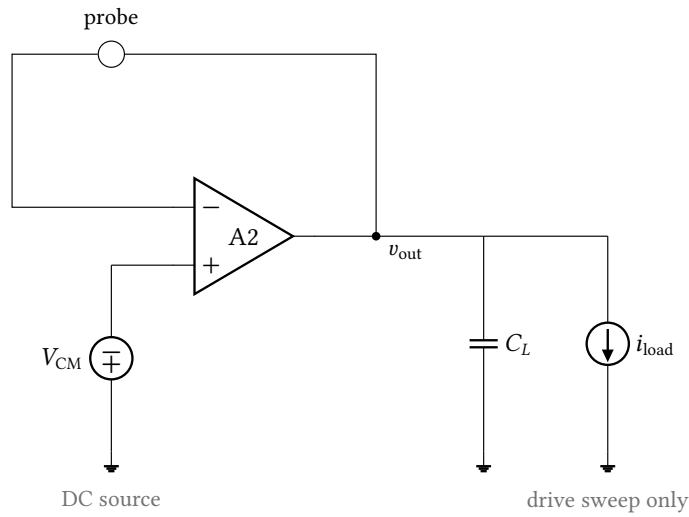
Figure 27: Unity-feedback bench. The amplifier’s output is returned to its inverting input through a current probe and loaded by C_L = 5 pF; the loop-gain analysis through that probe gives the amplifier’s own gain and margins, and DC and noise analyses on the same wiring give the offset and output noise. The drive measurement adds the swept load current i_{load} on the same schematic. Supplies, the bias rails and the enable pin are omitted here and in Figure 30.
