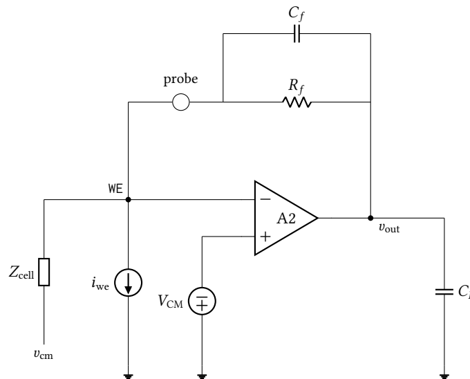
Figure 30: The closed transimpedance loop bench, the only one in this section that closes feedback around the electrode. R_f \parallel C_f returns the output to the working electrode through a current probe, i_{we} is the test source, and Z_{cell} is the Randles cell of Figure 13, returned to v_{cm} . The loop gain, phase margin and crossover are measured through the probe; the DC accuracy, closed-loop transfer and noise figures come from the same wiring.
