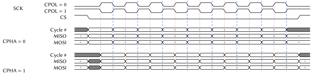
Figure 18: SPI Timing Diagram
