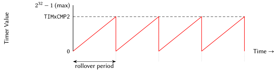
Figure 24: Timer Rollover Operation
