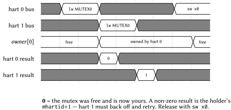
Figure 29: Two harts racing for the same mutex. The arbiter serializes the two claim reads, so the return-old-and-claim happens atomically with no retry loop: hart 0 reads 0 and thereby owns the mutex, and hart 1 reads hart 0's marker and must back off.
