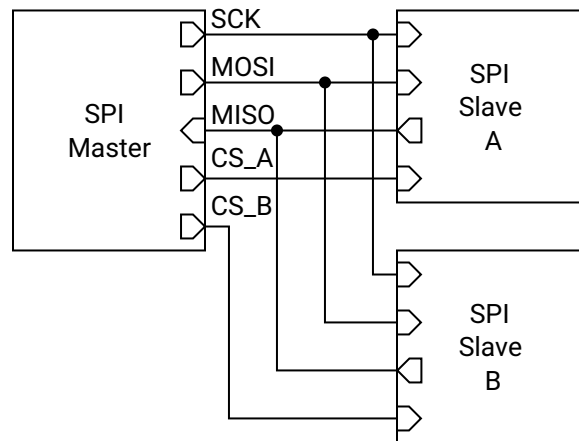
Figure 17: SPI Connection Diagram
