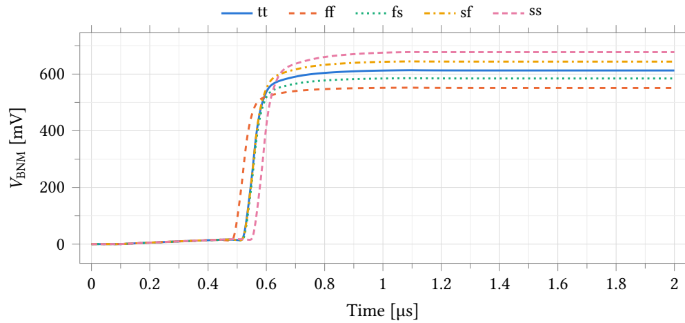
Figure 16: Power-up settling of V_{\text{BNM}} over all process corners.
