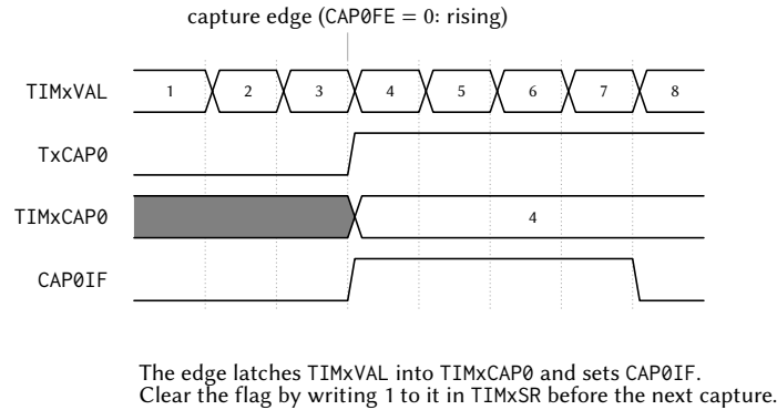
Figure 26: Input capture. The selected edge on TxCAP0 latches the live TIMxVAL into TIMxCAP0 and sets CAP0IF; the flag must be cleared by writing 1 to it in TIMxSR before the next capture event.
