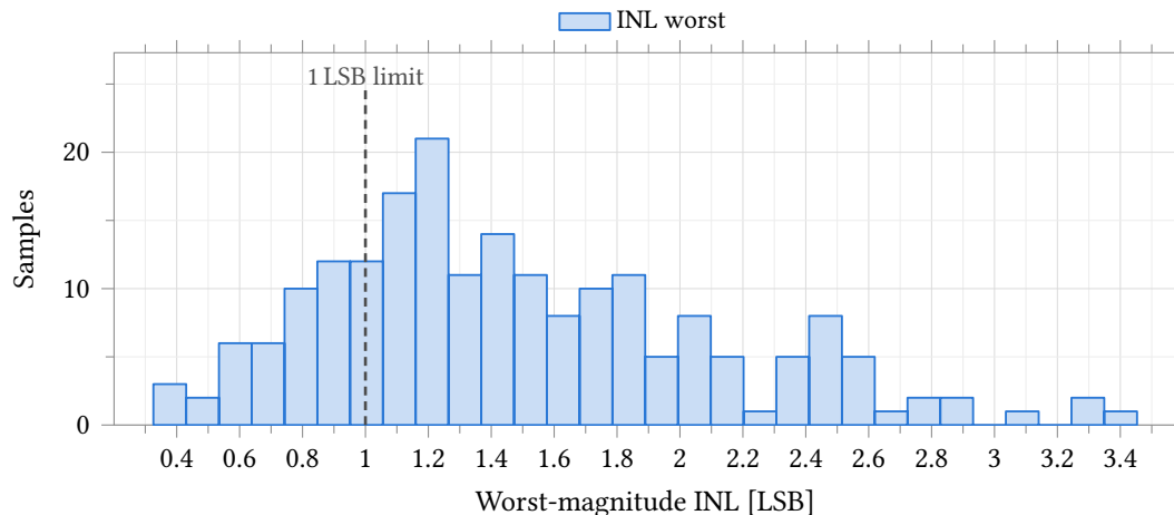
Figure 67: Integral nonlinearity of the R - 2R ladder driven from an ideal 2.5 V reference. Process and mismatch , model section castalia_pm_25 , 200 samples, seed 12345, low-discrepancy sampling, 25 °C, all 4096 codes. The dashed rule is the 1 LSB limit entered on the test; 42 of 200 samples fall inside it and the worst reaches 3.453 LSB. The distribution is right-skewed (Fisher skew +0.74), so Table 69 quotes the median and percentiles rather than \text{mean} \pm 3\sigma . LSB size, full scale and gain error are fixed to a part in 10^6 on this bench (Table 70), so the whole of this spread is resistor mismatch in the ladder and none of it is the reference.
