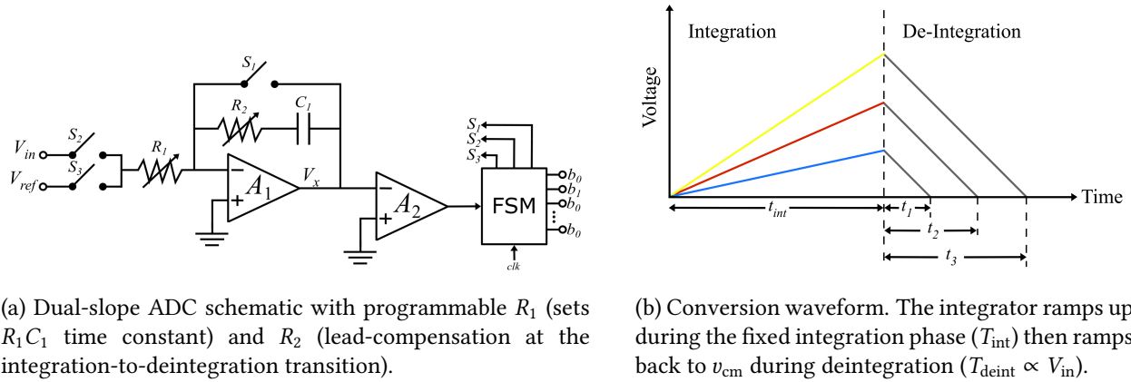
Figure 14: Dual-slope ADC circuit and conversion waveform.
