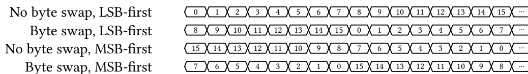
Figure 5: SPI Bit Ordering (16-bit transfer)
