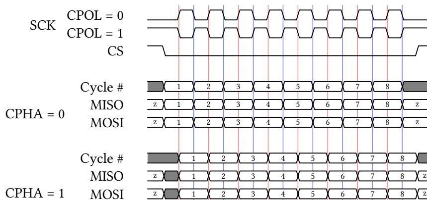
Figure 3: SPI Timing Diagram
