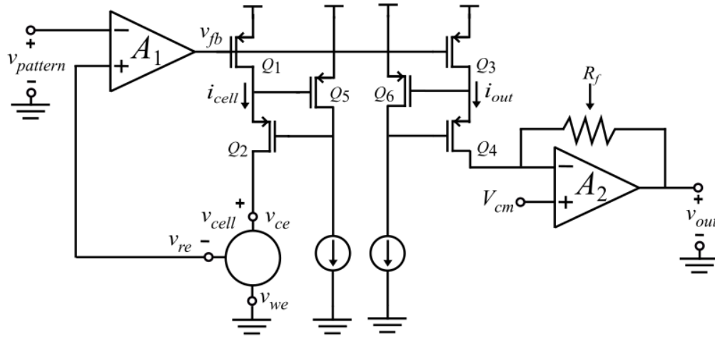
Figure 13: Potentiostat front-end schematic. A_1 (folded-cascode) is the control amplifier; Q_1 – Q_6 form the regulated cascode current mirror with unity gain; A_2 with R_f implements the transimpedance amplifier. The excitation voltage v_{\text{pattern}} is generated by the BIAS_REV_POT DAC.
