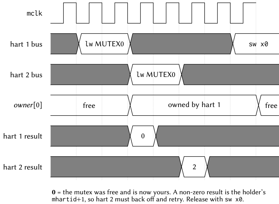
Figure 64: Two harts racing for the same mutex. The arbiter serializes the two claim reads, so the return-old-and-claim happens atomically with no retry loop: the hart the arbiter serves first reads 0 and thereby owns the mutex, and the other reads the winner's marker (mhartid + 1) and must back off.
