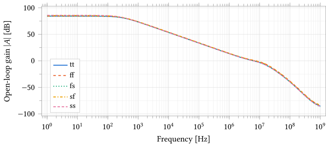
Figure 38: Open-loop gain over the five process corners, by stb through the feedback probe with the amplifier in unity feedback and a 5 pF load. Miller compensation gives a single-pole roll-off from 290 Hz to a 6.2 MHz to 7.6 MHz crossover. This is the amplifier alone. The loop that closes around the electrode is characterised in Figure 43 and Table 35; with the cell model and C_f = 22 \text{ pF} it holds 61.2^\circ to 64.9^\circ of phase margin.
