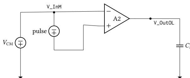
Figure 37: Open-loop slew testbench, SlewOpenLoopTB. The inverting input is held at V_{CM} and a floating pulse source drives the pair differentially rail to rail, into C_L = 5 pF. With no feedback the output is driven hard in both directions, so the slew rates of Table 33 are open-loop full-swing values and bound the closed-loop settling rate rather than equalling it.
