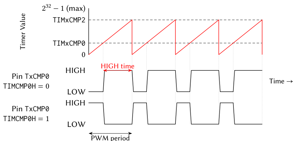
Figure 59: Timer Output Compare and PWM Operation
