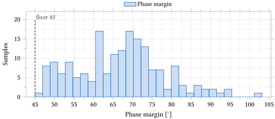
Figure 48: Transimpedance loop phase margin at maximum gain. Process and mismatch (castalia_pm_25), 37 °C, 200 samples, seed 12345, LDS sampling, N = 179 . Minimum 46.6° against a 45° criterion. Reported as percentiles and extreme sample; the distribution is right-skewed.
