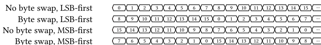
Figure 9: SPI Bit Ordering (16-bit transfer)
