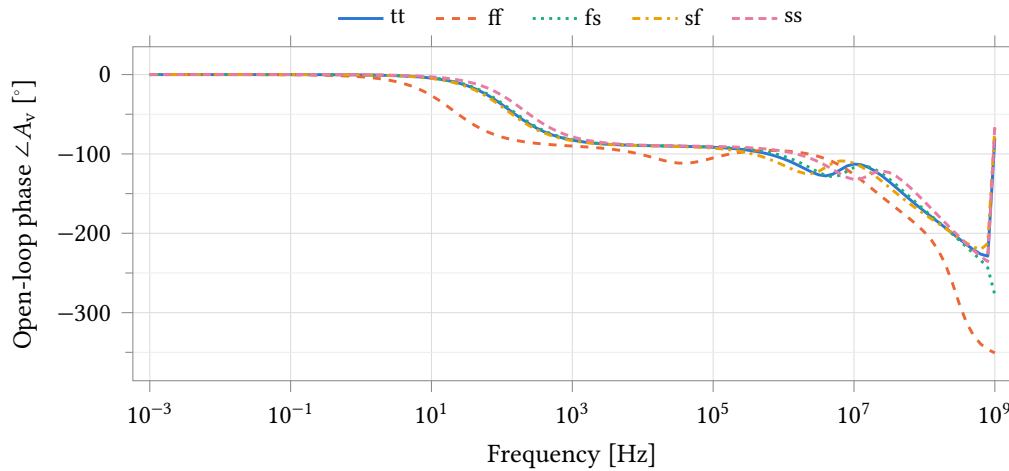
Figure 19: Open-loop phase against frequency, same conditions as Figure 18. The phase passes through -115.7^\circ at the unity-gain frequency, so the non-dominant poles have taken only about 26^\circ by the time the gain reaches unity. The step at the extreme right is an unwrapping artefact: at ten points per decade the phase moves by more than 180^\circ between the last two samples and the unwrapper cannot follow it. It is above 500 MHz, three decades past unity gain, and does not affect the margins in Table 16.
