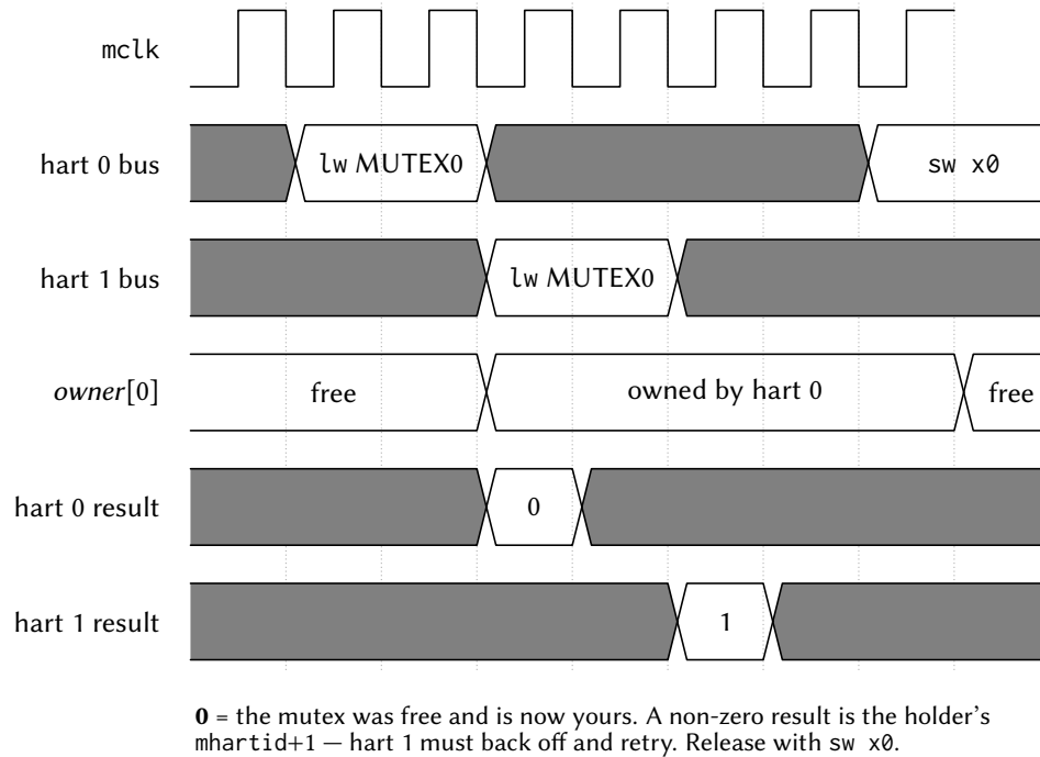
Figure 39: Two harts racing for the same mutex. The arbiter serializes the two claim reads, so the return-old-and-claim happens atomically with no retry loop: hart 0 reads 0 and thereby owns the mutex, and hart 1 reads hart 0's marker and must back off.
