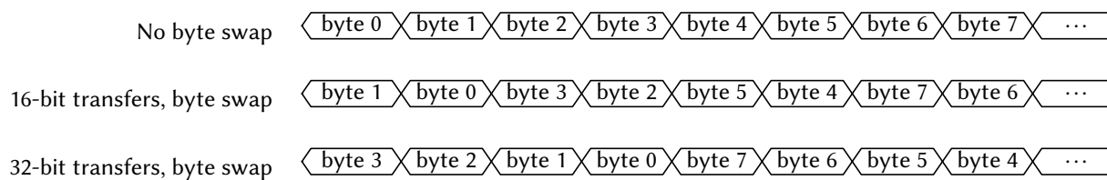
Figure 29: SPI Byte Ordering
