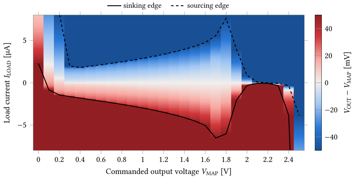
Figure 24: DC drive compliance of the control amplifier at the typical corner, as a map of the unity-gain tracking error over commanded output voltage and load current. Positive I_{\text{LOAD}} draws current out of the output, so the amplifier sources ; negative I_{\text{LOAD}} injects, so it sinks . The colour scale is clipped at \pm 50 mV, which is the compliance criterion: inside the envelope the error is the smooth I_{\text{LOAD}}R_{\text{OUT,CL}} gradient, and outside it the output has hit a rail and the error jumps by more than a volt, so everything beyond the envelope saturates to solid colour. The two black curves are the |V_{\text{OUT}} - V_{\text{MAP}}| = 50 mV edges, interpolated on the 50 nA sweep at each of the 26 commanded voltages; that they land on the boundary of the graded band is a check that the map and the envelope were derived independently. The vertical axis is cropped to \pm 8 \mu\text{A} . Figure 25 gives the same envelope over all five process corners.
