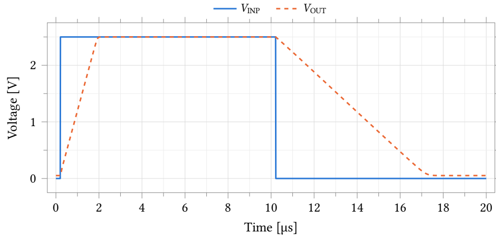
Figure 22: Large-signal step response. The open-loop bench slams the differential input from -1.25 V to +1.25 V and back, fully steering the input pair, so the output slews at the rate the output stage can charge and discharge the 10 pF load. The two edges are visibly unequal: the output takes 1.4 \mu\text{s} to slew up and 5.7 \mu\text{s} to slew back down, a factor of four.
