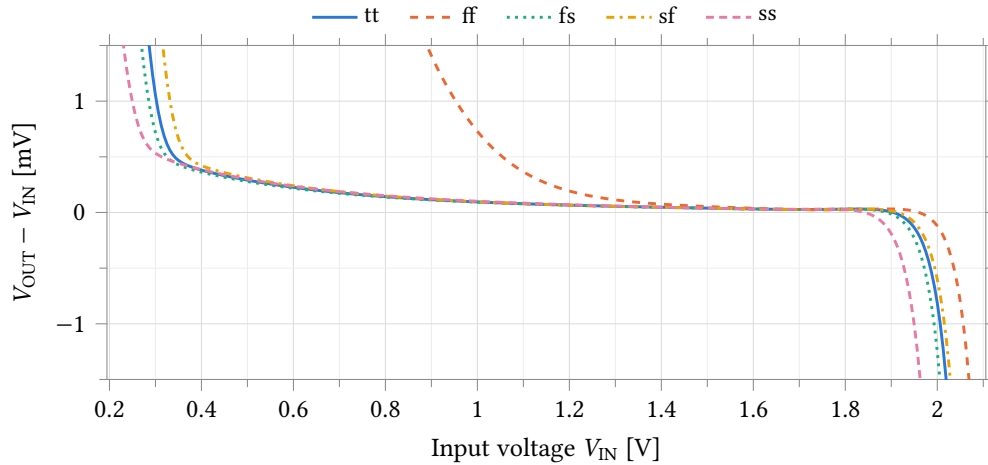
Figure 20: Unity-gain tracking error against input voltage. Inside the window 0.30 V to 2.01 V the error stays under 1 mV, passing through 61 \mu V at mid-supply; the curve leaves the frame at both ends, where the PMOS tail runs out of headroom near the supply and the output stage reaches its low limit near vss!. The vertical scale is clipped to \pm 1.5 mV so the in-range behaviour is visible at all — the error reaches 97 mV at 0 V and -382 mV at 2.5 V.
