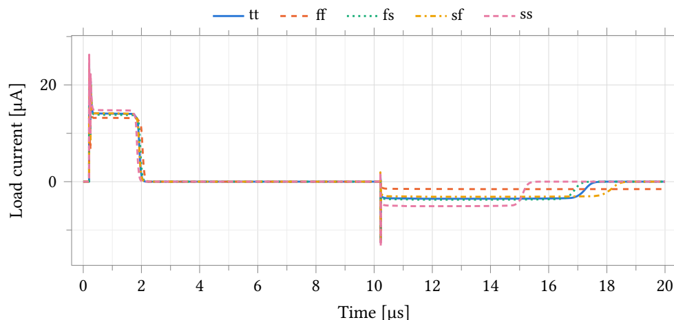
Figure 23: Current delivered into the 10 pF load during the same step, positive out of the amplifier. The asymmetry is plain: while the output slews up the cascoded PMOS mirror holds a flat 14.1 \mu\text{A} , and while it slews down the output pulls only 3.5 \mu\text{A} . The narrow spikes at each edge — 24.4 \mu\text{A} and 12.6 \mu\text{A} — last well under a microsecond; it is the flat sections that set the slew rate. These are slewing currents with the input pair overdriven past its common-mode range, so read them as the shape of the asymmetry rather than as a drive rating; see the discussion following Table 19.
