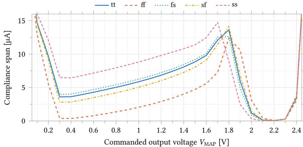
Figure 25: Width of the \pm 50 mV compliance envelope against commanded output voltage, over all five process corners. The shape is the same in every corner — pinched at both ends of the output range and widest around 1.8 V — so the deficit against the \pm 33 \mu A target is structural, not a corner artefact. The vertical scale is clipped at 16 \mu A : outside roughly 0.3 V to 1.9 V the buffer no longer tracks its input at zero load, and the apparent span there rises past 30 \mu A because it is measuring the current needed to force the output onto the commanded value, not compliance. Note also that the resistor and MIM rows are pinned at typical in all five corners (see the note below), so this is the transistor-corner spread only and understates the true one.
