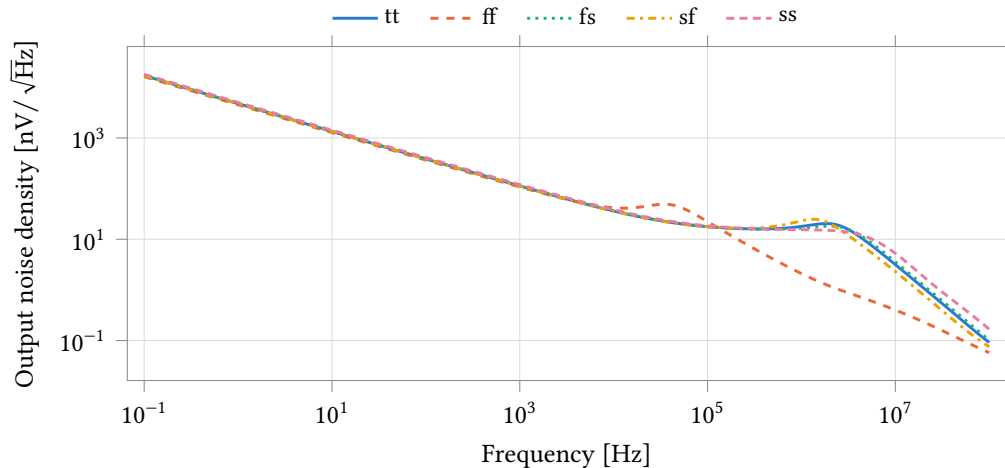
Figure 26: Output-referred noise density of the amplifier in unity-gain feedback, including the noise of the local bias generator. Flicker noise dominates below the 34 kHz corner and reaches 4.77 \mu\text{V}/\sqrt{\text{Hz}} at 1 Hz; the broadband floor is 16.0 \text{ nV}/\sqrt{\text{Hz}} , and the fall above about 2 MHz is the closed-loop bandwidth rolling the noise off, not a reduction in the noise generated.
