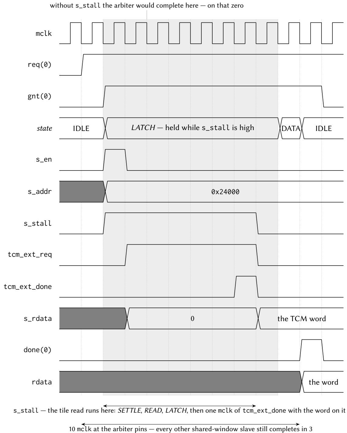
Figure 5: One stalled shared-window read: the management hart through a TCM aperture, at the same mp_arbiter pins as Figure 4. Up to the shaded region it is the ordinary walk — the grant, the one-cycle s_en strobe, the address presented. The aperture slave raises s_stall in that same cycle, and the arbiter stays in LATCH : grant pinned, address still presented, only the completion moves. Underneath, the tile's read port takes one SRAM read and returns the word on a single mclk of tcm_ext_done ; the slave captures it, drops s_stall , and the arbiter finishes the transaction it was holding. Without the stall it would have completed on the marked cycle, handing back the zero the slave had not filled in yet.
