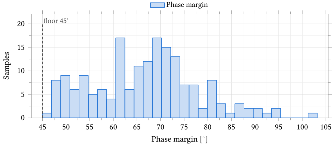
Figure 47: Transimpedance loop phase margin at maximum gain over 179 converged samples of 200 (process and mismatch), 37 °C. Every converged sample clears the 45° floor, the worst at 46.6°, which is what validates C_f = 22 pF — the corner run behind Table 33 gave 61.2° to 64.9° and carries no mismatch at all. The distribution is right-skewed, so p_1/p_{99} and worst case are quoted rather than mean \pm 3\sigma . 48 of 400 samples did not converge and are excluded (Section 7.4.4).
