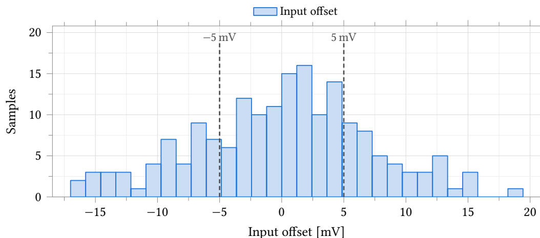
Figure 49: Input offset at maximum gain, 179 converged samples of 200 (process and mismatch). \sigma = 7.09 \text{ mV} against a \pm 5 \text{ mV} budget gives 54.7 % per-channel yield and, over four identical channels, roughly 9 % of chips with all four in budget. This is the block's binding limitation and it is a mismatch quantity, so no corner run bounds it. The control amplifier fails the same way (Section 7.3).
