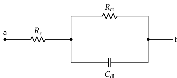
Figure 12: Single electrode–electrolyte interface, randles_electrode : a series solution resistance R_s ahead of the same charge-transfer and double-layer pair as Figure 11, presented as a two-terminal element. Values are given in Table 8; they describe a much smaller double layer and a much larger charge-transfer resistance than the three-electrode cell. None of the benches reported in this chapter uses it.
