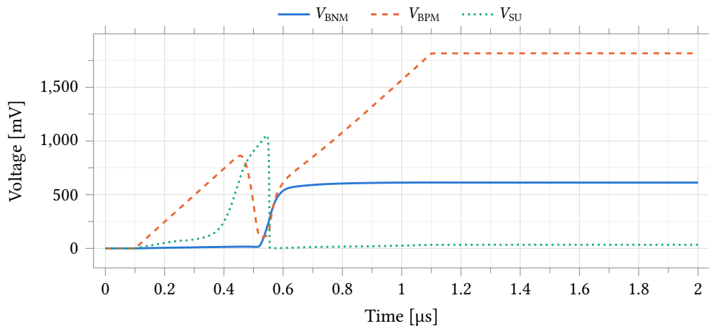
Figure 22: Power-up transient at the typical corner. The start-up node V_{SU} pulls the core out of its zero-current state, after which both mirror rails settle to their steady-state values.
