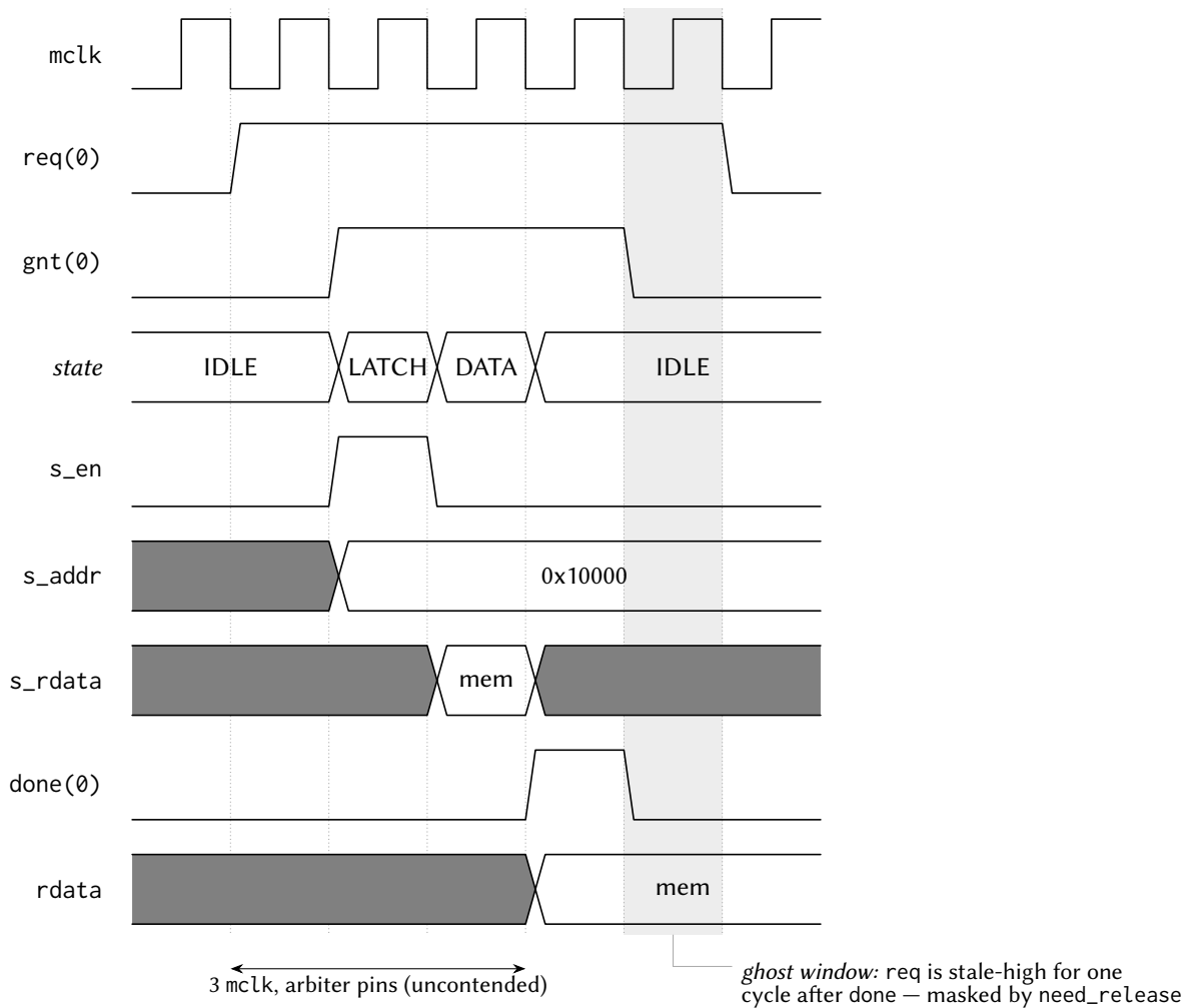
Figure 4: One uncontended shared-window read, at the mp_arbiter pins. The arbiter walks IDLE → LATCH → DATA : the transaction is presented to the slave for one cycle, the synchronous slave returns data the following cycle, and done and rdata are registered together at the edge leaving DATA — three mclk from an observed req . The hart itself sees about two cycles more, one in each direction across the registered tile boundary. In the shaded cycle the master's req is still high although its transaction is over; the arbiter masks that stale request until it is observed low, which is what stops a completed access from being served twice.
