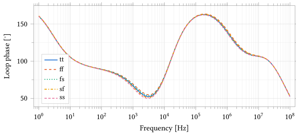
Figure 43: Loop phase for the same five runs. In this convention 0^\circ is the instability point, so the phase at crossover is the phase margin directly: 61.2^\circ to 64.9^\circ . Cadence's phaseMargin() returns exactly 180^\circ less on this result and is not used here or in Section 7.3.
