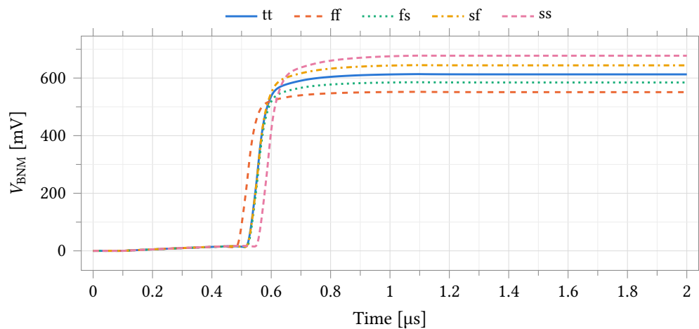
Figure 23: Power-up settling of V_{BNM} over all process corners.
