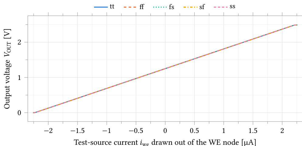
Figure 45: Output voltage against the swept test-source current over the five corners, at R_f = 560 kΩ with the electrode held at v_{cm} = 1.25 V. The bench source draws current out of the WE node, so i_{we} = -I_{WE} against Equation (1) and the slope is +R_f . The corners overlay to the line width because that slope is the feedback resistor, ideal in this bench.
