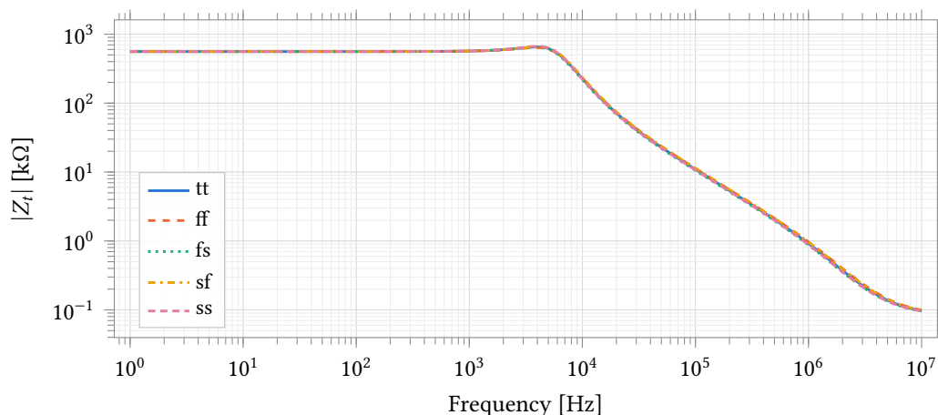
Figure 44: Closed-loop transimpedance magnitude, five corners, conditions as Figure 42. Peaking is 1.2 dB to 1.5 dB at 3.98 kHz and the -3 dB bandwidth 7.2 kHz to 7.5 kHz. Both are set by C_f ; at C_f = 5 pF the same cell peaks 3.0 dB to 3.7 dB with 41.7^\circ to 46.4^\circ of margin.
