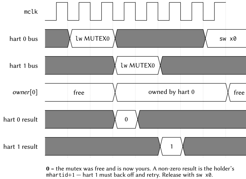
Figure 62: Two harts racing for the same mutex. The arbiter serializes the two claim reads, so the return-old-and-claim happens atomically with no retry loop: hart 0 reads 0 and thereby owns the mutex, and hart 1 reads hart 0's marker and must back off.
