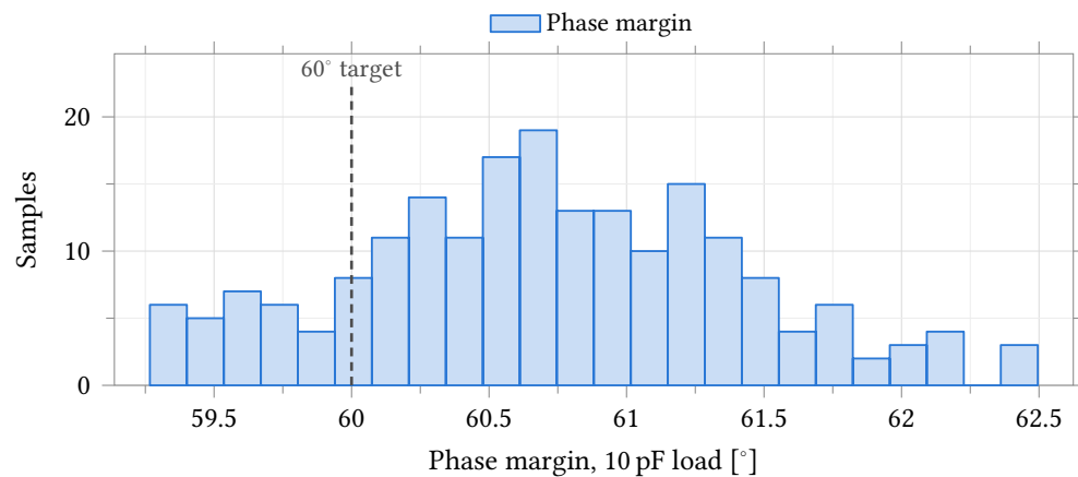
Figure 30: Phase margin driving the 10 pF test load, which is the worst case for this amplifier — a real cell adds resistive loading that lowers the loop gain and raises the margin (Table 18). 29 of 200 samples fall below the 60° target: 85.5 % per channel, 53.4 % across four. The worst is 59.3°, so no sample is near instability; it is the target that is missed.
