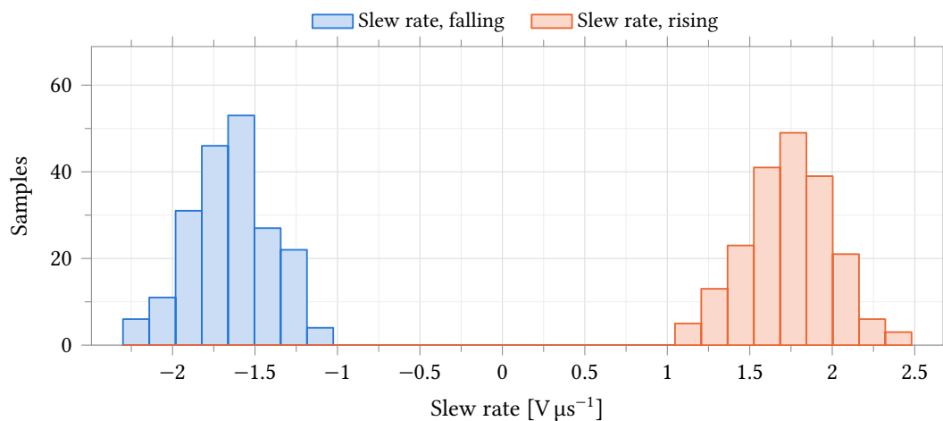
Figure 31: Slew rate on both edges of a 1 V step into 10 pF. Rising and falling averages are 1.74 \text{ V } \mu\text{s}^{-1} and 1.65 \text{ V } \mu\text{s}^{-1} , a 5 % imbalance: the tail current is steered into one input device and mirrored to the output, so the slewing current is equal in both directions by construction.
