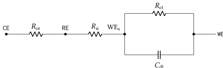
Figure 11: Three-electrode cell model randles_cell , the load the potentiostat actually drives. R_{ce} is the solution resistance from the counter to the reference electrode and R_u the uncompensated resistance from the reference to the working-electrode surface; the interface itself is the charge-transfer resistance R_{ct} in parallel with the double-layer capacitance C_{dl} . Values are given in Table 8. The model is lumped, linear and frequency-independent — no Warburg diffusion term and no potential dependence — so it represents small-signal behaviour about a bias point rather than a full electrochemical response.
