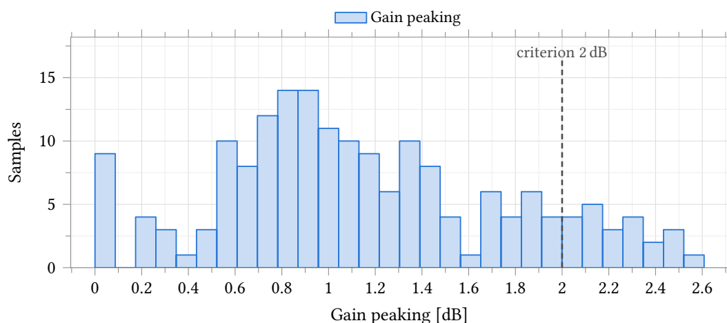
Figure 48: Closed-loop gain peaking at maximum gain, same 179 samples. 87.7 % sit below the 2 dB criterion, worst case 2.61 dB. Peaking fails before phase margin does because it responds to the same mismatch with less headroom against its limit; at R_f = 35 \text{ k}\Omega it is identically zero across every sample.
