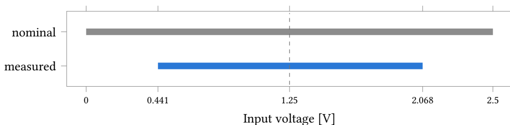
Figure 58: Usable input window of the converter against the nominal 0 V to 2.5 V supply span. The measured window runs 0.441 V to 2.068 V, 1.628 V wide, so 34.9 % of the nominal span is unreachable — 0.441 V at the bottom and 0.432 V at the top, near enough symmetric about the 1.25 V common mode (dashed). Outside that window the output sits at a code rail, so a transimpedance swing wider than \pm 0.81 V about V_{CM} is truncated rather than digitised.
