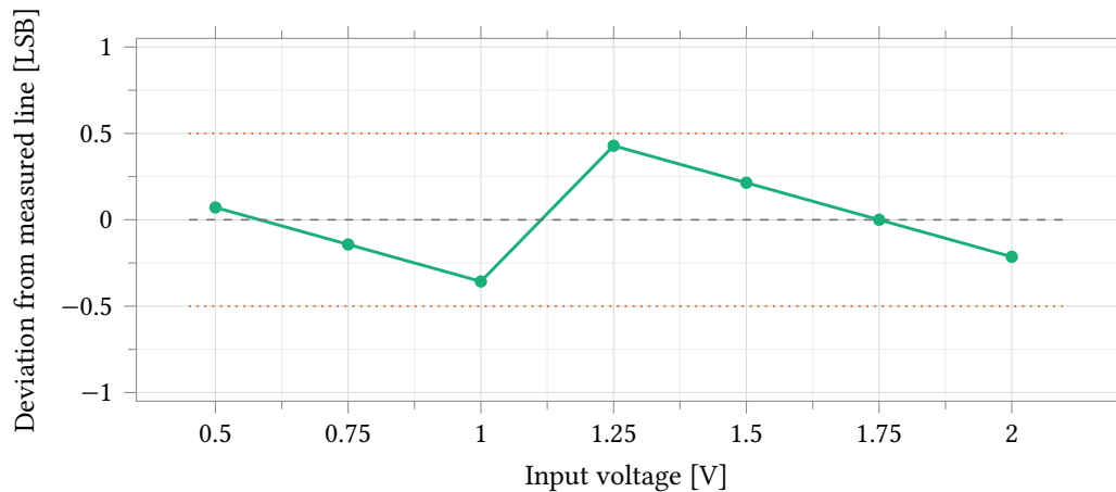
Figure 59: Deviation of each measured code from the converter’s own best-fit line, 628.85 codes/V, over the unclipped window. Referred to its own scale rather than the nominal one, the converter is straight to 0.429 LSB worst case and 0.247 LSB rms, against the \pm 0.5 LSB dotted guides — so the 168 LSB of Figure 57 is gain error alone and carries no linearity information. Seven points at 157 codes apart is a coarse grid: this bounds the deviation at the sampled inputs and is not a DNL or INL measurement, which needs every code.
