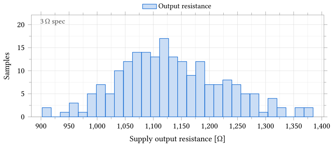
Figure 71: Output resistance of the DAC supply block, taken as the chord \Delta V / \Delta I over a 0 \mu A to 100 \mu A load sweep on VddDac. Process and mismatch , castalia_pm_25, 200 samples, 27 °C. The 3 \Omega limit entered on the test is two orders of magnitude below the data and is annotated at the left axis edge rather than drawn; no sample meets it. This is not a second defect: the reference movement of Figure 69 is this impedance multiplied by the ladder’s own code-dependent reference current.
