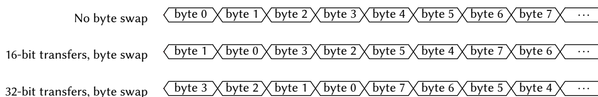
Figure 8: SPI Byte Ordering
