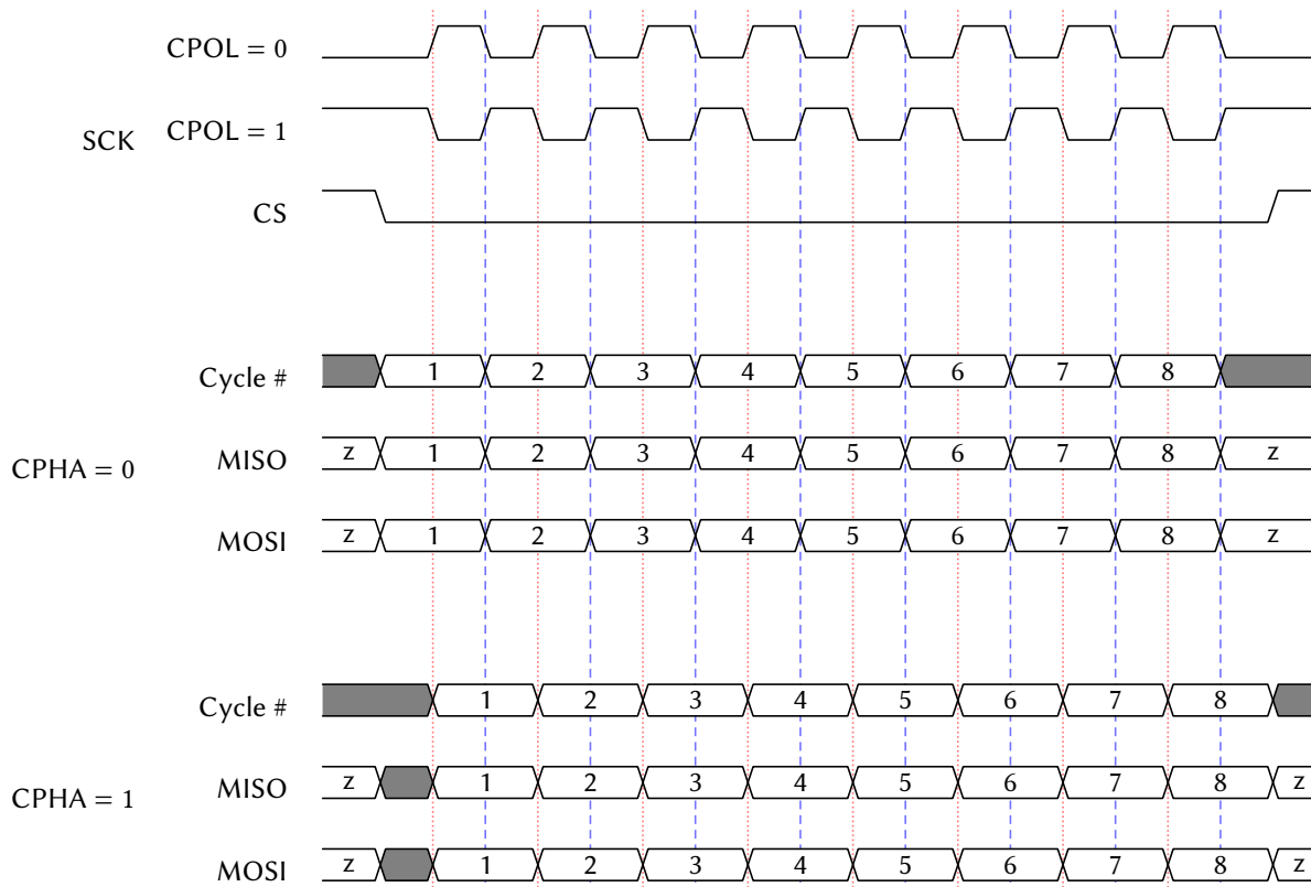
Figure 7: SPI Timing Diagram
