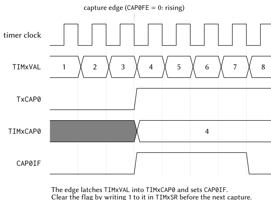
Figure 15: Input capture. The selected edge on TxCAP0 latches the live TIMxVAL into TIMxCAP0 and sets CAP0IF; the flag must be cleared by writing 1 to it in TIMxSR before the next capture event.
