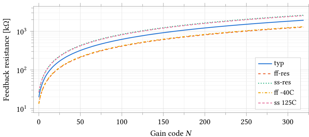
Figure 60: Measured resistance against gain code at all five corners, 500 nA forced through the A–B terminals with B held at V_{CM} = 1.25 V. The law is R = 18 \text{ k}\Omega + 6 \text{ k}\Omega \cdot N with N the binary value of ResEn<5:0> plus 64 per set ThEn<3:0> thermometer bit; every corner is strictly monotonic over all 320 codes, including the four thermometer seams. The corner families move the absolute value by -33 to +35 %, which is the poly sheet-resistance tolerance and must be absorbed by gain calibration, not by code choice.
