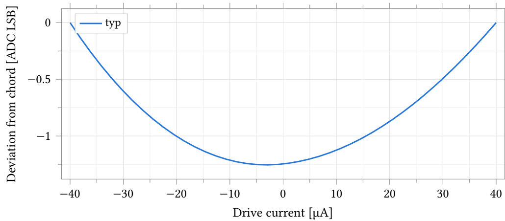
Figure 62: Drive nonlinearity of the bottom code ( N = 0 , R \approx 19.6 \text{ k}\Omega ): voltage deviation from the endpoint chord over \pm 90\% of full scale ( \pm 40 \mu\text{A} ), typical corner, expressed in 1.592 \text{ mV ADC LSB} . All ten bypass gates are closed at this code and carry the full signal current; their on-resistance rises with the terminal's excursion from V_{\text{CM}} , so the chord — pinned at the sweep endpoints where that excursion is largest — overestimates the mid-range voltage by up to 1.25 \text{ LSB} , and the deviation is bowl-shaped with a slight skew from the gates' voltage asymmetry. The same measurement at N = 63 and N = 319 , where the ladder dominates and current is 20\text{--}100\times smaller, stays below 0.004 \text{ LSB} and is tabulated, not plotted.
