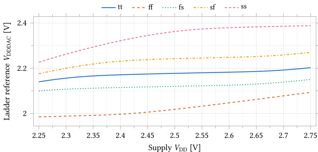
Figure 76: V_{\text{DDDAC}} against the supply, swept 2.25 \text{ V} to 2.75 \text{ V} , over five process corners at zero external load, 27^\circ\text{C} at point 1 and 25^\circ\text{C} at points 2–5. The slope is the line regulation tabulated in Table 79; it is not constant across the sweep, so the tabulated value is the chord between the two endpoints. The corner spread of the reference itself, 344 \text{ mV} at nominal supply, is larger than anything the supply sweep produces.
