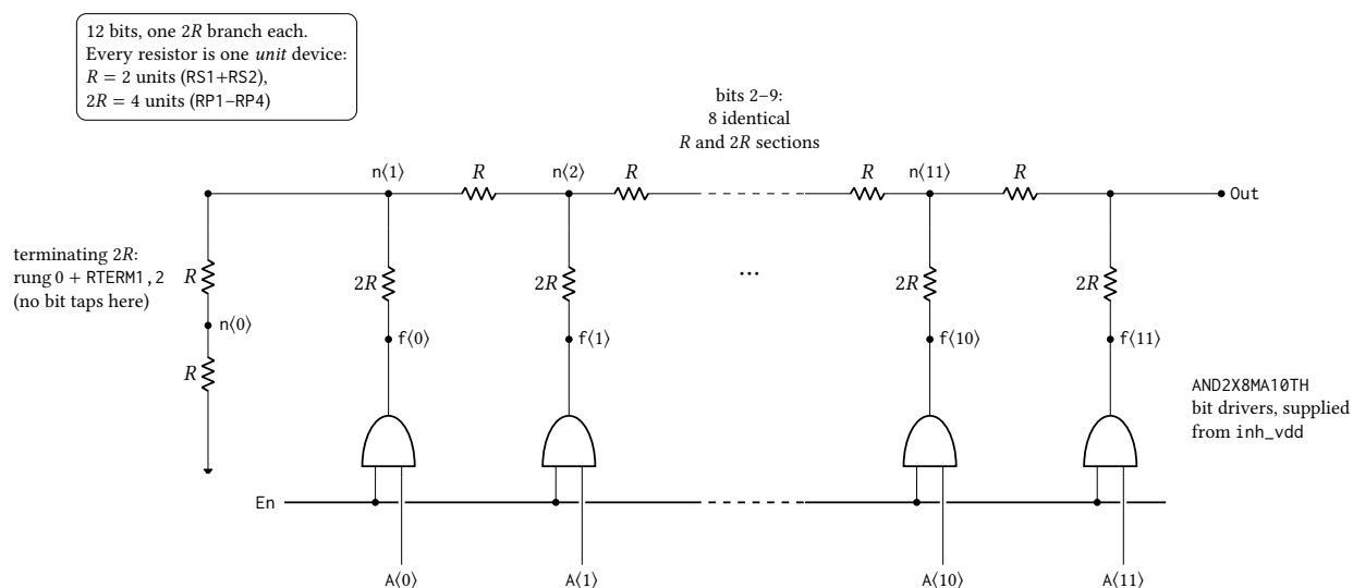
Figure 64: The 12-bit voltage-mode R-2R ladder of anatop_pixel_dacR2R12 , transcribed from the DacNonLinTB netlist. Bit k drives tap n\langle k+1 \rangle through its own 2R branch, so the twelve taps are n\langle 1 \rangle – n\langle 11 \rangle plus Out, and the MSB branch lands directly on Out at the top of the ladder; n\langle 0 \rangle carries no bit, its rung and RTERM1, 2 together forming the terminating 2R . Bits 2–9 are elided: eight further sections identical to those drawn sit between n\langle 2 \rangle and n\langle 11 \rangle . Every element is the same unit resistor, so the network itself is exact and gives \text{Out} = (\text{code}/4096) V_{\text{ref}} ; the reference is the output high level of the AND2X8MA10TH drivers, which sit in series with each 2R branch and bound the ladder in place of the rails — measured zero scale is 90 \mu\text{V} above V_{\text{SS}} and full scale 103 \mu\text{V} below the ideal (4095/4096) V_{\text{ref}} on a 2.5 \text{ V} rail. Device dimensions are proprietary and are not stated.
