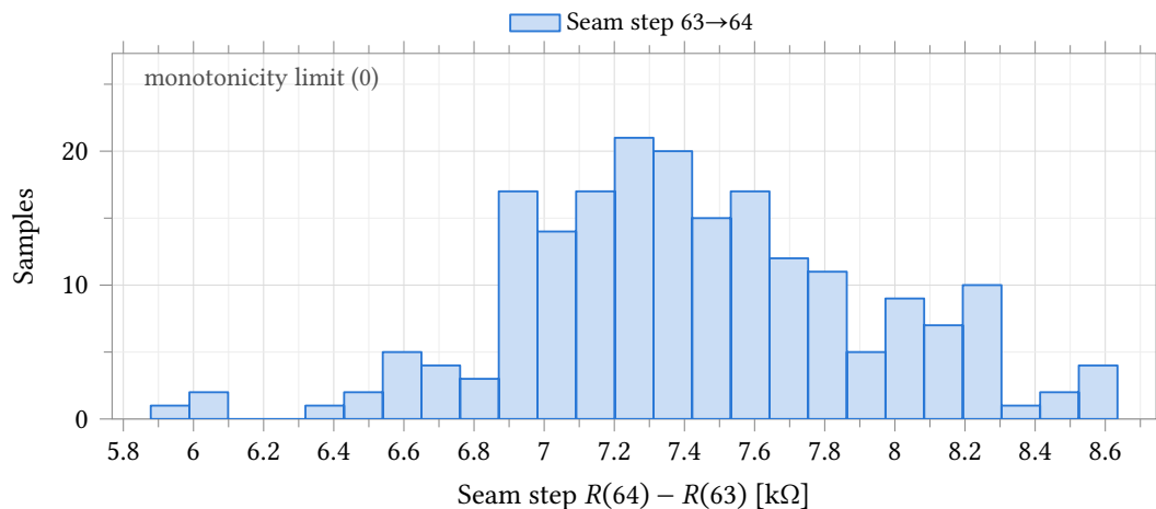
Figure 63: Per-sample step across the first thermometer seam (code 63 to 64: one 64-unit segment switches in while all six binary segments switch out), the code transition most exposed to mismatch. Mismatch only , model section castalia_pm_25 , nominal process, 200 samples, seed 12345, low-discrepancy sampling, 25 °C. Mean 7.42 kΩ, \sigma = 504 \Omega , worst sample 5.88 kΩ – 14.7 \sigma above the monotonicity limit at zero, so no realistic mismatch closes the seam.
