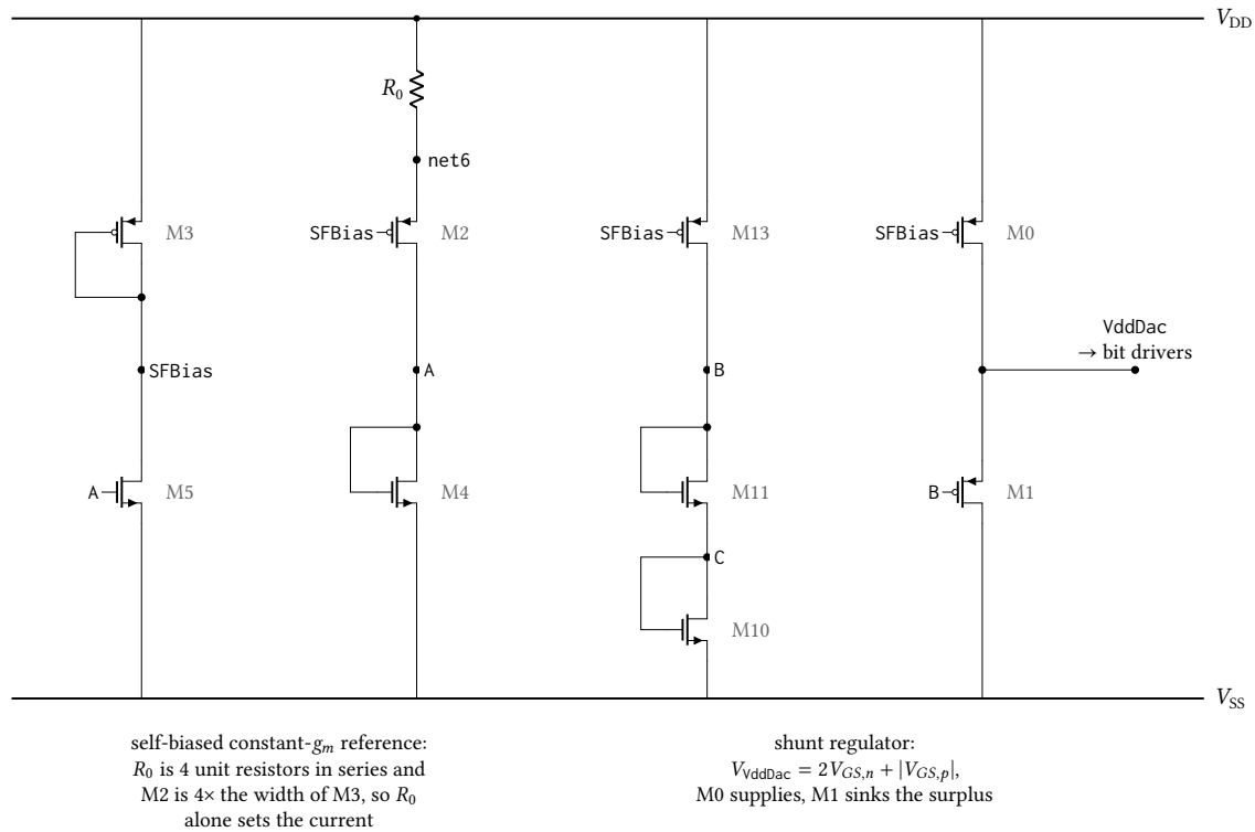
Figure 67: Core of anatop_pixel_dac_psu, the shunt regulator that generates the VddDac rail the ladder uses as its reference, transcribed from the LoadRegTB netlist. The self-biased constant- g_m reference on the left sets SFBias; M_{13} drives that current through the stacked diodes M_{11} and M_{10} to hold B two gate-source voltages above V_{SS} , and M_1 sinks whatever of M_0 's current the ladder leaves, clamping VddDac one PMOS gate-source voltage above B: 2.177 V unloaded from a 2.5 V rail. There is no error amplifier, so load regulation is set by M_1 's g_m alone. The five start-up and enable devices — the weak pull-up and its two kick devices on SU, the shutdown pull-up on SFBias and the En inverter — are omitted; none carries current once the loop is running. Device dimensions are proprietary and are not stated.
