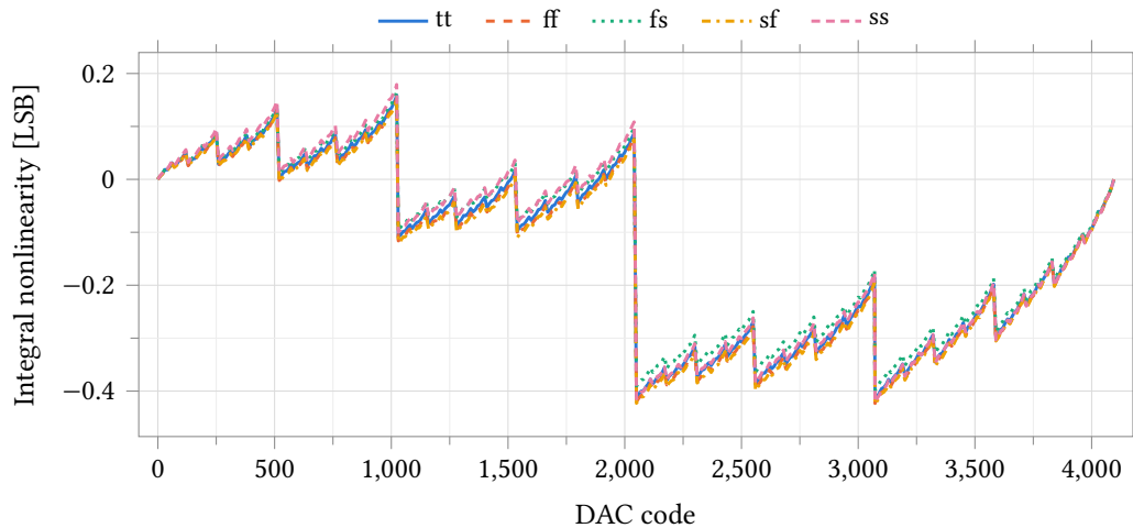
Figure 65: Integral nonlinearity against code over five process corners, ladder on an ideal 2.5 V rail, 25 °C, \text{reltol} = 1 \times 10^{-6} . INL is taken from the endpoint line through each corner’s own zero- and full-scale outputs, so it is zero at codes 0 and 4095 by construction. The positive extreme is code 1023, +0.15 to +0.18 LSB; the negative extreme is shared by the major carries at codes 2048 and 3072, which sit within 0.006 LSB of each other at -0.39 to -0.43 LSB at every corner. The code of each extreme is the same at all five corners: the shape is set by the ladder, not by the process. Corner run, no device mismatch — R-2R linearity is a matching property, so this envelope is the systematic term alone.
