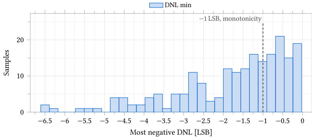
Figure 72: Worst negative differential nonlinearity, same bench, samples and conditions as Figure 71. The dashed rule at -1 LSB is the monotonicity limit entered on the test: 80 of 200 samples clear it, so 40 % of channels are monotonic and 0.40^4 = 2.6 % of four-channel chips are monotonic on all four. The distribution is left-skewed (skew -1.11 ) with a tail to -6.608 LSB, so the median -1.318 LSB and the percentiles of Table 73 describe it and mean \pm 3\sigma does not.
