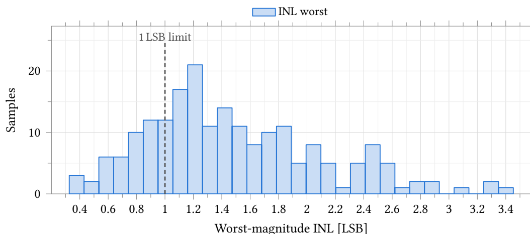
Figure 71: Integral nonlinearity of the R -2 R ladder driven from an ideal 2.5 V reference. Process and mismatch , model section castalia_pm_25 , 200 samples, seed 12345, low-discrepancy sampling, 25 °C, all 4096 codes. The dashed rule is the 1 LSB limit entered on the test; 42 of 200 samples fall inside it and the worst reaches 3.453 LSB. The distribution is right-skewed (Fisher skew +0.74), so Table 73 quotes the median and percentiles rather than \text{mean} \pm 3\sigma . LSB size, full scale and gain error are fixed to a part in 10^6 on this bench (Table 74), so the whole of this spread is resistor mismatch in the ladder and none of it is the reference.
