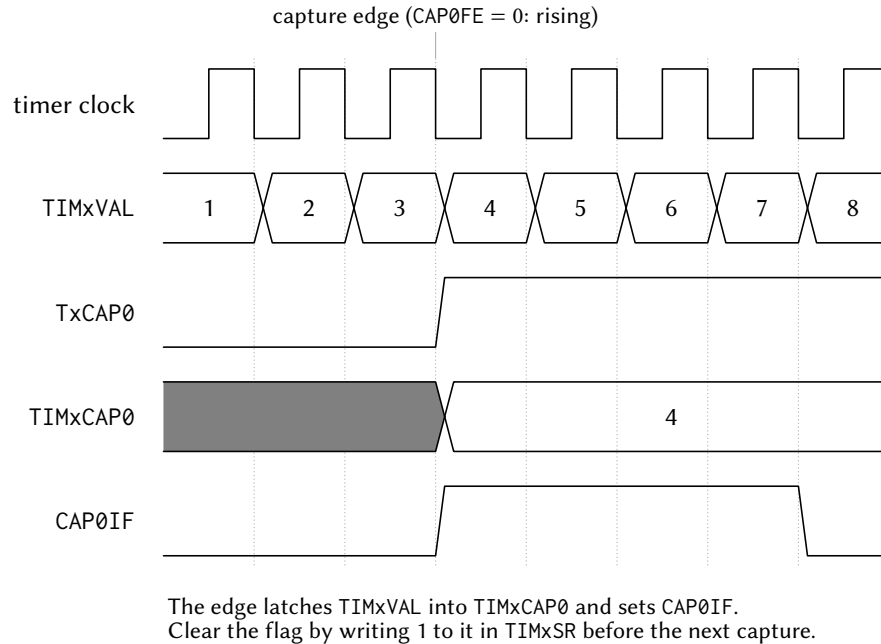
Figure 89: Input capture. The selected edge on TxCAP0 latches the live TIMxVAL into TIMxCAP0 and sets CAP0IF; the flag must be cleared by writing 1 to it in TIMxSR before the next capture event.
