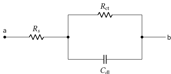
Figure 7: Single electrode–electrolyte interface, randles_electrode : a series solution resistance R_s ahead of the same charge-transfer and double-layer pair as Figure 6, presented as a two-terminal element. Values are given in Table 8; they describe a much smaller double layer and a much larger charge-transfer resistance than the three-electrode cell. None of the benches reported in this chapter uses it.
