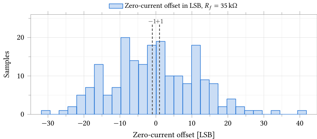
Figure 24.38: Zero-current output offset at R_f = 35 \text{ k}\Omega , in nominal 2.441 mV ADC LSB. Mismatch only , 25 °C nominal process, 200 samples, R_{ct} = 10 \text{ k}\Omega electrode. The limit shown is the \pm 1 LSB entered on the test in Assembler – comparable in kind across the four gain taps but mechanically harder to meet as R_f rises, since the underlying offset is closer to gain-independent in current (Table 24.53). The converter’s measured step is 1.591 mV, not the nominal 2.441 mV (Table 24.58); multiply the axis and the limit by 1.535 to read them as converter codes. Statistics are in Table 24.53.
