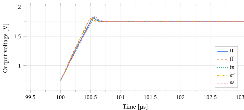
Figure 39: Rising edge of a 1 V step ( v_{cm} \pm 0.5 V) in unity feedback into 5 pF, over the five corners; the window is 3.5 \mu s around the edge at 100 \mu s, and the falling edge at 1.1 ms lies outside it. The output slews for about 0.4 \mu s, overshoots once by 5.0 % to 9.0 % of the step and recovers without ringing — slew recovery, not small-signal ringing, as the 88° phase margin predicts.
