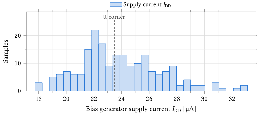
Figure 30: Supply current of the local bias generator over 200 process-and-mismatch samples, with the tt corner at the same trim code marked. Monte Carlo gives \sigma/\mu = 12.5\% , 17.7–33.1 \mu\text{A} , where the five process corners span 1.2 %, 23.25–23.52 \mu\text{A} (Table 10, interpolated to BiasAdj = 37); the corner sweep is at 27 °C against 37 °C here, which accounts for the 0.45 \mu\text{A} of mean offset and not for the width. A self-biased loop fixes its current by a device-ratio and resistor balance that a global corner shift leaves intact but local mismatch does not, so corner analysis under-reports this term tenfold. It is the largest single contributor to A1’s own spread – peak cell current 14.5 %, f_u 12.4 % – leaving roughly 7 % in quadrature for the amplifier’s own devices. This is a separate netlist and a separate draw, so sample n here is not sample n in the A1 tests and the two must not be paired.
