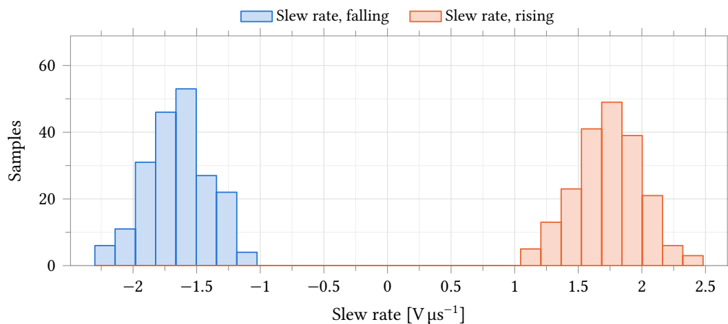
Figure 29: Slew rate on both edges of a 1 V step into 10 pF. Rising and falling averages are 1.74 \text{V } \mu\text{s}^{-1} and 1.65 \text{V } \mu\text{s}^{-1} , a 5 % imbalance: the tail current is steered into one input device and mirrored to the output, so the slewing current is equal in both directions by construction.
