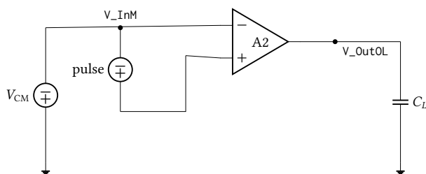
Figure 34: Open-loop slew testbench, SlewOpenLoopTB. The inverting input is held at V_{CM} and a floating pulse source drives the pair differentially rail to rail, into C_L = 5\ \text{pF} . With no feedback the output is driven hard in both directions, so the slew rates of Table 31 are open-loop full-swing values and bound the closed-loop settling rate rather than equalling it.
