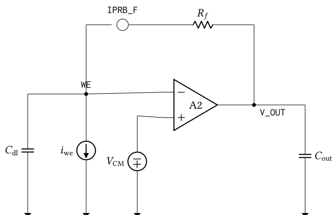
Figure 33: The closed transimpedance loop, TiaFbTB — the only bench in this section that closes feedback around the electrode. R_f returns the output to the working electrode through the probe IPRB_F, and i_{we} is the swept test source; every closed-loop figure in Section 7.4.3 comes from here. The electrode is a bare 1\ \mu\text{F} to ground, not the Randles cell of Figure 9 , which is why the reported peaking is an upper bound. The probe is present but only an ac analysis was run, so the loop gain itself is not measured.
