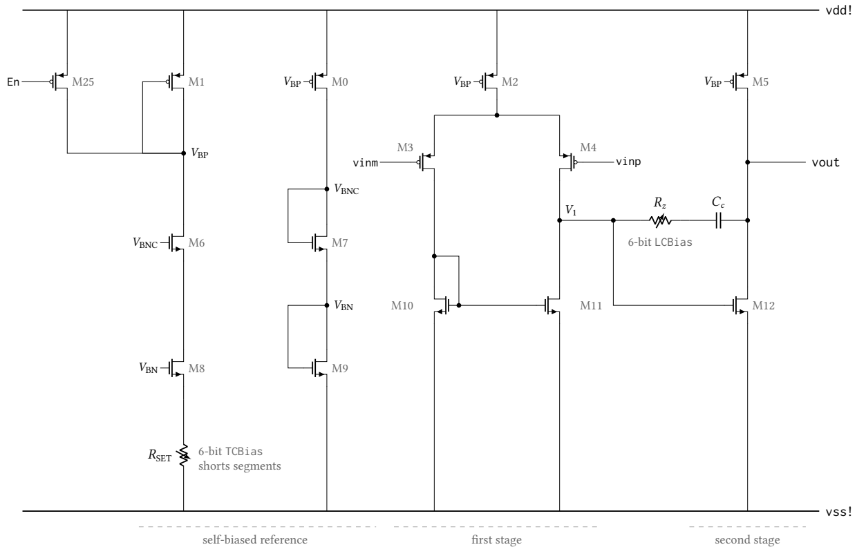
Figure 31: Simplified core of the transimpedance amplifier anatop_tiaamp , drawn from its netlist. First stage: PMOS pair M3/M4 on tail source M2 with NMOS current-mirror load M10/M11, output at V_1 ; second stage: common-source driver M12 with PMOS current-source load M5. The Miller branch R_z - C_c runs from V_1 to v_{out} , with M12's gate taken ahead of R_z ; C_c measures 1.00 pF. Being class A, the second stage sources the fixed current in M5 and sinks whatever M12 pulls — the asymmetry of Table 30. R_{SET} and R_z are each drawn as one trimmable resistor; both are segmented poly ladders with an NMOS shunt switch per trim bit. Device dimensions are omitted.
