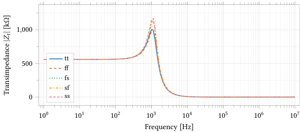
Figure 40: Transimpedance |Z_t| against frequency over the five corners, at maximum gain ( R_f = 560 \text{ k}\Omega ) with 1 \mu\text{F} of double-layer capacitance at the working electrode. Flat at 560 \text{ k}\Omega to about 200 \text{ Hz} , it peaks to 1.00 \text{ M}\Omega to 1.17 \text{ M}\Omega near 1 \text{ kHz} . The peak is a marginally stable loop caused by C_{dl} rolling the feedback factor off from 0.28 \text{ Hz} , not by the amplifier.
