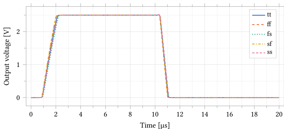
Figure 38: Open-loop large-signal response to a rail-to-rail input pulse into 5 pF, over the five corners. The falling edge is 1.7 times faster because the second stage is class A: M12 is a driven device, M5 a fixed current source.
