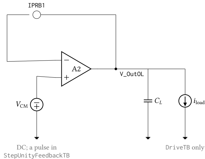
Figure 32: Unity-feedback testbench. The amplifier's output is returned to its inverting input through the current probe IPRB1 and loaded by C_L = 5 \text{ pF} ; a stb analysis through that probe gives the loop gain and phase, and dc and noise on the same wiring give the offset, tracking range and input-referred noise. Two variants share this schematic: DriveTB adds the swept load current i_{\text{load}} , and StepUnityFeedbackTB replaces the DC source with a pulse. Supplies, the bias trim buses and the enable pin are omitted here and in Figures 33 and 34.
