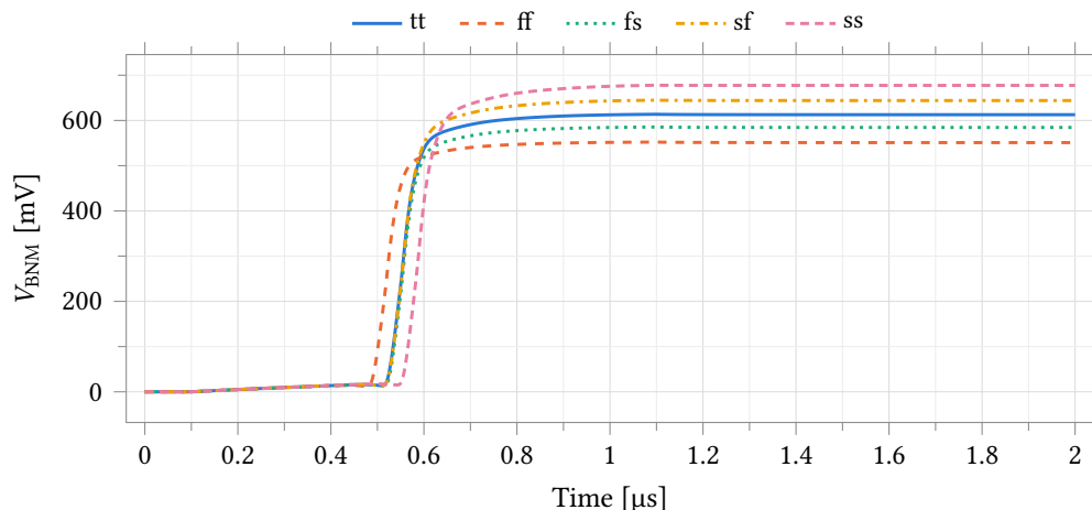
Figure 33: Power-up settling of V_{\text{BNM}} over all process corners.
