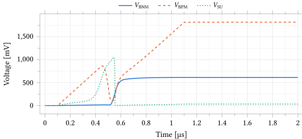
Figure 32: Power-up transient at the typical corner. The start-up node V_{SU} pulls the core out of its zero-current state, after which both mirror rails settle to their steady-state values.
