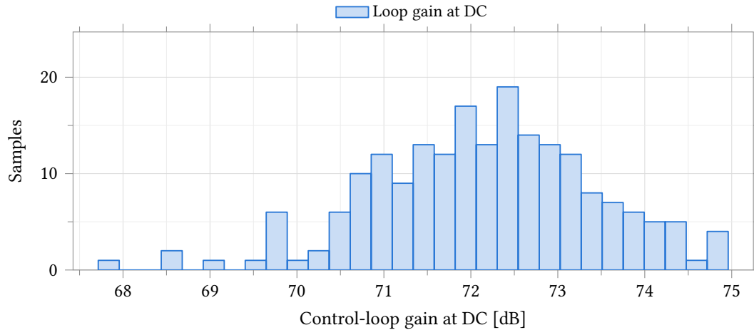
Figure 46: DC gain of the control loop closed around an electrochemical cell. Process and mismatch , 37 °C, 200 samples, cell-drive bench (Figure 44) with a Randles cell of R_{CE} = 1 k \Omega , R_u = 1 k \Omega , R_{ct} = 10 k \Omega , C_{dl} = 1 \mu F, working electrode at 1.25 V, C_L = 5 pF, C_c = 500 fF, 2.5 V supply. The loop is measured through the reference-electrode sense wire and therefore includes the cell, whose 12 k \Omega loads an open-loop output resistance of about 25 k \Omega and is 10 dB below the unity-feedback gain of Table 30. The spread is 7 dB peak to peak and no sample falls below 67 dB. No limit was entered on this output.
