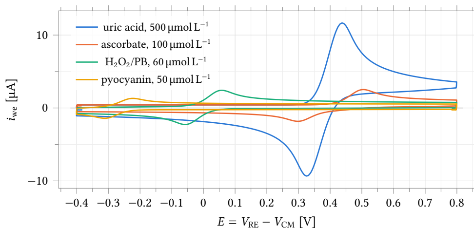
Figure 22: Voltammograms of the four-analyte wound panel through the rev-2 channel, one electrode_bc parameter set per channel, from the ps_cv Maestro corner run of Section 8.2 (2 V s -1 , R_f = 35 k \Omega , conditions of the in-loop run above). Peak potential identifies the analyte and peak height its concentration; each trace is one full cycle started at that analyte’s non-faradaic vertex. E^{0'} and concentrations are literature-anchored; k^0 is fitted (no measured value exists on carbon for any of the four), and reversal peaks appear for the chemically irreversible couples because following chemistry is not modelled. The two cathodic markers span -1.4 \mu\text{A} to -2.4 \mu\text{A} — unmeasurable by the unidirectional rev-1 front end.
