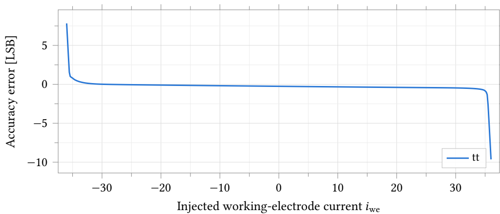
Figure 48: Bipolar accuracy error against injected working-electrode current, R_f = 35\text{ k}\Omega , R_{ct} = 10\text{ k}\Omega electrode, typical process point, 37 °C, full \pm 36\text{ }\mu\text{A} sweep (full scale \pm 33\text{ }\mu\text{A} ). The zero crossing is smooth with no kink or discontinuity between the sourcing and sinking halves of the sweep: the error’s slope through zero is -1/T exactly (Table 52) and the same single anatop_tia_amp_ab TIA feedback path serves both current directions, unlike the rev-1 PMOS-only mirror it replaces.
