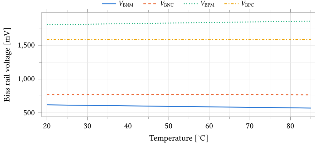
Figure 25: The four local bias rails against temperature at the typical corner. V_{\text{BNM}} and V_{\text{BNC}} are referred to v_{\text{ss}} !; V_{\text{BPM}} and V_{\text{BPC}} sit near the supply.
