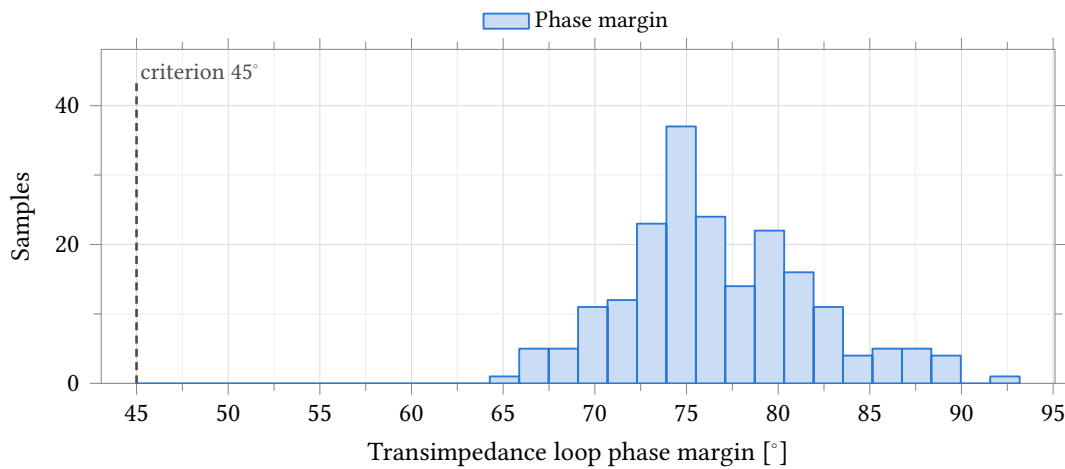
Figure 42: Phase margin of the transimpedance loop, conditions as Figure 41. The loop is measured through the feedback probe of Figure 38 and includes the amplifier, the feedback network and the Randles electrode ( R_s = 100\text{ }\Omega , R_{ct} = 1\text{ M}\Omega , C_{dl} = 100\text{ nF} ). All 200 samples clear the 45° criterion, minimum 64.7°. The distribution is right-skewed, so percentiles and the extreme sample are quoted in Table 41 rather than \pm 3\sigma .
