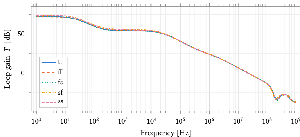
Figure 50: Potentiostat control-loop gain over five process corners, measured through the 0 \text{ V} probe IPRB1 in the RE feedback path (Figure 47). R_f = 35 \text{ k}\Omega , cell R_{ce} = R_u = 1 \text{ k}\Omega , R_{ct} = 10 \text{ k}\Omega , C_{dl} = 100 \text{ nF} , 2.5 \text{ V} supply. This is the full loop – A1, A2, both feedback networks and the electrode together – and is not the open-loop amplifier gain of Section 8.4. tt is at 37^\circ\text{C} , the four skew corners at 25^\circ\text{C} .
