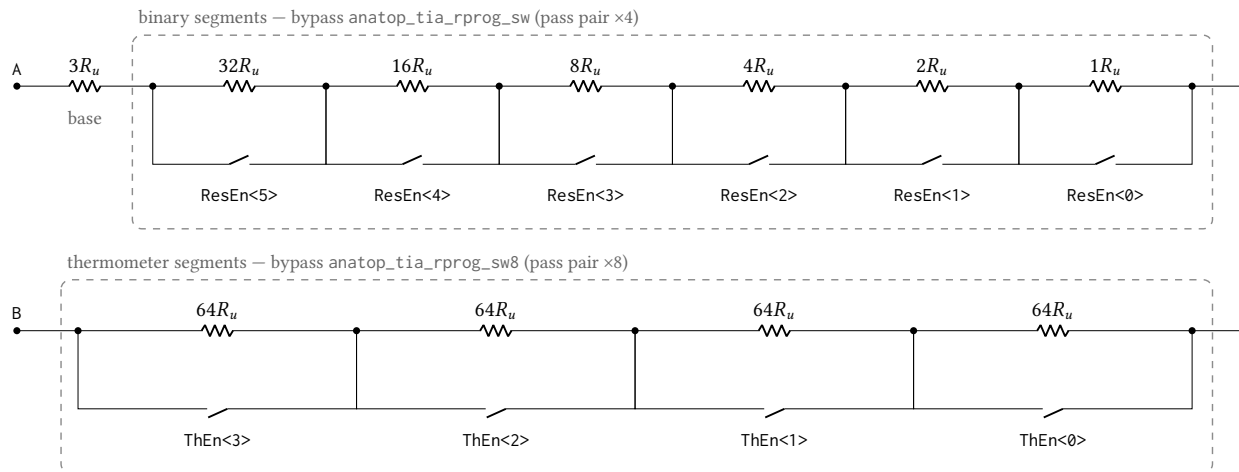
Figure 62: Segment and bypass-switch structure of anatop_tia_rprog, transcribed from the executed spec-run netlist. The unit R_u is one series poly resistor; from terminal A the chain runs through the never-switched three-unit base, the six binary-weighted segments of 32 down to 1 unit, and the four identical 64-unit thermometer segments to terminal B. Each switched segment is shunted by a CMOS transmission gate with a local inverter: the control pin EnBar is the ResEn/ThEn bit itself and drives the PMOS pass gate directly and the NMOS pass gate through the inverter, so a bit at 1 turns both pass devices off and inserts the segment. The pass pair has multiplicity 4 in the binary switch ( _sw ) and 8 in the thermometer switch ( _sw8 ), which halves the thermometer gates' on-resistance where up to six binary gates close at a seam. Three grounded dummy units accompany the 322 active units for matching.
