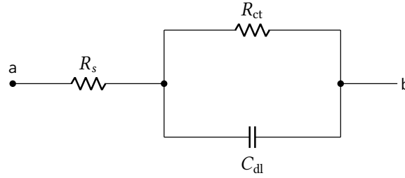
Figure 20: Single electrode–electrolyte interface: a series solution resistance R_s ahead of the same charge-transfer and double-layer pair as Figure 19, presented as a two-terminal element. Values are given in Table 12; they describe a much smaller double layer and a much larger charge-transfer resistance than the three-electrode cell. None of the benches reported in this chapter uses it.
