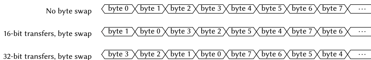
Figure 76: SPI Byte Ordering
