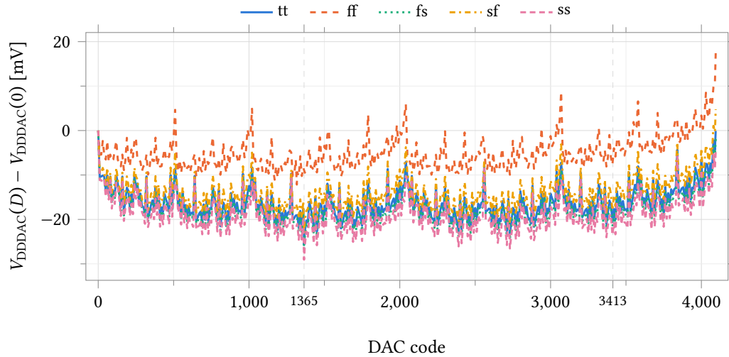
Figure 62: Ladder reference V_{DDAC} referred to its value at code 0, against DAC code, over five process corners, DacWPSUTB at 25 °C with the external load current set to zero. The ladder is the only load on the supply block and its current is code-dependent, so the reference the ladder divides moves 25.7 mV to 29.6 mV peak-to-peak with no external load at all; the absolute levels, which differ by 357 mV across corners, are Table 67. The two marked codes are alternating-bit patterns: 1365 = 0b0101010101 is the global minimum at four of the five corners (1317 at ff), and 3413 = 1365 + 2048 droops 23.4 mV at 2.5× the code weight and therefore sets the worst raw INL of Figure 63. Reference droop times code accounts for −36.9 of the −37.1 LSB measured there, so the raw nonlinearity of the delivered block is reference modulation and not a ladder error.
