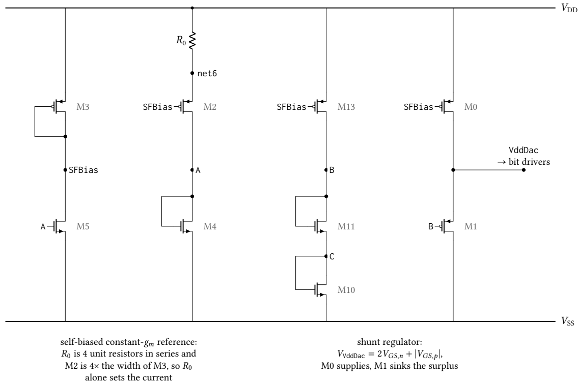
Figure 61: Core of anatop_pixel_dac_psu , the shunt regulator that generates the V_{ddDac} rail the ladder uses as its reference, transcribed from the LoadRegTB netlist. The self-biased constant- g_m reference on the left sets SFBias ; M13 drives that current through the stacked diodes M11 and M10 to hold B two gate-source voltages above V_{SS} , and M1 sinks whatever of M0's current the ladder leaves, clamping V_{ddDac} one PMOS gate-source voltage above B: 2.177 V unloaded from a 2.5 V rail. There is no error amplifier, so load regulation is set by M1's g_m alone. The five start-up and enable devices — the weak pull-up and its two kick devices on SU, the shutdown pull-up on SFBias and the En inverter — are omitted; none carries current once the loop is running. Device dimensions are proprietary and are not stated.
