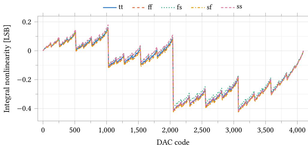
Figure 59: Integral nonlinearity against code over five process corners, ladder on an ideal 2.5 V rail, 25 °C, \text{reltol} = 1 \times 10^{-6} . INL is taken from the endpoint line through each corner's own zero- and full-scale outputs, so it is zero at codes 0 and 4095 by construction. The positive extreme is code 1023, +0.15 to +0.18 LSB; the negative extreme is shared by the major carries at codes 2048 and 3072, which sit within 0.006 LSB of each other at -0.39 to -0.43 LSB at every corner. The code of each extreme is the same at all five corners: the shape is set by the ladder, not by the process. Corner run, no device mismatch — R-2R linearity is a matching property, so this envelope is the systematic term alone.
