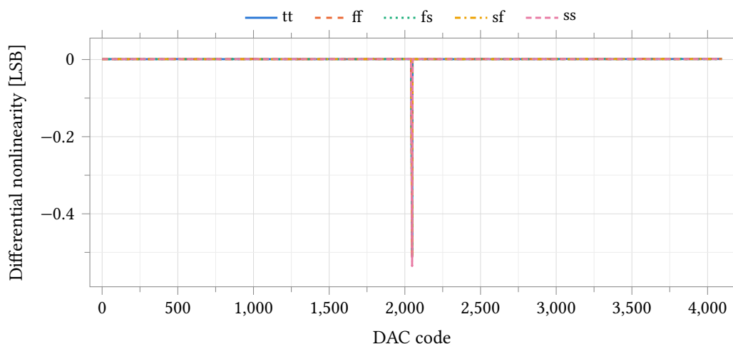
Figure 60: Differential nonlinearity against code over five process corners, conditions as Figure 59. DNL is the first difference of the transfer divided by the endpoint LSB, minus one. The worst step is the mid-scale major carry at code 2048, -0.50 to -0.54 LSB; the sub-carries measure -0.27 at code 1024, -0.23 at 3072, -0.14 at 512 and -0.13 LSB at 2560. The 4095-point curve is stride-decimated for the plot, so the comb drawn is a sample of the code grid and not every tooth of it; the extreme is preserved exactly. The converter is monotonic at every corner, with 0.46 LSB of margin to the -1 LSB limit at worst.
