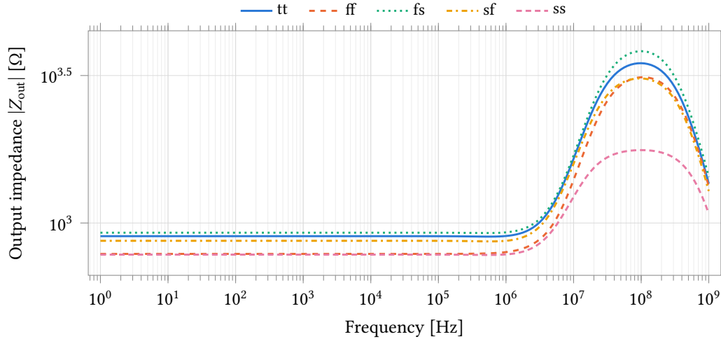
Figure 71: Magnitude of the supply block's output impedance against frequency over five process corners, 27 °C at point 1 and 25 °C at points 2–5. The AC load source carries unit magnitude, so |V_{DDDAC}| is the impedance in ohms. It is flat at 781 Ω to 927 Ω from 1 Hz to 100 kHz and peaks at 1.8 kΩ to 3.8 kΩ near 100 MHz. This is the small-signal impedance at zero load; the large-signal chord over the 0 μA to 100 μA sweep is 18 % to 51 % higher (Table 73).
