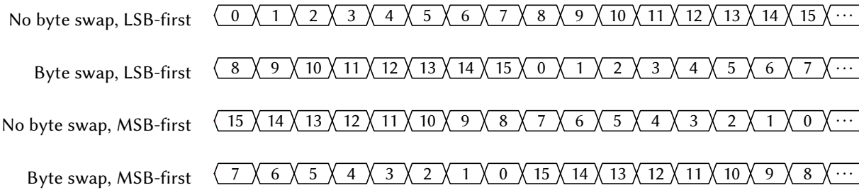
Figure 77: SPI Bit Ordering (16-bit transfer)
