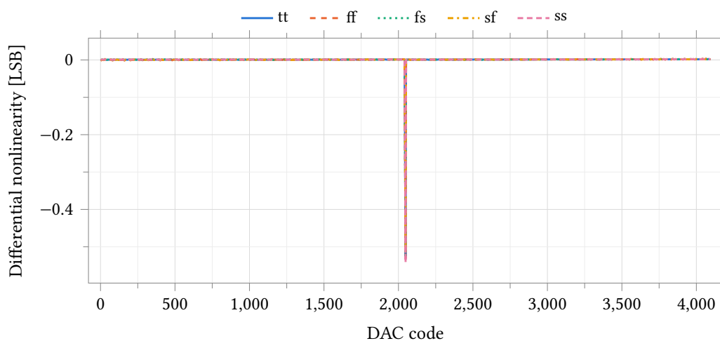
Figure 64: Ratiometric differential nonlinearity against code over five process corners: each code's output is divided by the reference measured at that code before the LSB and the first difference are taken, so the reference droop divides out and the ladder alone is measured. Conditions as Figure 63; the 4095-point curve is stride-decimated for the plot as in Figure 60. The major-carry hierarchy is the ideal-rail one — -0.53 at code 2048, then -0.28 at 1024, -0.24 at 3072, -0.14 at 512 and -0.13 LSB at 2560 — and the worst step matches Figure 60 to within 0.03 LSB. Raw DNL on the same bench is -9.8 to -18.4 LSB (Table 68); the difference is the reference step between adjacent codes and nothing else.
