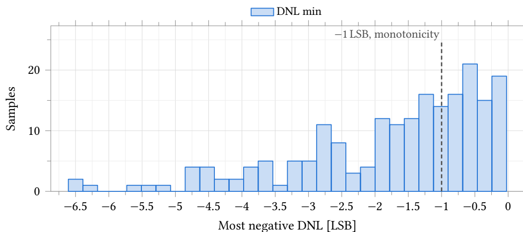
Figure 66: Worst negative differential nonlinearity, same bench, samples and conditions as Figure 65. The dashed rule at -1 LSB is the monotonicity limit entered on the test: 80 of 200 samples clear it, so 40 % of channels are monotonic and 0.40^4 = 2.6\% of four-channel chips are monotonic on all four. The distribution is left-skewed (skew -1.11 ) with a tail to -6.608 LSB, so the median -1.318 LSB and the percentiles of Table 69 describe it and \text{mean} \pm 3\sigma does not.
