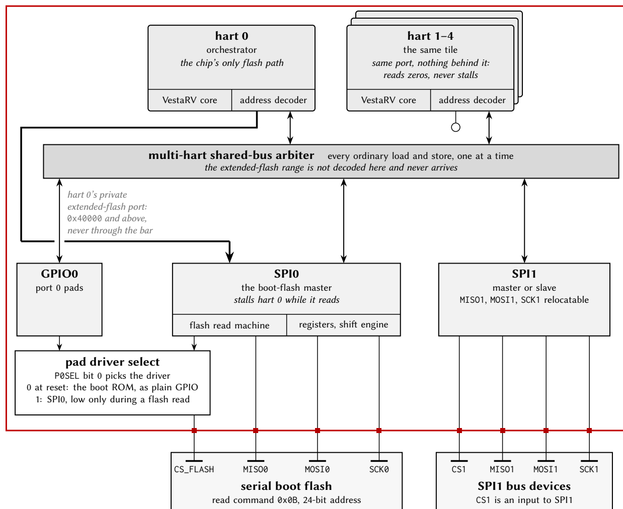
Figure 74: SPI connection diagram: SPI0 and the boot flash. Everything drawn is generated from this configuration. SPI0's registers are an ordinary arbiter slave, so every hart reaches them the same way, through the bar. The flash is different: hart 0's own address decoder claims every address at or above 0x40000 — the strict complement of the shared window — and takes it out of the tile on a private port that never reaches the bar and is never arbitrated, which is what makes execute-in-place possible (Section 16.10). SPI0 turns each such access into a flash read, sending the command byte and then (\text{CPU address} + \text{SPI0FOS}) \bmod 2^{24} , and stalls hart 0 until the word comes back. Every other hart has the same decoder and the same port with nothing behind it, so its accesses in that range read zeros and do not stall. CS_FLASH has two drivers and the pad's PxSEL bit chooses between them: it resets to 0, a plain GPIO output driven high, which is how the boot ROM clocks the flash before any of this is set up. SPI1, in configurations that include it, is a separate block with its own pins and no flash path of any kind.
