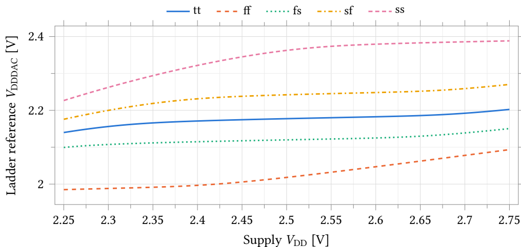
Figure 85: V DDDAC against the supply, swept 2.25 V to 2.75 V, over five process corners at zero external load, 27 °C at point 1 and 25 °C at points 2–5. The slope is the line regulation tabulated in Table 92; it is not constant across the sweep, so the tabulated value is the chord between the two endpoints. The corner spread of the reference itself, 344 mV at nominal supply, is larger than anything the supply sweep produces.
