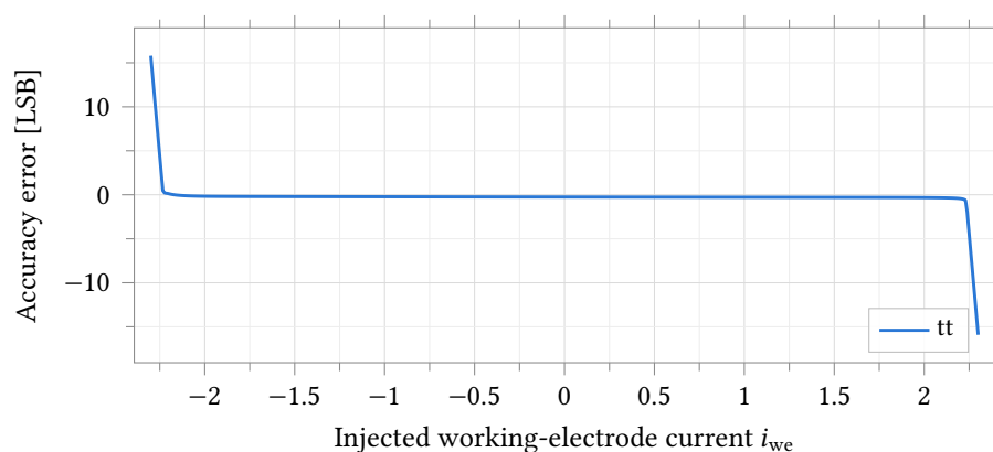
Figure 33.33: Accuracy error at the operational max-gain point, R_f = 560\text{ k}\Omega into R_{ct} = 1\text{ M}\Omega , typical process point, 37\text{ }^\circ\text{C} . The truth current sweep is \pm 2.3\text{ }\mu\text{A} , just beyond the 2.06\text{ }\mu\text{A} full-scale current at this gain tap; the crossing at zero is smooth, with no kink, over the full swept range shown. The error axis is referred to the nominal 2.441\text{ mV} step; the converter's measured step is 1.591\text{ mV} (Table 33.58), so multiply by 1.535 to read it as converter codes.
