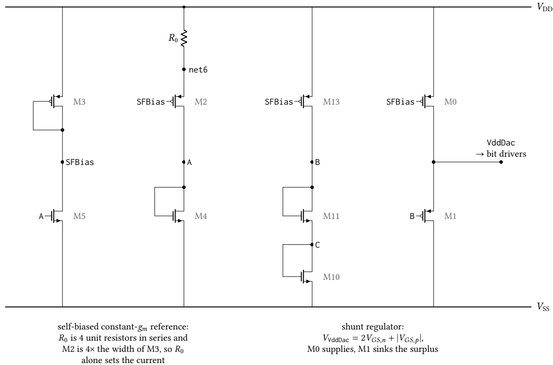
Figure 75: Core of anatotop_pixel_dac_psu, the shunt regulator that generates the VddDac rail the ladder uses as its reference, transcribed from the LoadRegTB netlist. The self-biased constant- g_m reference on the left sets SFBias; M13 drives that current through the stacked diodes M11 and M10 to hold B two gate-source voltages above V_{SS} , and M1 sinks whatever of M0's current the ladder leaves, clamping VddDac one PMOS gate-source voltage above B: 2.177 V unloaded from a 2.5 V rail. There is no error amplifier, so load regulation is set by M1's g_m alone. The five start-up and enable devices — the weak pull-up and its two kick devices on SU, the shutdown pull-up on SFBias and the En inverter — are omitted; none carries current once the loop is running. Device dimensions are proprietary and are not stated.
