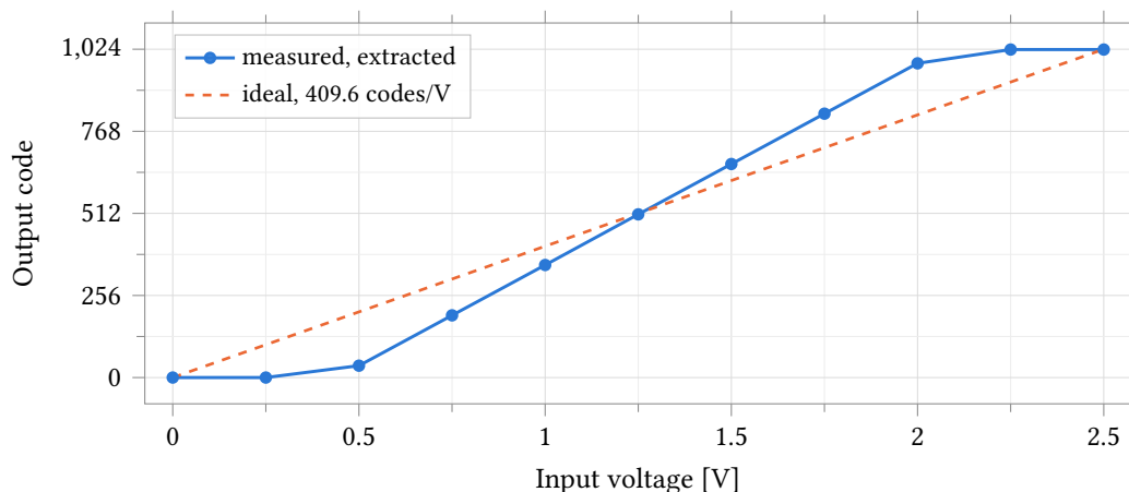
Figure 63: Output code against input voltage for the extracted anatop_pixel_adc , nominal corner, 37 °C, 2.5 V analog and 1.0 V digital supplies, with the ideal 409.6 codes/V line overlaid. The transfer is monotonic and reaches both code limits, but its slope is 628.64 codes/V — 1.535 times ideal — so the flat segments below 0.44 V and above 2.07 V are the code limits, not the ends of the sweep. Markers are the eleven simulated points; the 0.25 V step is 157 codes, so the curve between them is interpolation and carries no linearity information.
