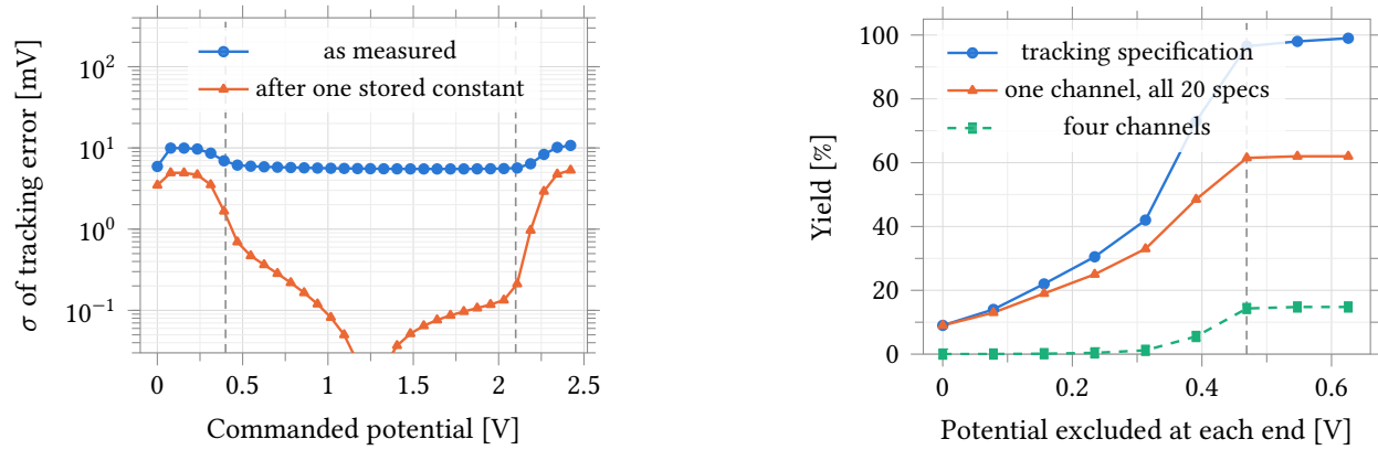
Figure 60: Reference tracking on the assembled channel, 200 samples, process and mismatch, nominal process point, 37 °C. Left: the spread of V_{RE} - V_{PATTERN} against the commanded potential, as measured and after the same sample’s mid-code value is subtracted — the residual one stored per-channel constant leaves behind, zero at mid-code by construction and off the axis there. Dashed lines mark the specified window; interior to it the error is a pure constant to 0.36 mV, while outside it A1’s input pair is leaving its common-mode range and no constant reaches the remainder. Right: yield against how much commanded potential the 2 mV tracking specification excludes at each end, after that calibration, on the sweep’s 128-code grid; the 0.4 V to 2.1 V window selects the points from 0.469 to 1.952 V and is the dashed line. Every yield is an upper bound (Section 8.6.9), and the per-channel curve saturates at 62 % because the reference-electrode floor of Table 67, not tracking, then binds.
