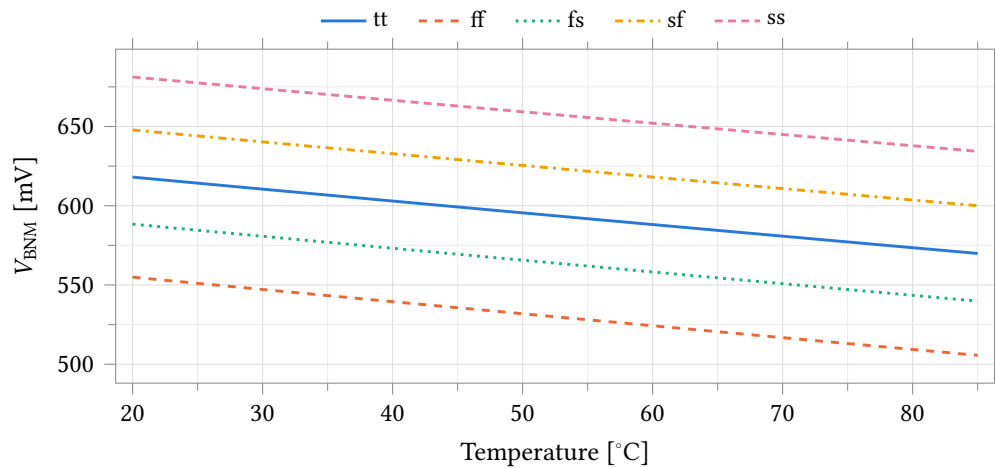
Figure 34.10: NMOS mirror bias V_{\text{BNM}} against temperature over all process corners. The corner separation drawn here is a lower bound: the corner set holds the passive model rows at typical (pinned-passive caveat, page 295).
