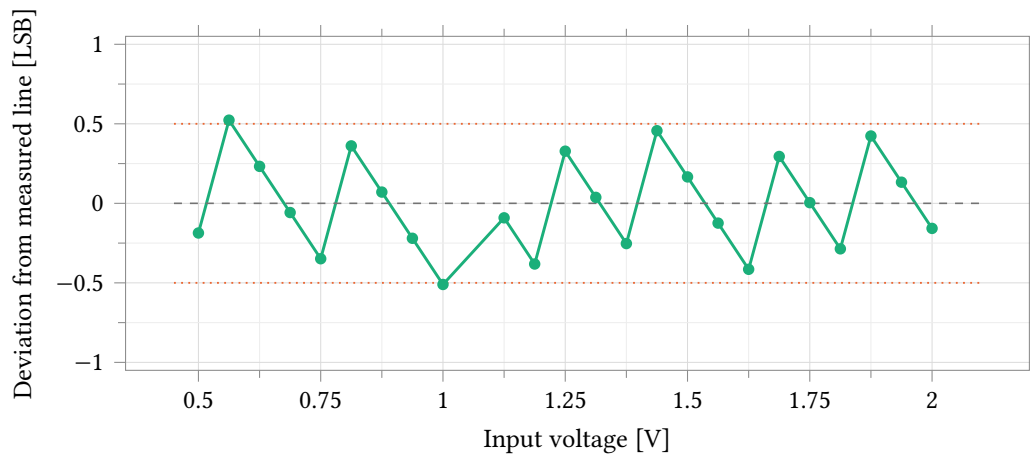
Figure 34.45: Deviation of each measured code from the converter's own best-fit line, 628.64 codes/V, over a 0.0625 V sweep of the unclipped window. Referred to its own scale rather than the nominal one the converter is straight to 0.523 LSB worst case and 0.294 LSB rms, so the 168 LSB of Figure 34.43 is gain error alone and carries no linearity information. The worst point sits just outside the \pm 0.5 LSB dotted guides. Twenty-four points 39 codes apart bound the deviation at the sampled inputs; a DNL or INL measurement needs every code and this grid does not provide one. A twenty-fifth point at 1.0625 V is absent because its simulation returned an error.
