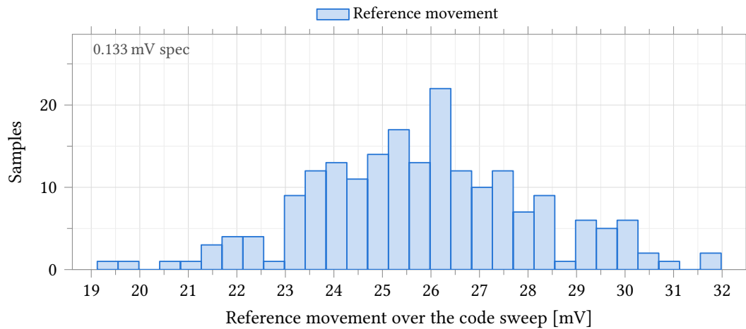
Figure 34.60: Peak-to-peak movement of the DAC reference VddDac across the 4096-code sweep, with the ladder referenced to the on-chip supply block instead of an ideal rail. Process and mismatch , castalia_pm_25, 200 samples, 25 °C, no external load on VddDac. The quarter-LSB budget of 133 \mu\text{V} entered on the test sits about 200 times below the data, so it is annotated at the left axis edge rather than drawn and the distribution is not compressed into a single bar; the closest sample misses it by a factor of 144. Meeting it needs the supply’s output impedance down by a factor of 193, to about 5 \Omega , against 894 \Omega small-signal (Table 34.81) and 1133 \Omega as a 0 \mu\text{A} to 100 \mu\text{A} chord (Table 34.77).
