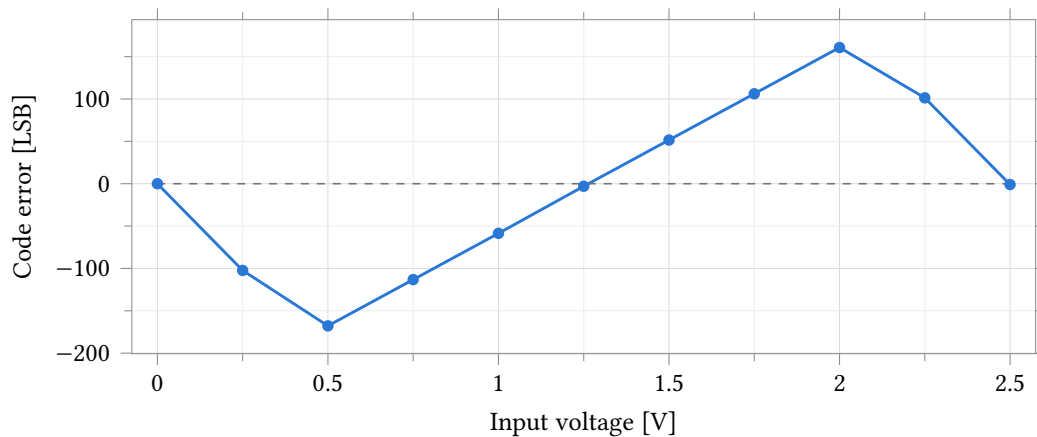
Figure 34.43: Code error against input voltage, measured code minus the ideal 409.6 codes/V line, from the same run as Figure 34.42. The error is the 1.535 slope ratio, not nonlinearity: it reaches -167.8 LSB at 0.5 V and 160.8 LSB at 2.0 V, crossing zero near the 1.25 V common mode where the measured and ideal lines intersect. It also returns near zero at 0 V and 2.5 V, where the clipped output coincides with the ideal endpoints; those two points are not accuracy. Referred to the fitted line instead, the residual over 0.5 V to 2.0 V is at most 0.52 LSB.
