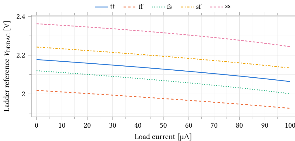
Figure 34.61: V_{\text{DDDAC}} against external load current over five process corners, supply block alone, 27 °C at point 1 and 25 °C at points 2–5, ADE default tolerances. There is no feedback loop around the output, so the slope is the block’s own output resistance and the reference falls 92.7 mV to 119.3 mV across the 0 \mu\text{A} to 100 \mu\text{A} sweep. The curve steepens with load, which is why the chord in Table 34.76 exceeds the small-signal |Z_{\text{out}}| of Table 34.80. This sweep is an external load only: the ladder is not connected on this bench, and its own code-dependent draw is Figure 34.57.
