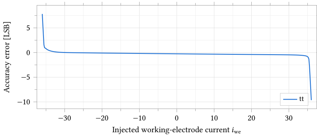
Figure 34.32: Bipolar accuracy error against injected working-electrode current, R_f = 35\text{ k}\Omega , R_{ct} = 10\text{ k}\Omega electrode, typical process point, 37 °C, full \pm 36\text{ }\mu\text{A} sweep (full scale \pm 33\text{ }\mu\text{A} ). The zero crossing is smooth with no kink or discontinuity between the sourcing and sinking halves of the sweep: the error’s slope through zero is -1/T exactly (Table 34.42) and the same single anatop_tia_amp_ab TIA feedback path serves both current directions, unlike the rev-1 PMOS-only mirror it replaces. The error axis is referred to the nominal 2.441 mV step; the converter’s measured step is 1.591 mV (Table 34.58), so multiply by 1.535 to read it as converter codes.
