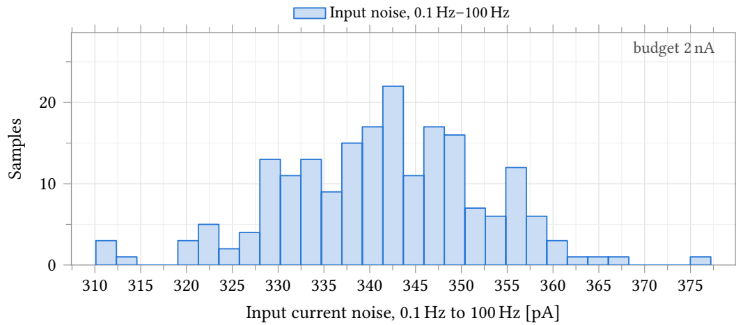
Figure 34.27: Input-referred current noise integrated 0.1 Hz to 100 Hz, conditions as Figure 34.25. Output noise divided by R_f , from a noise analysis that runs 0.1 Hz to 10 kHz at 20 points per decade. The 2 nA budget entered on the test is about six times the measured value and is annotated at the axis edge rather than drawn, so that the 310 pA to 377 pA spread stays legible. The figure scales inversely with the selected gain tap.
