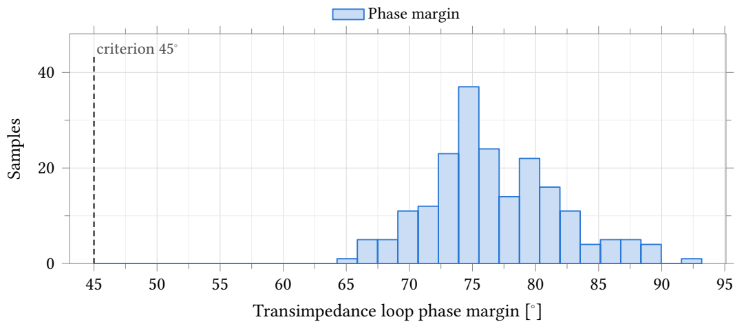
Figure 34.26: Phase margin of the transimpedance loop, conditions as Figure 34.25. The loop is measured through the feedback probe of Figure 34.22 and includes the amplifier, the feedback network and the Randles electrode ( R_s = 100\ \Omega , R_{ct} = 1\ \text{M}\Omega , C_{dl} = 100\ \text{nF} ). All 200 samples clear the 45^\circ criterion, minimum 64.7^\circ . The distribution is right-skewed, so percentiles and the extreme sample are quoted in Table 34.31 rather than \pm 3\sigma .
