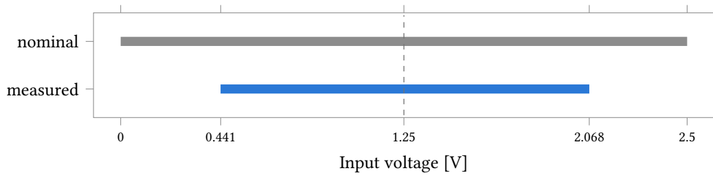
Figure 34.44: Usable input window of the converter against the nominal 0 V to 2.5 V supply span. The measured window runs 0.441 V to 2.068 V, 1.627 V wide, so 34.9 % of the nominal span is unreachable: 0.441 V at the bottom and 0.432 V at the top, near enough symmetric about the 1.25 V common mode (dashed). Outside that window the output sits at a code rail, so a transimpedance swing wider than \pm 0.81 V about V_{CM} is truncated rather than digitised.
