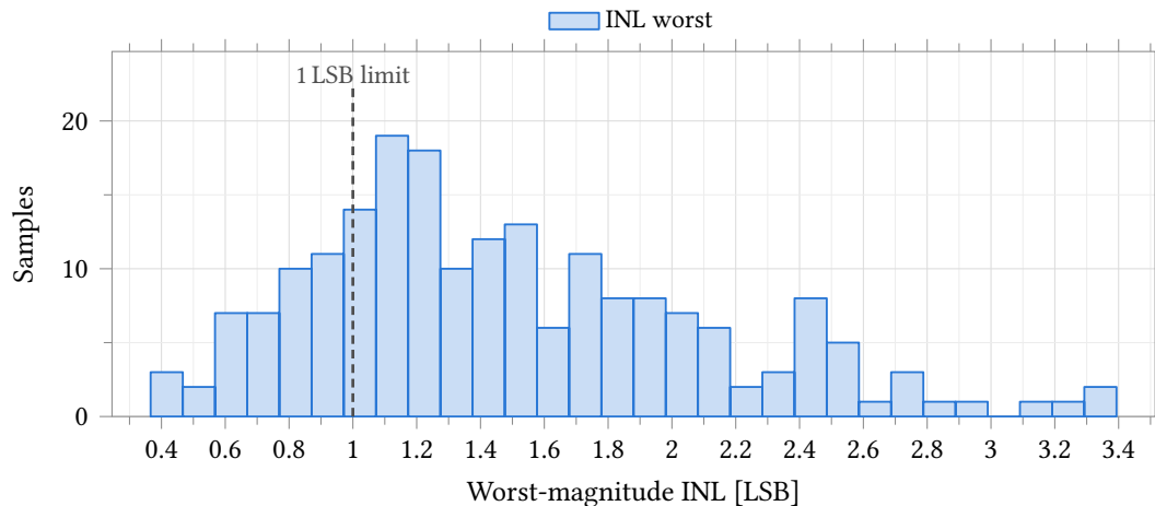
Figure 34.54: Integral nonlinearity of the R - 2R ladder driven from an ideal 2.5 V reference, with the custom 2.5 V bit driver anatop_and2_dac the tapeout cell carries. Process and mismatch , model section castalia_pm_25 , 200 samples, seed 12345, low-discrepancy sampling, 25 °C, all 4096 codes. The dashed rule is the 1 LSB limit entered on the test; 41 of 200 samples fall inside it and the worst reaches 3.393 LSB. The distribution is right-skewed (Fisher skew +0.74 ), so Table 34.70 quotes the median and percentiles rather than \text{mean} \pm 3\sigma . LSB size, full scale and gain error are fixed to a part in 10^6 on this bench (Table 34.71), so the whole of this spread is resistor mismatch in the ladder and none of it is the reference.
