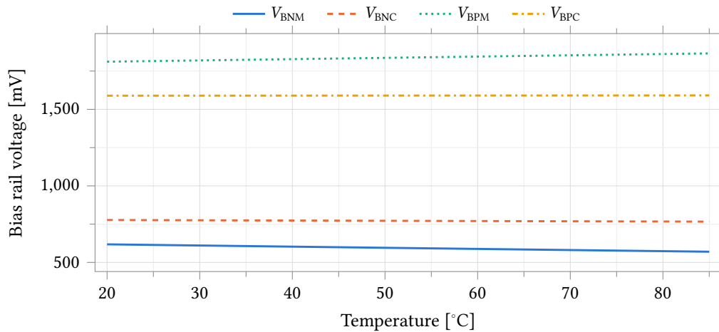
Figure 34.9: The four local bias rails against temperature at the typical corner. V_{\text{BNM}} and V_{\text{BNC}} are referred to vss!; V_{\text{BPM}} and V_{\text{BPC}} sit near the supply.
