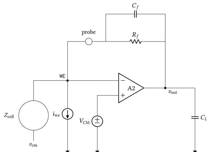
Figure 34.22: The closed transimpedance loop bench, the only one in this section that closes feedback around the electrode. R_f \parallel C_f returns the output to the working electrode through a current probe, i_{we} is the test source, and Z_{cell} is the Randles cell of Figure 34.1, returned to v_{cm} . The loop gain, phase margin and crossover are measured through the probe; the DC accuracy, closed-loop transfer and noise figures come from the same wiring.
