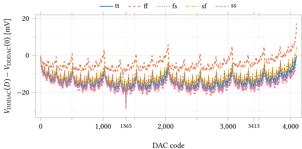
Figure 34.57: Ladder reference V_{DDDAC} referred to its value at code 0, against DAC code, over five process corners, DacWPSUTB at 25 °C with the external load current set to zero. The ladder is the only load on the supply block and its current is code-dependent, so the reference the ladder divides moves 25.7 mV to 29.6 mV peak-to-peak with no external load at all; the absolute levels, which differ by 357 mV across corners, are Table 34.72. The two marked codes are alternating-bit patterns: 1365 = 0b0101010101 is the global minimum at four of the five corners (1317 at ff), and 3413 = 1365 + 2048 droops 23.4 mV at 2.5× the code weight and therefore sets the worst raw INL of Figure 34.58. Reference droop times code accounts for −36.9 of the −37.1 LSB measured there, so the raw nonlinearity of the delivered block is reference modulation and not a ladder error.
