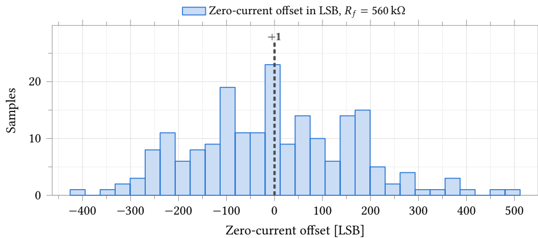
Figure 34.39: Zero-current output offset at R_f = 560\text{ k}\Omega , conditions as Figure 34.38 but at R_{ct} = 10\text{ k}\Omega (the same stiff electrode as the finite-loop-gain demonstration of Table 34.44, NOT the 1 M \Omega operational electrode of Table 34.43). Some samples reach the sweep’s output rails (Table 34.53); the LSB spread here is 14 \times wider than at 35 k \Omega for the same underlying current offset, since the same offset current is multiplied through a 16 \times larger R_f .
