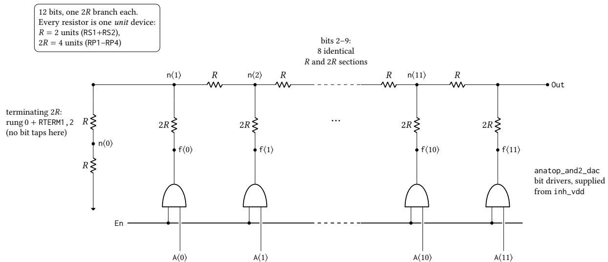
Figure 34.51: The 12-bit voltage-mode R - 2R ladder of anatop_pixel_dacR2R12 , transcribed from the DacNonLinTB netlist. Bit k drives tap n(k+1) through its own 2R branch, so the twelve taps are n(1) – n(11) plus Out, and the MSB branch lands directly on Out at the top of the ladder; n(0) carries no bit, its rung and R_{TERM1,2} together forming the terminating 2R . Bits 2–9 are elided: eight further sections identical to those drawn sit between n(2) and n(11) . Every element is the same unit resistor, so the network itself is exact and gives \text{Out} = (\text{code}/4096) V_{\text{ref}} ; the reference is the output high level of the anatop_and2_dac drivers, which sit in series with each 2R branch and bound the ladder in place of the rails: measured zero scale is 20 nV above V_{\text{SS}} and full scale 1.2 \mu\text{V} below the ideal (4095/4096) V_{\text{ref}} on a 2.5 V rail. Device dimensions are proprietary and are not stated.
