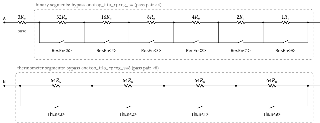
Figure 34.46: Segment and bypass-switch structure of anatop_tia_rprog , transcribed from the executed spec-run netlist. The unit R_u is one series poly resistor; from terminal A the chain runs through the never-switched three-unit base, the six binary-weighted segments of 32 down to 1 unit, and the four identical 64-unit thermometer segments to terminal B. Each switched segment is shunted by a CMOS transmission gate with a local inverter: the control pin EnBar is the ResEn/ThEn bit itself and drives the PMOS pass gate directly and the NMOS pass gate through the inverter, so a bit at 1 turns both pass devices off and inserts the segment. The pass pair has multiplicity 4 in the binary switch ( _sw ) and 8 in the thermometer switch ( _sw8 ), which halves the thermometer gates' on-resistance where up to six binary gates close at a seam. Three grounded dummy units accompany the 322 active units for matching.
