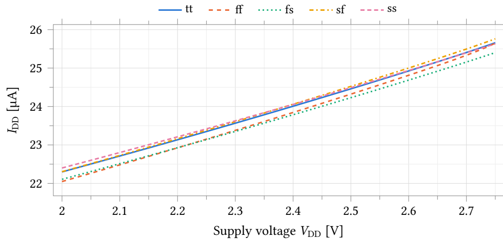
Figure 34.13: Quiescent supply current against supply voltage over all process corners. The corner separation drawn here is a lower bound: the corner set holds the passive model rows at typical (pinned-passive caveat, page 295).
