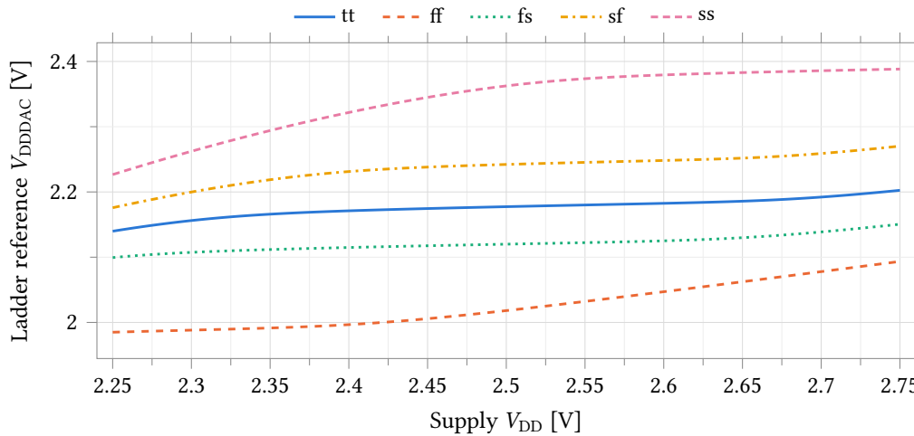
Figure 34.63: V_{DDDAC} against the supply, swept 2.25 V to 2.75 V, over five process corners at zero external load, 27 °C at point 1 and 25 °C at points 2–5. The slope is the line regulation tabulated in Table 34.78; it is not constant across the sweep, so the tabulated value is the chord between the two endpoints. The corner spread of the reference itself, 344 mV at nominal supply, is larger than anything the supply sweep produces.
