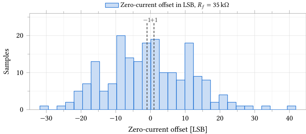
Figure 34.38: Zero-current output offset at R_f = 35\text{ k}\Omega , in nominal 2.441 mV ADC LSB. Mismatch only , 25 °C nominal process, 200 samples, R_{ct} = 10\text{ k}\Omega electrode. The limit shown is the \pm 1 LSB entered on the test in Assembler – comparable in kind across the four gain taps but mechanically harder to meet as R_f rises, since the underlying offset is closer to gain-independent in current (Table 34.53). The converter’s measured step is 1.591 mV, not the nominal 2.441 mV (Table 34.58); multiply the axis and the limit by 1.535 to read them as converter codes. Statistics are in Table 34.53.
