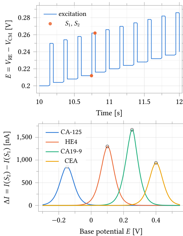
Figure 34.5: Differential-pulse voltammetry through the rev-2 channel, four-reporter immunoassay panel, one electrode parameter set per reporter ( R_f = 560 \text{ k}\Omega , C_{dl} = 200 \text{ nF} , 37^\circ\text{C} ). Top: a 2 s excerpt of the excitation (4 mV treads, 50 mV / 50 ms pulses at a 200 ms period, every level quantised to 152.6 \mu\text{V} ), with the two current-sampling instants 5 ms before each edge. Bottom: the differential current over the full -0.300 \text{ V} to 0.548 \text{ V} scan (213 steps, 42.6 s); peak potential separates the reporters, peak height carries concentration (circles mark the apexes: 855 nA, 1300 nA, 1666 nA and 938 nA). Reporter kinetics as in the cyclic-voltammetry runs; the panel differs from Figure 34.4 in readout, gain tap and reporter set. The 152.6 \mu\text{V} step is finer than the 610.35 \mu\text{V} LSB of the shipped 12-bit reference DAC (Section 34.9), so the apex accuracy read off this panel is a lower bound on the channel's.
