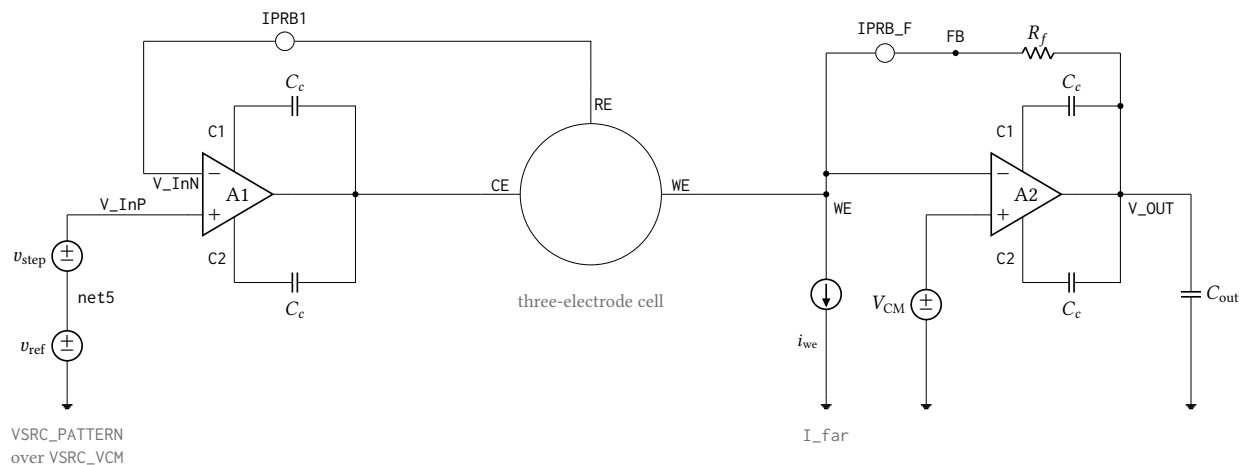
Figure 34.31: The complete rev-2 potentiostat pixel as simulated, tb_anatop_pixel view PotFbTB : control amplifier A1 drives the counter electrode and closes its loop on the reference electrode, while transimpedance amplifier A2 holds the working electrode at V_{CM} and returns the cell current through R_f to V_{OUT} . Both amplifiers are the same anatop_tia_amp_ab class-AB cell, each with its own external compensation capacitors C_c = 500 fF from pins C1/C2 onto its own output; supplies, E_n and the shared local bias generator are omitted. IPRB1 and IPRB_F are 0 V current probes inserted only so that stb can break the control loop and the transimpedance loop respectively – they add no impedance and no offset. I_far injects the accuracy-truth current with positive i_{we} flowing from the working electrode to ground, so v_{out} = V_{CM} + i_{we} \cdot R_f and the measured current is the probe current in IPRB_F ; the opposite source orientation inverts the sign of every accuracy number. Cell elements are R_{ce} = R_u = 1 k \Omega fixed with R_{ct} and C_{dl} swept over the electrode grid, R_f is the programmable feedback resistor (35 k \Omega to 560 k \Omega ), and C_{out} = 5 pF.
