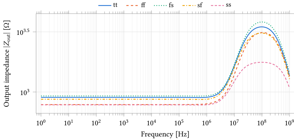
Figure 34.64: Magnitude of the supply block’s output impedance against frequency over five process corners, 27 °C at point 1 and 25 °C at points 2–5. The AC load source carries unit magnitude, so |V_{\text{DDDAC}}| is the impedance in ohms. It is flat at 781 \Omega to 927 \Omega from 1 Hz to 100 kHz and peaks at 1.8 k \Omega to 3.8 k \Omega near 100 MHz. This is the small-signal impedance at zero load; the large-signal chord over the 0 \mu\text{A} to 100 \mu\text{A} sweep is 18 % to 51 % higher (Table 34.76).
