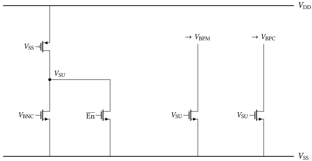
Figure 34.8: Start-up branch. A gate-grounded, permanently-on weak PMOS pulls V_{SU} up at power-on; while V_{SU} is high it drags V_{BPM} and V_{BPC} down, forcing current into the core and breaking the degenerate zero-current state. Once the core is running, the rising V_{BNC} turns on the left NMOS and collapses V_{SU} , so the branch draws no static current in normal operation, the behaviour visible in the power-up transient of Figure 34.16. A second device holds V_{SU} low whenever the cell is disabled.
