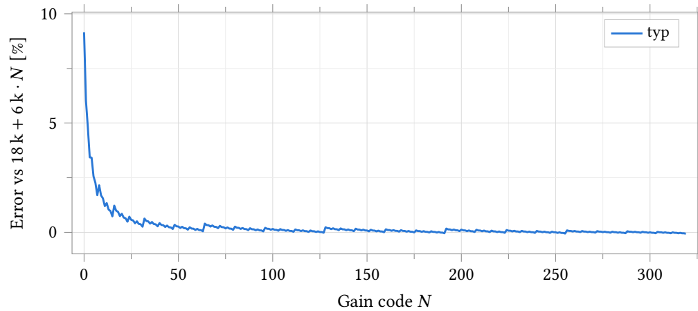
Figure 34.48: Typical-corner deviation from the ideal code law. The +9.2 % at N = 0 is the series resistance of the ten closed bypass switches (1.65 k \Omega , about 165 \Omega each), which decays as 1/R once real ladder segments dominate; by N = 319 the error is -0.063 %. The ripple is the carry structure: at each binary carry and at each thermometer seam the set of closed switches changes, so the R_{on} term steps while the ladder term is exact.
