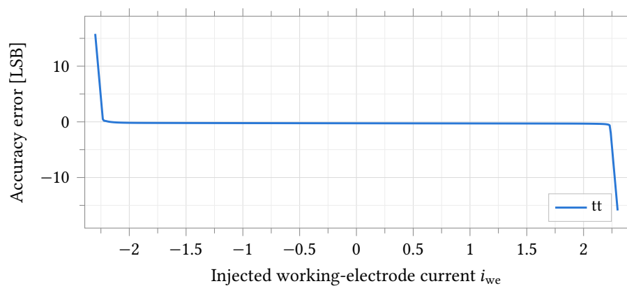
Figure 34.33: Accuracy error at the operational max-gain point, R_f = 560\text{ k}\Omega into R_{ct} = 1\text{ M}\Omega , typical process point, 37^\circ\text{C} . The truth current sweep is \pm 2.3\text{ }\mu\text{A} , just beyond the 2.06\text{ }\mu\text{A} full-scale current at this gain tap; the crossing at zero is smooth, with no kink, over the full swept range shown. The error axis is referred to the nominal 2.441\text{ mV} step; the converter's measured step is 1.591\text{ mV} (Table 34.58), so multiply by 1.535 to read it as converter codes.
