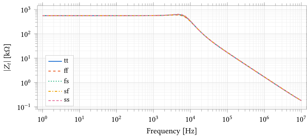
Figure 34.23: Closed-loop transimpedance magnitude over five process corners, conditions as Figure 34.24. The AC stimulus is a 1 \text{ A} current into the working electrode, so the ordinate is transimpedance directly. The feedback resistor is an ideal element here rather than the 16-tap string, which is why the corners separate only near the band edge; the numbers are in Table 34.26. The corner separation drawn here is a lower bound: the corner set holds the passive model rows at typical (pinned-passive caveat, page 295).
