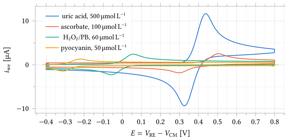
Figure 34.4: Voltammograms of the four-analyte panel through the rev-2 channel, one electrode parameter set per channel, from the cyclic-voltammetry Maestro corner run of Section 34.2 ( 2 \text{ V s}^{-1} , R_f = 35 \text{ k}\Omega , conditions of the in-loop run above). Peak potential identifies the analyte and peak height its concentration; each trace is one full cycle started at that analyte's non-faradaic vertex. E^{0'} and concentrations are literature-anchored; k^0 is fitted (no measured value exists on carbon for any of the four), and reversal peaks appear for the chemically irreversible couples because following chemistry is not modelled. The two cathodic markers span -1.4 \mu\text{A} to -2.4 \mu\text{A} , unmeasurable by the unidirectional rev-1 front end.
