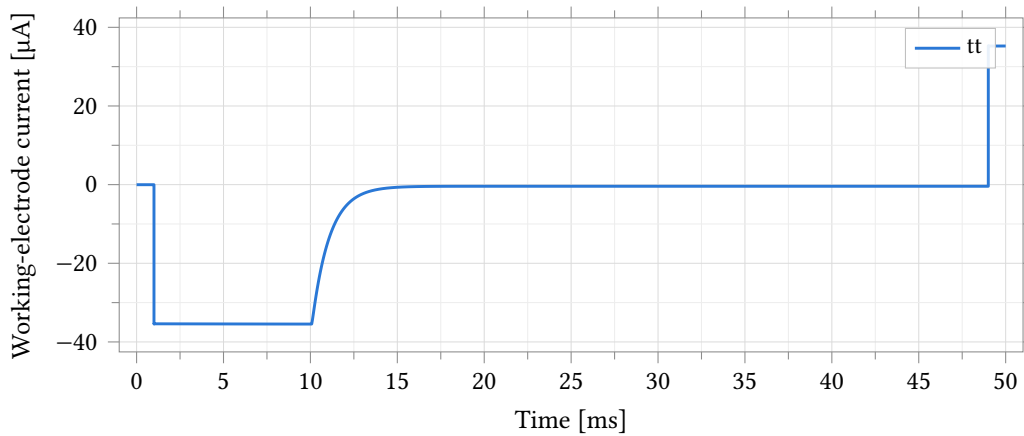
Figure 34.37: Step response of the working-electrode current to a 400 mV step in the commanded reference potential, typical process point, 37 °C, R_f = 35 \text{ k}\Omega , R_{ct} = 1 \text{ M}\Omega electrode, 1 \mu\text{s} edge. The transient overshoots and briefly rails against the loop’s slew-limited edges immediately after the step – by design, the bench exercises the edge rather than a settled operating condition – before settling to the value set by the cell impedance.
