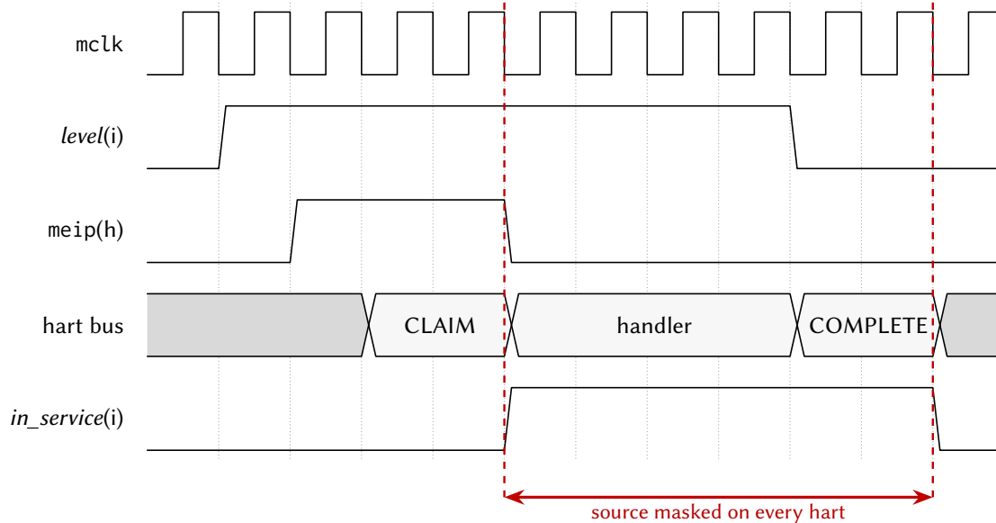
Figure 33.2: Claim/complete delivery of one peripheral interrupt.
