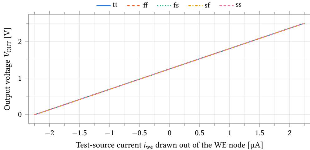
Figure 45: Output voltage against the swept test-source current over the five corners, at R_f = 560 kΩ with the electrode held at v_{cm} = 1.25 V. The bench source draws current out of the WE node, so i_{we} = -I_{WE} against Equation (1) and the slope is +R_f . The corners overlay to the line width because that slope is the feedback resistor, ideal in this bench.
