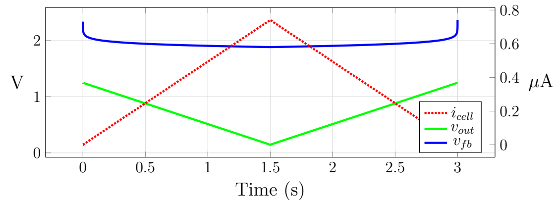
Electrochemical Response to CV Excitation
