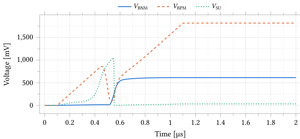
Figure 34: Power-up transient at the typical corner. The start-up node V_{SU} pulls the core out of its zero-current state, after which both mirror rails settle to their steady-state values.
