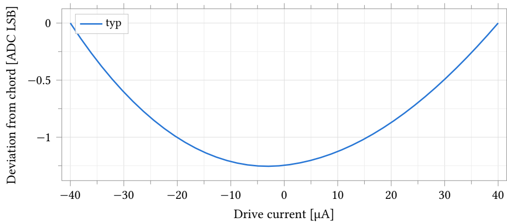
Figure 67: Drive nonlinearity of the bottom code ( N = 0 , R \approx 19.6 \text{ k}\Omega ): voltage deviation from the endpoint chord over \pm 90\% of full scale ( \pm 40 \mu\text{A} ), typical corner, expressed in 1.592 \text{ mV ADC LSB} . All ten bypass gates are closed at this code and carry the full signal current; their on-resistance rises with the terminal's excursion from V_{\text{CM}} , so the chord — pinned at the sweep endpoints where that excursion is largest — overestimates the mid-range voltage by up to 1.25 \text{ LSB} , and the deviation is bowl-shaped with a slight skew from the gates' voltage asymmetry. The same measurement at N = 63 and N = 319 , where the ladder dominates and current is 20\text{--}100\times smaller, stays below 0.004 \text{ LSB} and is tabulated, not plotted.
