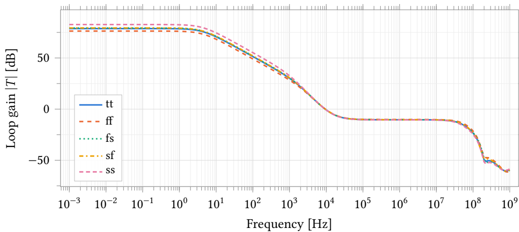
Figure 42: Transimpedance loop gain over five process corners, measured through a probe in series with the feedback network (Figure 40). R_f = 560\text{ k}\Omega , C_f = 22\text{ pF} , C_L = 5\text{ pF} , C_c = 500\text{ fF} , BiasAdj = 37, 2.5 V, Randles electrode with R_s = 100\text{ }\Omega , R_{ct} = 1\text{ M}\Omega , C_{dl} = 100\text{ nF} . tt is at 37^\circ\text{C} , the four skew corners at 25^\circ\text{C} . This is the loop around the amplifier, the feedback network and the electrode together, not the amplifier's own gain; the two are tabulated separately in Table 37 and Table 24.
