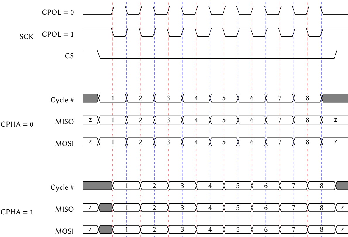
Figure 86: SPI Timing Diagram
