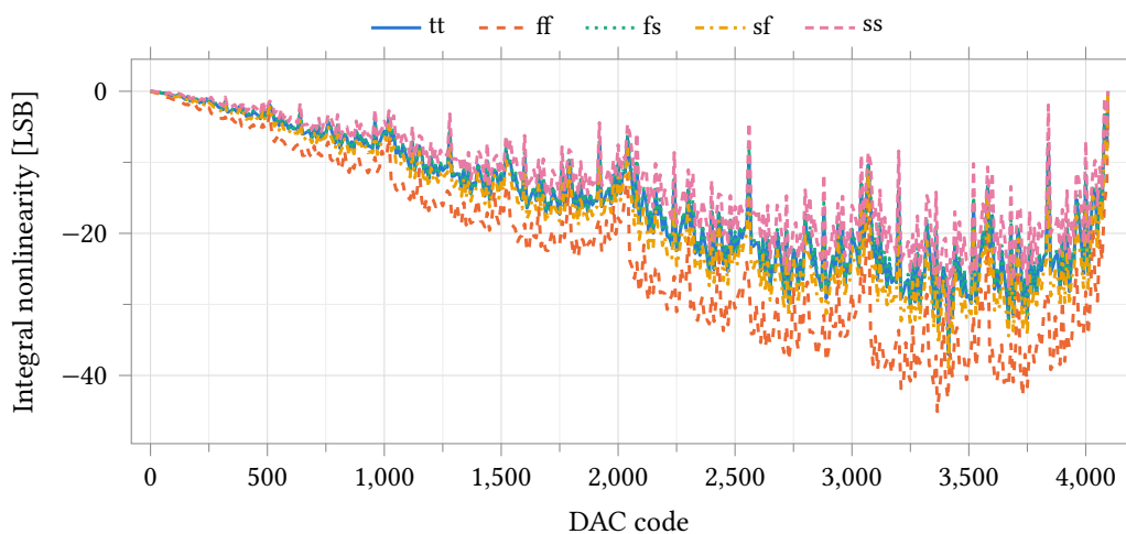
Figure 74: Integral nonlinearity against code over five process corners with the ladder referenced to V_{ddDac} from the supply block, zero external load, 25 °C. Endpoint-line INL as in Figure 70; the vertical scale is tens of LSB, not tenths. The bow reaches -37.1 LSB at tt (code 3413) and -45.1 LSB at ff (code 3365) and tracks the reference droop of Figure 73 scaled by code. Dividing each code's output by the reference measured at that code removes it and leaves 0.43 to 0.45 LSB (Table 76), so the ladder is unchanged from the ideal-rail case.
