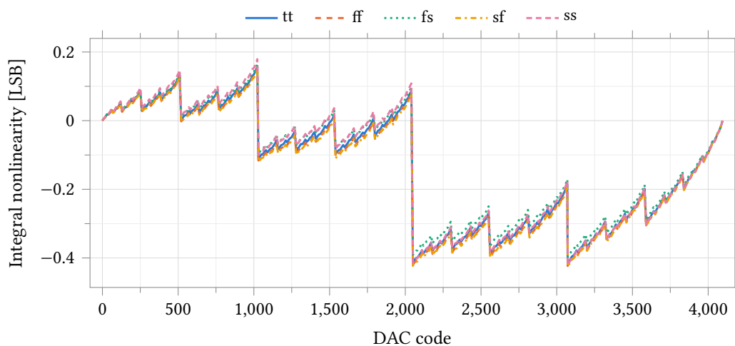
Figure 70: Integral nonlinearity against code over five process corners, ladder on an ideal 2.5 V rail, 25 °C, \text{reltol} = 1 \times 10^{-6} . INL is taken from the endpoint line through each corner's own zero- and full-scale outputs, so it is zero at codes 0 and 4095 by construction. The positive extreme is code 1023, +0.15 to +0.18 LSB; the negative extreme is shared by the major carries at codes 2048 and 3072, which sit within 0.006 LSB of each other at -0.39 to -0.43 LSB at every corner. The code of each extreme is the same at all five corners: the shape is set by the ladder, not by the process. Corner run, no device mismatch — R-2R linearity is a matching property, so this envelope is the systematic term alone.
