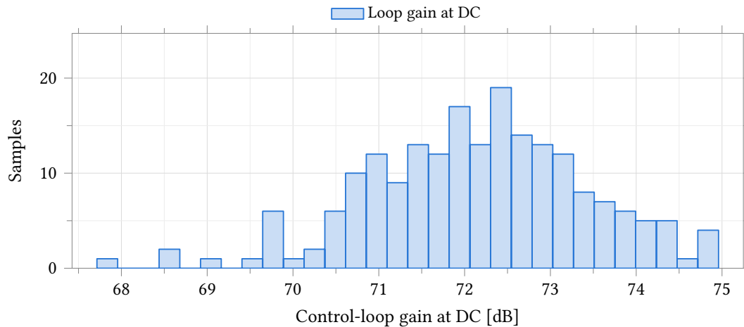
Figure 48: DC gain of the control loop closed around an electrochemical cell. Process and mismatch , 37 °C, 200 samples, cell-drive bench (Figure 46) with a Randles cell of R_{\text{CE}} = 1 k \Omega , R_u = 1 k \Omega , R_{\text{ct}} = 10 k \Omega , C_{\text{dl}} = 1 \mu\text{F} , working electrode at 1.25 V, C_L = 5 pF, C_c = 500 fF, 2.5 V supply. The loop is measured through the reference-electrode sense wire and therefore includes the cell, whose 12 k \Omega loads an open-loop output resistance of about 25 k \Omega and is 10 dB below the unity-feedback gain of Table 30. The spread is 7 dB peak to peak and no sample falls below 67 dB. No limit was entered on this output.
