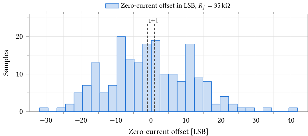
Figure 56: Zero-current output offset at R_f = 35 k \Omega , referred to the 2.441 mV ADC LSB. Mismatch only , 25 °C nominal process, 200 samples, R_{\text{ct}} = 10 k \Omega electrode. The limit shown is the \pm 1 LSB entered on the test in Assembler – comparable in kind across the four gain taps but mechanically harder to meet as R_f rises, since the underlying offset is closer to gain-independent in current (Table 63). Statistics are in Table 63.
