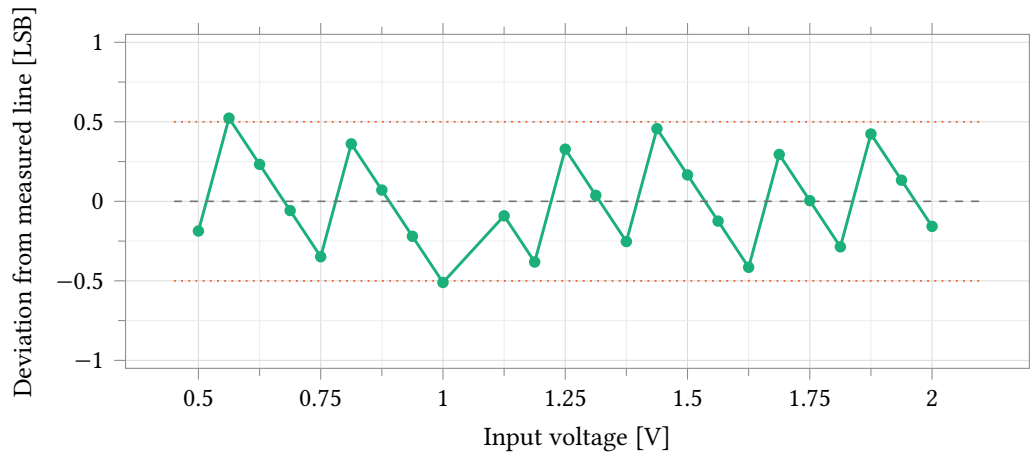
Figure 63: Deviation of each measured code from the converter's own best-fit line, 628.64 codes/V, over a 0.0625 V sweep of the unclipped window. Referred to its own scale rather than the nominal one the converter is straight to 0.523 LSB worst case and 0.294 LSB rms, so the 168 LSB of Figure 61 is gain error alone and carries no linearity information. The worst point sits just outside the \pm 0.5 LSB dotted guides. Twenty-four points 39 codes apart bound the deviation at the sampled inputs; a DNL or INL measurement needs every code and this grid does not provide one. A twenty-fifth point at 1.0625 V is absent because its simulation returned an error.
