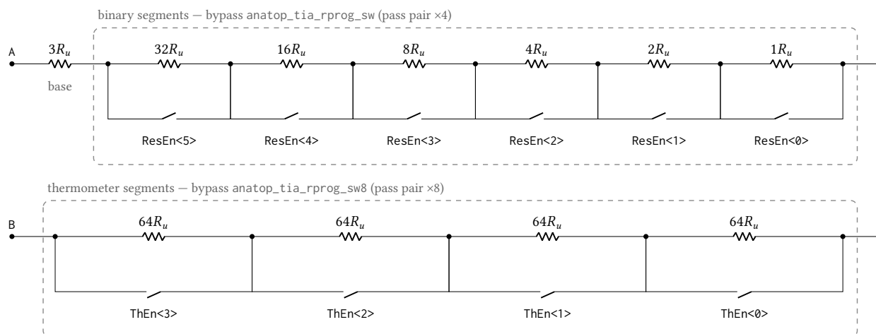
Figure 64: Segment and bypass-switch structure of anatop_tia_rprog , transcribed from the executed spec-run netlist. The unit R_u is one series poly resistor; from terminal A the chain runs through the never-switched three-unit base, the six binary-weighted segments of 32 down to 1 unit, and the four identical 64-unit thermometer segments to terminal B. Each switched segment is shunted by a CMOS transmission gate with a local inverter: the control pin EnBar is the ResEn/ThEn bit itself and drives the PMOS pass gate directly and the NMOS pass gate through the inverter, so a bit at 1 turns both pass devices off and inserts the segment. The pass pair has multiplicity 4 in the binary switch ( _sw ) and 8 in the thermometer switch ( _sw8 ), which halves the thermometer gates' on-resistance where up to six binary gates close at a seam. Three grounded dummy units accompany the 322 active units for matching.
