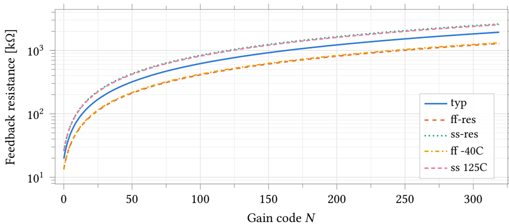
Figure 65: Measured resistance against gain code at all five corners, 500 nA forced through the A–B terminals with B held at V_{CM} = 1.25 V. The law is R = 18 \text{ k}\Omega + 6 \text{ k}\Omega \cdot N with N the binary value of ResEn<5:0> plus 64 per set ThEn<3:0> thermometer bit; every corner is strictly monotonic over all 320 codes, including the four thermometer seams. The corner families move the absolute value by -33 to +35 %, which is the poly sheet-resistance tolerance and must be absorbed by gain calibration, not by code choice.
