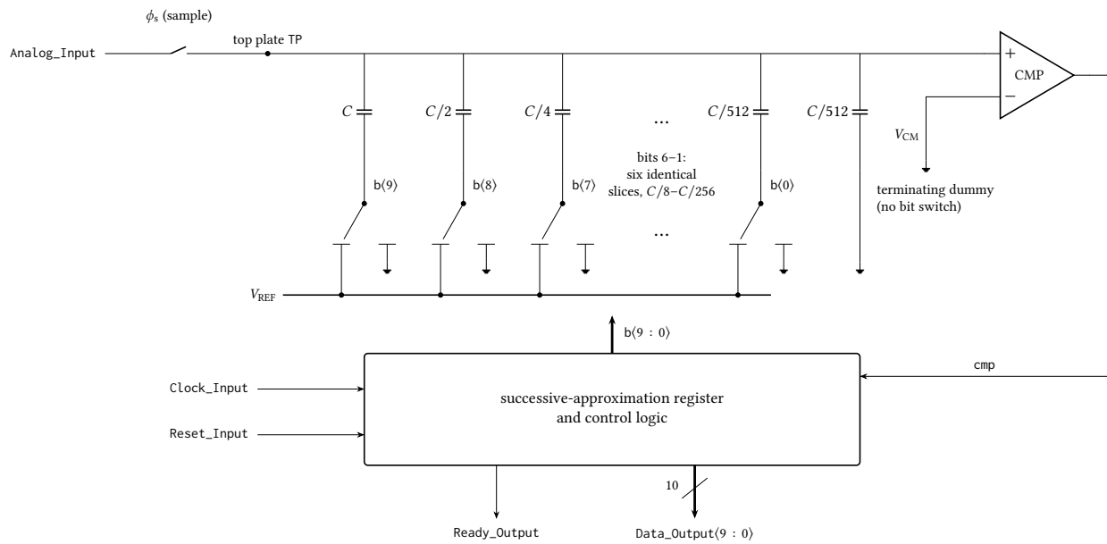
Figure 58: Generic single-ended charge-redistribution SAR ADC, drawn to explain the architecture of the 10-bit converter rather than to reproduce its implemented transistor-level schematic. The input is sampled through \phi_s onto the top plate of a binary-weighted array; the logic then switches each bottom plate from V_{REF} to ground one bit at a time, most significant first, and keeps or discards the trial from the comparator decision, so the conversion takes ten comparator cycles and the top plate converges to V_{CM} . Bits 6–1 are elided: six further slices identical to those drawn sit between C/4 and C/512 , and the terminating dummy C/512 carries no bit switch, which makes the total array 2C and the LSB weight C/512 . Only the external port names are those of the implemented block; the sampling network, comparator topology, clock generation and reset behaviour are representative, and no device dimensions are stated.
