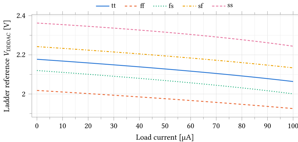
Figure 79: V_{\text{DDDAC}} against external load current over five process corners, supply block alone, 27 °C at point 1 and 25 °C at points 2–5, ADE default tolerances. There is no feedback loop around the output, so the slope is the block’s own output resistance and the reference falls 92.7 mV to 119.3 mV across the 0 \mu\text{A} to 100 \mu\text{A} sweep. The curve steepens with load, which is why the chord in Table 81 exceeds the small-signal |Z_{\text{out}}| of Table 85. This sweep is an external load only: the ladder is not connected on this bench, and its own code-dependent draw is Figure 73.
