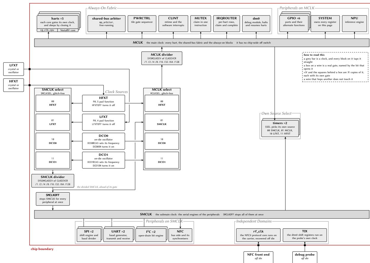
Figure 95: The MCU clock system, generated from this configuration. The layout is a mirror: the sources stand in one column, in the order SMCLKSEL enumerates them, the SMCLK chain runs left out of that column and down into its own bar, and the MCLK chain runs right out of it and up into its own, so every source leg is a straight horizontal at its own row. Each select box prints every code it has, with the name of what that code picks, and those rows are built from the register model itself rather than drawn by hand. One code is not a source: MCLKSEL 01 takes SMCLK, tapped after the SMCLK divider and before the SMCLKOFF gate, which is why stopping SMCLK never stops MCLK; it is the one wire in the drawing that has to leave its row, and it hops the legs it crosses rather than touching them. A source that either select is using stays enabled whatever its own bit says. Every block on a bar taps it straight up or straight down; the sleep gate is drawn where the hardware puts it, inside each core, so the stack of five harts is a stack of five gates. A block with a select of its own names every code it has and taps the two bars it can reach, so the crystal sources it may also pick are named in its box rather than drawn as two more wires across the page. The blocks under Independent Domains are on neither bar: they are clocked from outside this tree entirely, and SYSCLKCR does not reach them. The register interface of every peripheral is clocked from MCLK even where its engine runs on SMCLK, which is why a peripheral stays readable with SMCLK stopped.
