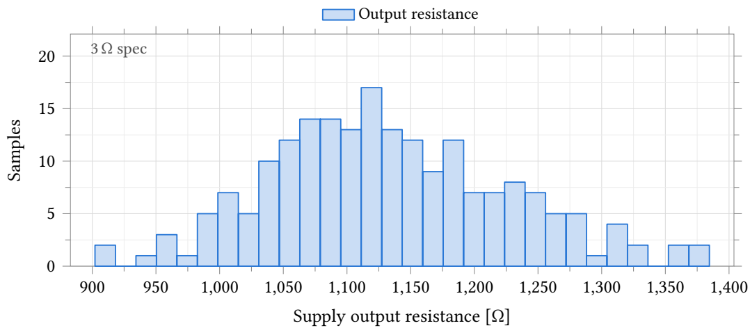
Figure 80: Output resistance of the DAC supply block, taken as the chord \Delta V / \Delta I over a 0 \mu A to 100 \mu A load sweep on VddDac. Process and mismatch , castalia_pm_25, 200 samples, 27 °C. The 3 \Omega limit entered on the test is two orders of magnitude below the data and is annotated at the left axis edge rather than drawn; no sample meets it. This is not a second defect: the reference movement of Figure 78 is this impedance multiplied by the ladder’s own code-dependent reference current.
