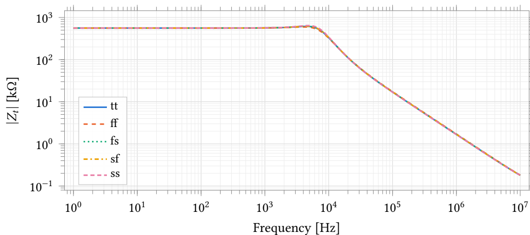
Figure 41: Closed-loop transimpedance magnitude over five process corners, conditions as Figure 42. The AC stimulus is a 1 A current into the working electrode, so the ordinate is transimpedance directly. The feedback resistor is an ideal element here rather than the 16-tap string, which is why the corners separate only near the band edge; the numbers are in Table 36.
