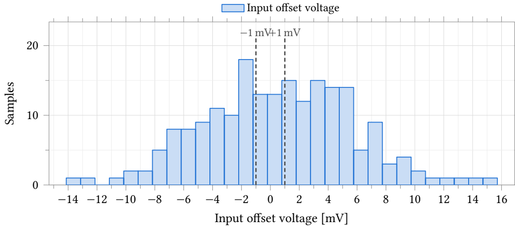
Figure 38: Input offset voltage of the amplifier. Process and mismatch , 37^\circ\text{C} , 200 samples, 2.5 V supply, C_L = 5\ \text{pF} , C_c = 500\ \text{fF} , a 5\ \text{pF} load, differential input swept about mid-supply. The distribution is symmetric about 0.58\ \text{mV} , so the systematic term of Table 26 is small against the random one, and the \pm 1\ \text{mV} rules are the limits entered on the test; 24 of 200 samples fall inside them. Statistics are in Table 29.
