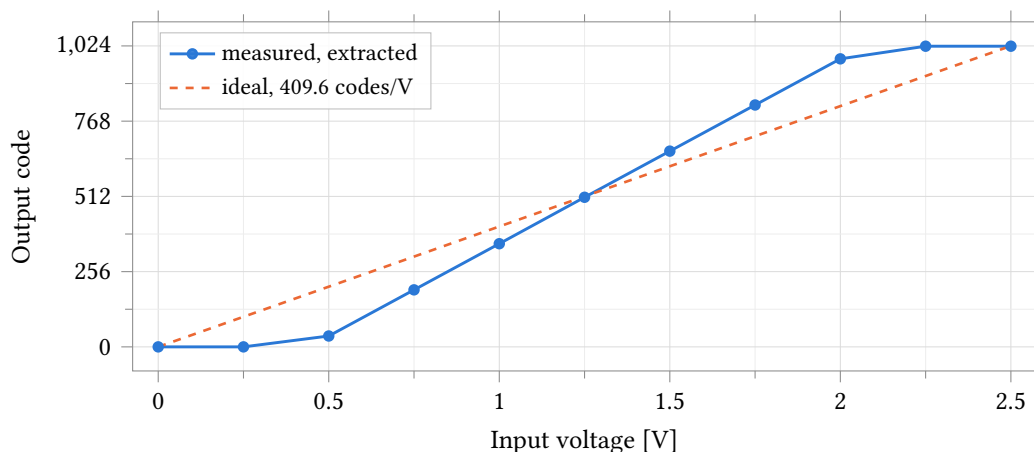
Figure 60: Output code against input voltage for the extracted anatop_pixel_adc , nominal corner, 37 °C, 2.5 V analog and 1.0 V digital supplies, with the ideal 409.6 codes/V line overlaid. The transfer is monotonic and reaches both code limits, but its slope is 628.64 codes/V – 1.535 times ideal – so the flat segments below 0.44 V and above 2.07 V are the code limits, not the ends of the sweep. Markers are the eleven simulated points; the 0.25 V step is 157 codes, so the curve between them is interpolation and carries no linearity information.
