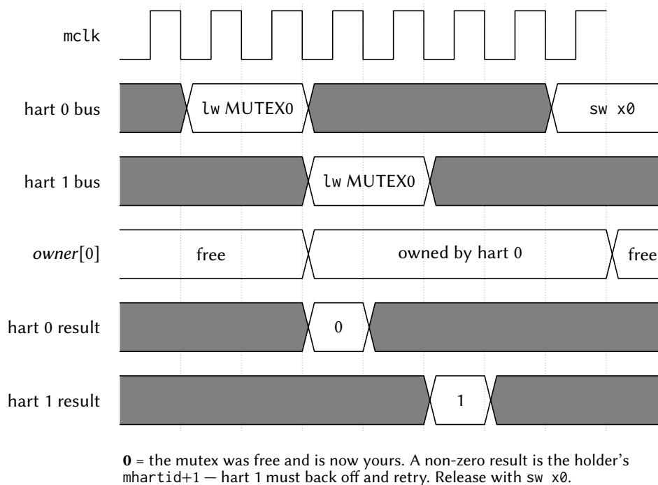
Figure 37: Two harts racing for the same mutex. The arbiter serializes the two claim reads, so the return-old-and-claim happens atomically with no retry loop: hart 0 reads 0 and thereby owns the mutex, and hart 1 reads hart 0's marker and must back off.
