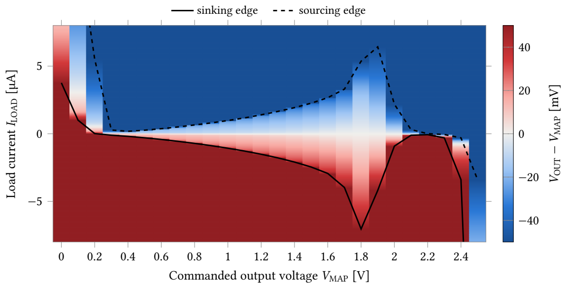
Figure 23: DC drive compliance of the control amplifier, as a map of the unity-gain tracking error over commanded output voltage and load current. Positive I_{LOAD} draws current out of the output, so the amplifier sources ; negative I_{LOAD} injects, so it sinks . The colour scale is clipped at \pm 50 mV, which is the compliance criterion: inside the envelope the error is the smooth I_{LOAD}R_{OUT,CL} gradient, and outside it the output has hit a rail and the error jumps by more than a volt, so everything beyond the envelope saturates to solid colour. The two black curves are the |V_{OUT} - V_{MAP}| = 50 mV edges, interpolated on the 50 nA sweep at each of the 26 commanded voltages; that they land on the boundary of the graded band is a check that the map and the envelope were derived independently. The vertical axis is cropped to \pm 8 \mu\text{A} ; the envelope never exceeds that inside the tracking range. This is the ff corner with typical resistors – see Table 20 and the note below it.
