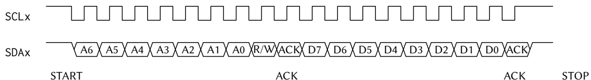
Figure 36: One I2C byte write on the wire: START, the 7-bit address and direction bit, the addressed device's ACK, one data byte, its ACK, then STOP. START and STOP are the two transitions of SDAx that occur while SCLx is high; every data bit is stable across the SCLx high period.
