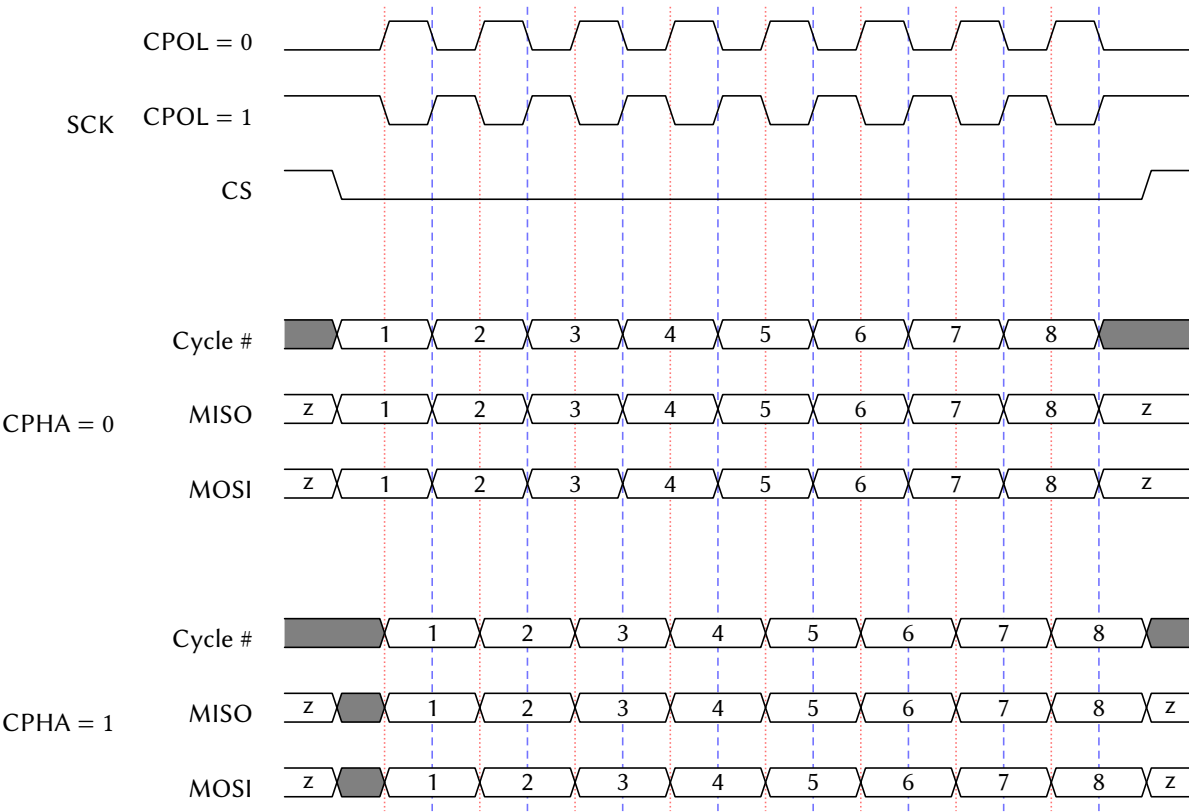
Figure 83: SPI Timing Diagram
