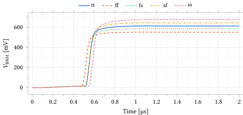
Figure 32: Power-up settling of V_{BNM} over all process corners.
