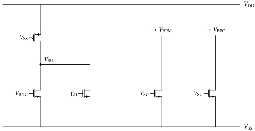
Figure 23: Start-up branch. A gate-grounded, permanently-on weak PMOS pulls V_{SU} up at power-on; while V_{SU} is high it drags V_{BPM} and V_{BPC} down, forcing current into the core and breaking the degenerate zero-current state. Once the core is running, the rising V_{BNC} turns on the left NMOS and collapses V_{SU} , so the branch draws no static current in normal operation, the behaviour visible in the power-up transient of Figure 31. A second device holds V_{SU} low whenever the cell is disabled.
