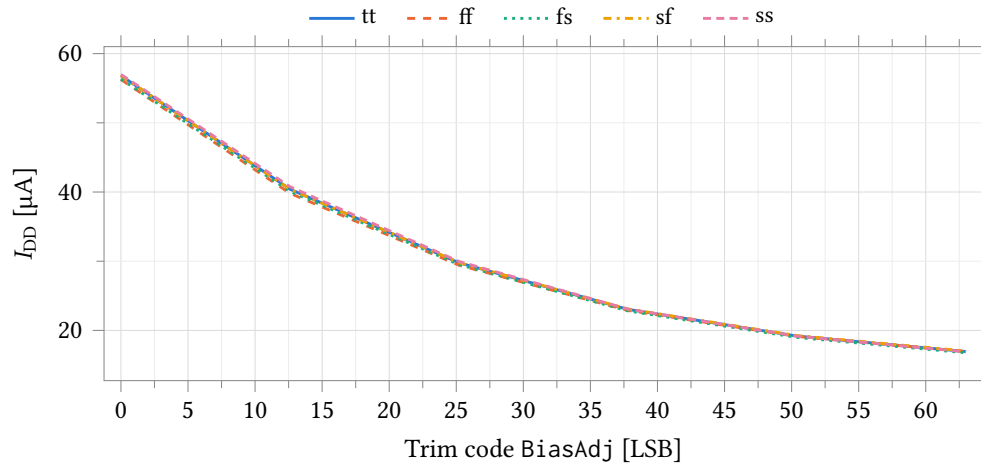
Figure 30: Trim characteristic: quiescent supply current against the BiasAdj word over all process corners, at the same six sampled codes. The current is strongly monotonic in the trim word, falling by a factor of about 3.4 from code 0 to code 63.
