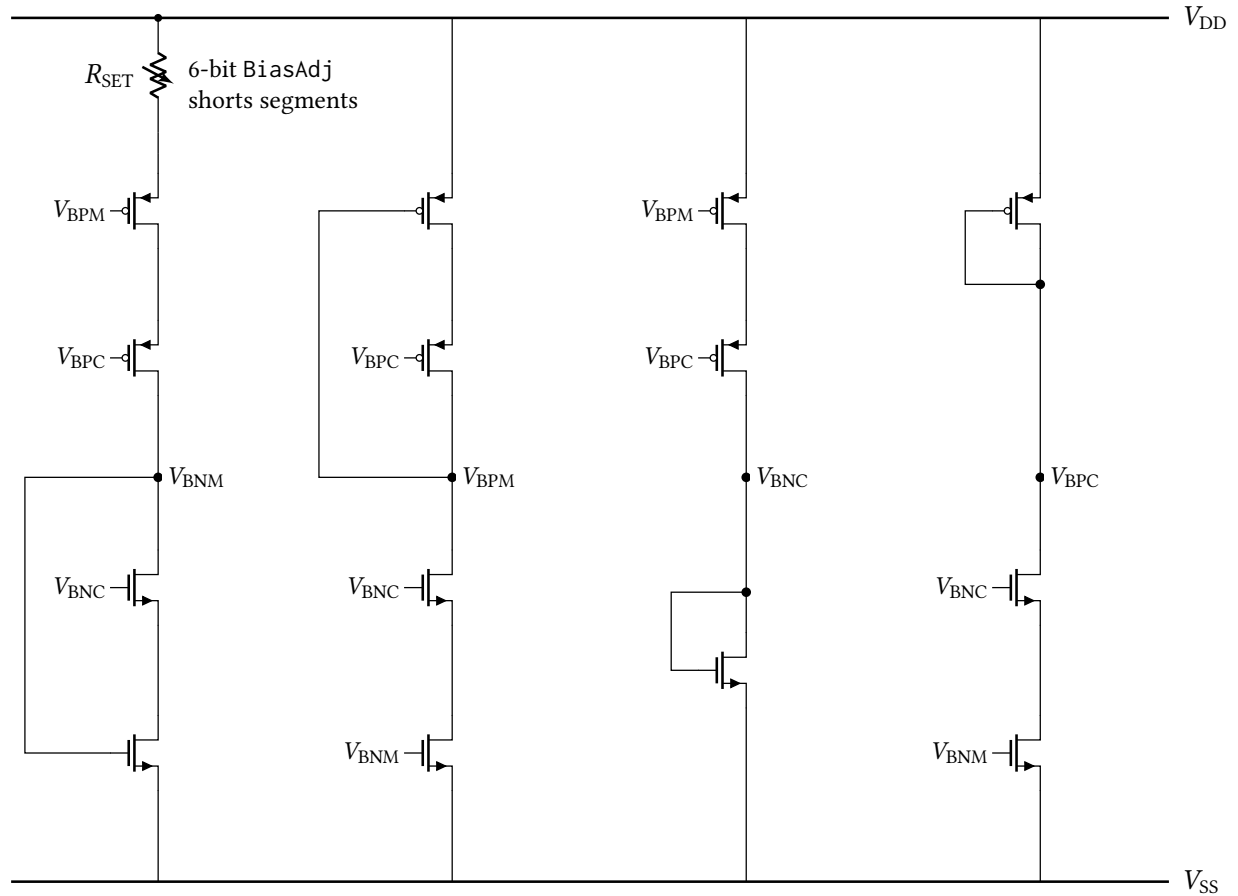
Figure 22: Simplified core of the local wide-swing cascode bias generator, drawn from the anatop_biasgen_local schematic. Four self-biased branches develop the four rails: the reference branch (left) passes the current set by the trimmable resistor R_{SET} , and the remaining branches mirror it to produce V_{BPM} , V_{BNC} and V_{BPC} . Each branch's own self-bias (diode) connection is drawn, from the rail it generates back to the gate it drives in the same branch; the cross-branch gate connections are identified by net name rather than drawn as buses. The enable switches, the decoupling capacitors on each rail and the individual segments of the resistor string are omitted for clarity.
