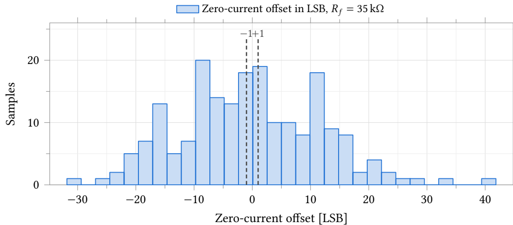
Figure 53: Zero-current output offset at R_f = 35\ \text{k}\Omega , referred to the 2.441\ \text{mV} ADC LSB. Mismatch only , 25^\circ\text{C} nominal process, 200 samples, R_{\text{ct}} = 10\ \text{k}\Omega electrode. The limit shown is the \pm 1\ \text{LSB} entered on the test in Assembler – comparable in kind across the four gain taps but mechanically harder to meet as R_f rises, since the underlying offset is closer to gain-independent in current (Table 63). Statistics are in Table 63.
