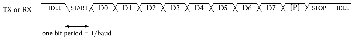
Figure 87: UART Data Frame Timing Diagram
