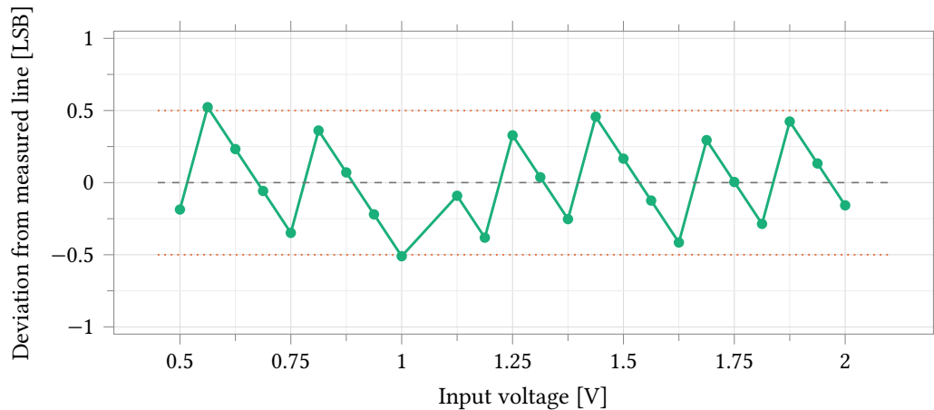
Figure 60: Deviation of each measured code from the converter's own best-fit line, 628.64 codes/V, over a 0.0625 V sweep of the unclipped window. Referred to its own scale rather than the nominal one the converter is straight to 0.523 LSB worst case and 0.294 LSB rms, so the 168 LSB of Figure 58 is gain error alone and carries no linearity information. The worst point sits just outside the \pm 0.5 LSB dotted guides. Twenty-four points 39 codes apart bound the deviation at the sampled inputs; a DNL or INL measurement needs every code and this grid does not provide one. A twenty-fifth point at 1.0625 V is absent because its simulation returned an error.
