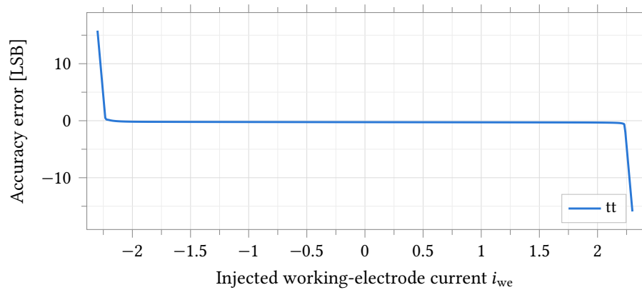
Figure 48: Accuracy error at the operational max-gain point, R_f = 560\text{ k}\Omega into R_{ct} = 1\text{ M}\Omega , typical process point, 37\text{ }^\circ\text{C} . The truth current sweep is \pm 2.3\text{ }\mu\text{A} , just beyond the 2.06\text{ }\mu\text{A} full-scale current at this gain tap; the crossing at zero is smooth, with no kink, over the full swept range shown.
