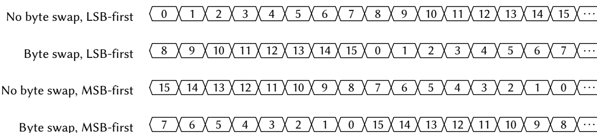
Figure 85: SPI Bit Ordering (16-bit transfer)
