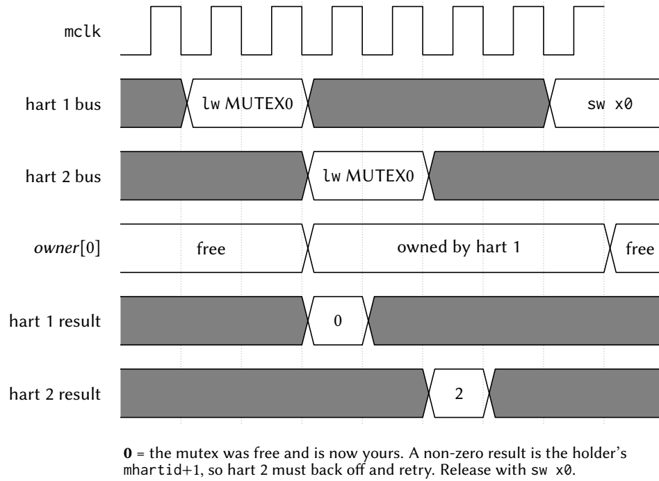
Figure 96: Two harts racing for the same mutex. The arbiter serializes the two claim reads, so the return-old-and-claim happens atomically with no retry loop: the hart the arbiter serves first reads 0 and thereby owns the mutex, and the other reads the winner's marker (mhartid + 1) and must back off.
