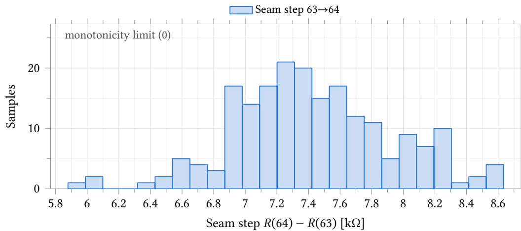
Figure 65: Per-sample step across the first thermometer seam (code 63 to 64: one 64-unit segment switches in while all six binary segments switch out), the code transition most exposed to mismatch. Mismatch only , model section castalia_pm_25 , nominal process, 200 samples, seed 12345, low-discrepancy sampling, 25 °C. Mean 7.42 k \Omega , \sigma = 504 \Omega , worst sample 5.88 k \Omega – 14.7\sigma above the monotonicity limit at zero, so no realistic mismatch closes the seam.
