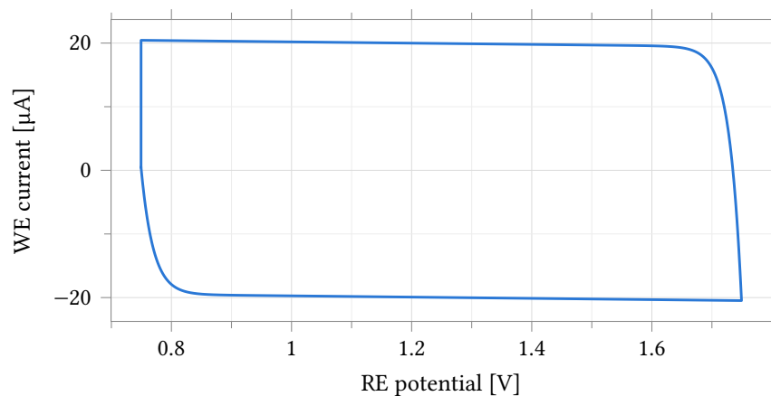
Figure 50: Working-electrode current against commanded reference-electrode potential over one triangular voltammetry sweep, typical process point, 37^\circ\text{C} , R_f = 35\text{ k}\Omega , R_{ct} = 1\text{ M}\Omega electrode. The trace is an ellipse-like loop rather than a single-valued curve because the double-layer capacitance C_{dl} carries a current proportional to dv_{re}/dt in addition to the resistive charge-transfer current; the two straight sweep segments (RE potential linear in time, Figure 51) are why the loop closes into two nearly-parallel branches rather than a smooth curve. The current stays unclipped over the whole sweep (Table 61).
