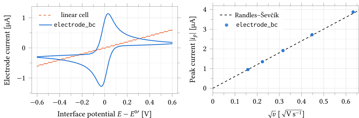
Figure 21: Standalone validation of electrode_bc against closed-form voltammetry, ideal potential source, model defaults of Table 13 with R_s = 500 \Omega and C_{\text{dl}} = 0.2 \mu\text{F} in series and in parallel respectively, 25^\circ\text{C} . Left: current against interface potential over a \pm 0.6 \text{ V} triangular sweep at 50 \text{ mV s}^{-1} , second cycle, for the nonlinear model (solid) and for the linear cell of Section 8.1 driven identically (dashed, R_{\text{ct}} = 1 \text{ M}\Omega ); the linear response is a ramp with its extrema pinned at the switching potentials — its C_{\text{dl}} box is only 20 \text{ nA} wide at this scan rate and invisible here — while the nonlinear one peaks 30 \text{ mV} either side of E^{0'} and decays afterwards. Right: peak cathodic current of the first scan against \sqrt{v} over 25 \text{ mV s}^{-1} to 400 \text{ mV s}^{-1} , against the Randles–Ševčík line, of slope 6.015 \mu\text{A} per \sqrt{\text{V s}^{-1}} ; the two panels use different cycles because Randles–Ševčík describes the first scan into an undepleted bulk, while the second cycle is the repeatable steady response and sits 3 % to 5 % below it. Numbers in Table 14.
