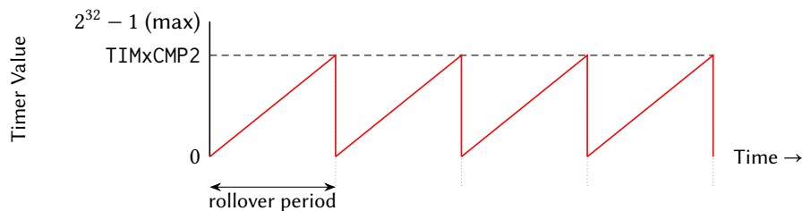
Figure 89: Timer Rollover Operation
