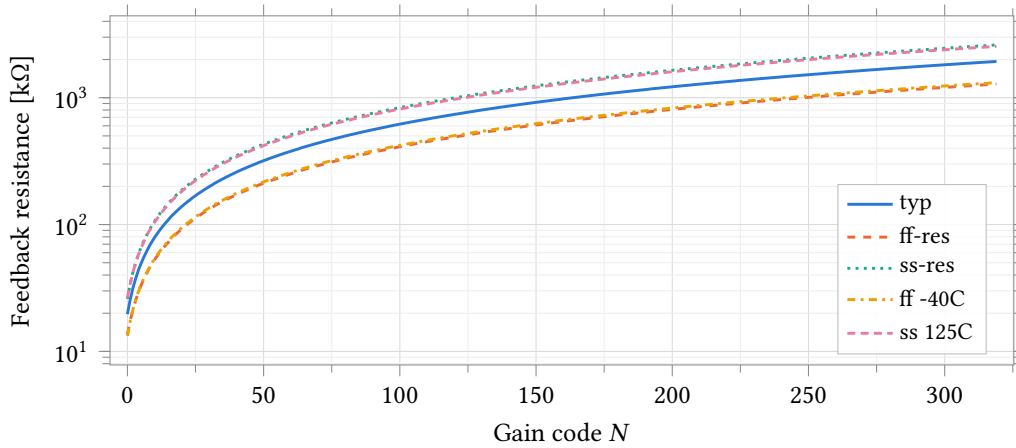
Figure 62: Measured resistance against gain code at all five corners, 500 nA forced through the A–B terminals with B held at V_{CM} = 1.25 V. The law is R = 18 \text{ k}\Omega + 6 \text{ k}\Omega \cdot N with N the binary value of ResEn<5:0> plus 64 per set ThEn<3:0> thermometer bit; every corner is strictly monotonic over all 320 codes, including the four thermometer seams. The corner families move the absolute value by -33 to +35 %, which is the poly sheet-resistance tolerance and must be absorbed by gain calibration, not by code choice.
