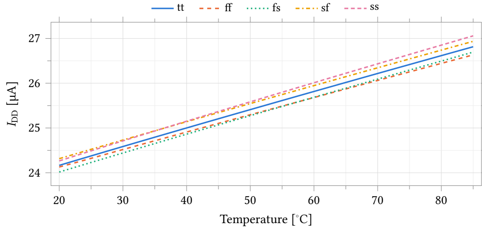
Figure 26: Quiescent supply current of the bias generator against temperature over all process corners.
