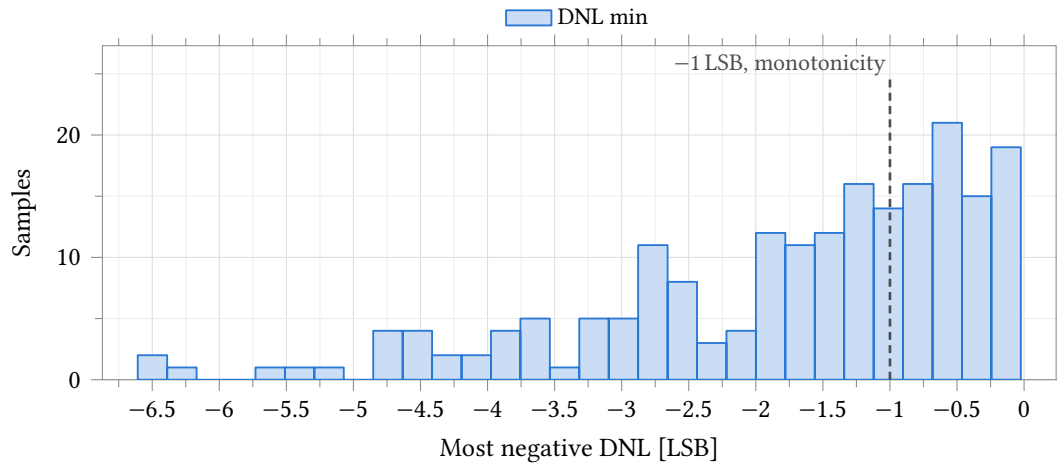
Figure 74: Worst negative differential nonlinearity, same bench, samples and conditions as Figure 73. The dashed rule at -1 LSB is the monotonicity limit entered on the test: 80 of 200 samples clear it, so 40 % of channels are monotonic and 0.40^4 = 2.6 % of four-channel chips are monotonic on all four. The distribution is left-skewed (skew -1.11 ) with a tail to -6.608 LSB, so the median -1.318 LSB and the percentiles of Table 77 describe it and mean \pm 3\sigma does not.
