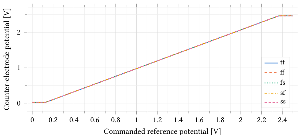
Figure 44: Counter-electrode potential against commanded reference potential over five process corners, cell-drive bench (Figure 43). The amplifier drives a Randles cell with R_{CE} = 1\text{ k}\Omega , R_u = 1\text{ k}\Omega , R_{ct} = 10\text{ k}\Omega , C_{dl} = 1\text{ }\mu\text{F} with the working electrode held at 1.25 V, C_L = 5\text{ pF} , C_c = 500\text{ fF} , 2.5 V supply; the typical point is at 37 °C and the four skew corners at 25 °C. The central segment rises with slope 12/11, the divider between the 1 k \Omega counter-electrode branch and the 11 k \Omega remainder of the cell; the flat ends are the amplifier against its rails, and their heights are the compliance limits tabulated in Table 46. Over the whole central segment the cell current is set by the cell resistance and the commanded potential, not by the amplifier.
