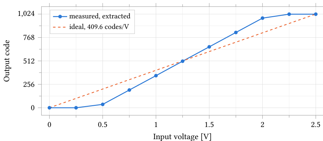
Figure 57: Output code against input voltage for the extracted anatop_pixel_adc , nominal corner, 37 °C, 2.5 V analog and 1.0 V digital supplies, with the ideal 409.6 codes/V line overlaid. The transfer is monotonic and reaches both code limits, but its slope is 628.64 codes/V – 1.535 times ideal – so the flat segments below 0.44 V and above 2.07 V are the code limits, not the ends of the sweep. Markers are the eleven simulated points; the 0.25 V step is 157 codes, so the curve between them is interpolation and carries no linearity information.
