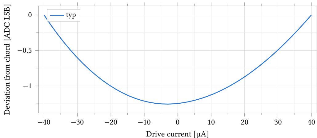
Figure 64: Drive nonlinearity of the bottom code ( N = 0 , R \approx 19.6 k \Omega ): voltage deviation from the endpoint chord over \pm 90 % of full scale ( \pm 40 \mu A), typical corner, expressed in 1.592 mV ADC LSB. All ten bypass gates are closed at this code and carry the full signal current; their on-resistance rises with the terminal's excursion from V_{CM} , so the chord — pinned at the sweep endpoints where that excursion is largest — overestimates the mid-range voltage by up to 1.25 LSB, and the deviation is bowl-shaped with a slight skew from the gates' voltage asymmetry. The same measurement at N = 63 and N = 319 , where the ladder dominates and current is 20–100 \times smaller, stays below 0.004 LSB and is tabulated, not plotted.
