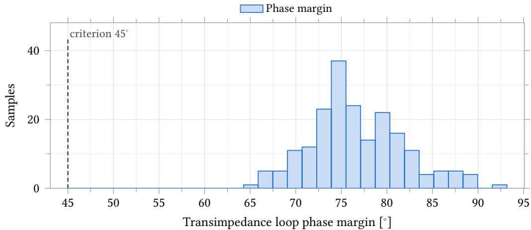
Figure 41: Phase margin of the transimpedance loop, conditions as Figure 40. The loop is measured through the feedback probe of Figure 37 and includes the amplifier, the feedback network and the Randles electrode ( R_s = 100 \Omega , R_{ct} = 1 \text{ M}\Omega , C_{dl} = 100 \text{ nF} ). All 200 samples clear the 45^\circ criterion, minimum 64.7^\circ . The distribution is right-skewed, so percentiles and the extreme sample are quoted in Table 41 rather than \pm 3\sigma .
