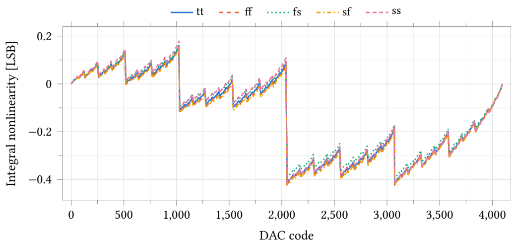
Figure 67: Integral nonlinearity against code over five process corners, ladder on an ideal 2.5 V rail, 25^\circ\text{C} , \text{reltol} = 1 \times 10^{-6} . INL is taken from the endpoint line through each corner's own zero- and full-scale outputs, so it is zero at codes 0 and 4095 by construction. The positive extreme is code 1023, +0.15 to +0.18 LSB; the negative extreme is shared by the major carries at codes 2048 and 3072, which sit within 0.006 LSB of each other at -0.39 to -0.43 LSB at every corner. The code of each extreme is the same at all five corners: the shape is set by the ladder, not by the process. Corner run, no device mismatch — R - 2R linearity is a matching property, so this envelope is the systematic term alone.
