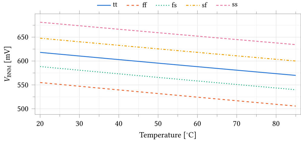
Figure 25: NMOS mirror bias V_{\text{BNM}} against temperature over all process corners.
