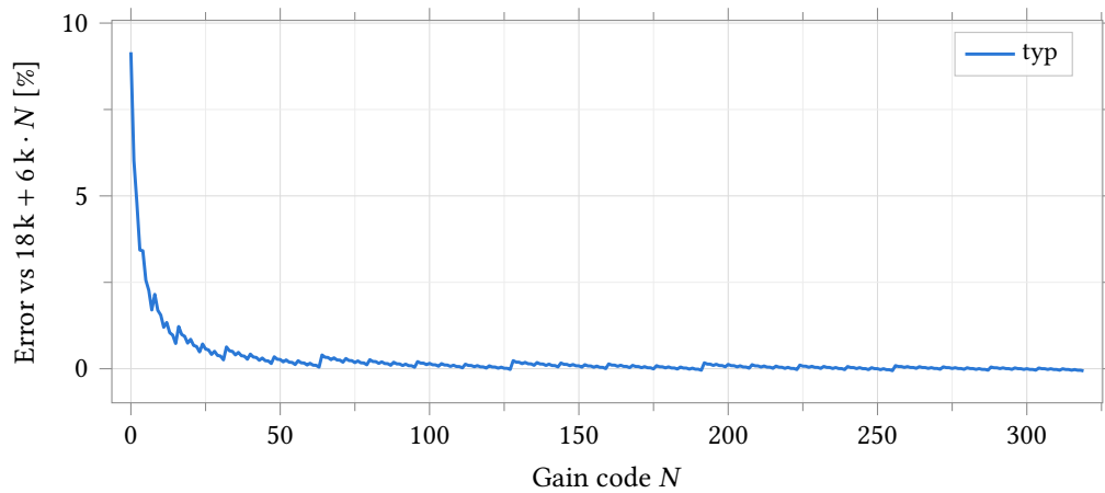
Figure 63: Typical-corner deviation from the ideal code law. The +9.2 % at N = 0 is the series resistance of the ten closed bypass switches (1.65 k \Omega , about 165 \Omega each), which decays as 1/R once real ladder segments dominate; by N = 319 the error is -0.063 %. The ripple is the carry structure: at each binary carry and at each thermometer seam the set of closed switches changes, so the R_{on} term steps while the ladder term is exact.
