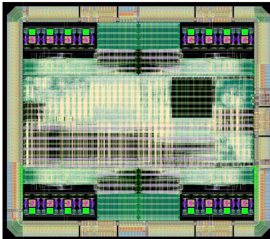
Chip Layout, 2.25 \times 2.00 mm
