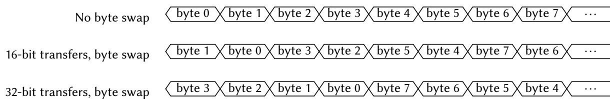
Figure 41: SPI Byte Ordering
