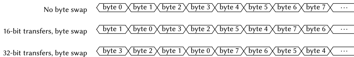
Figure 26: SPI Byte Ordering
