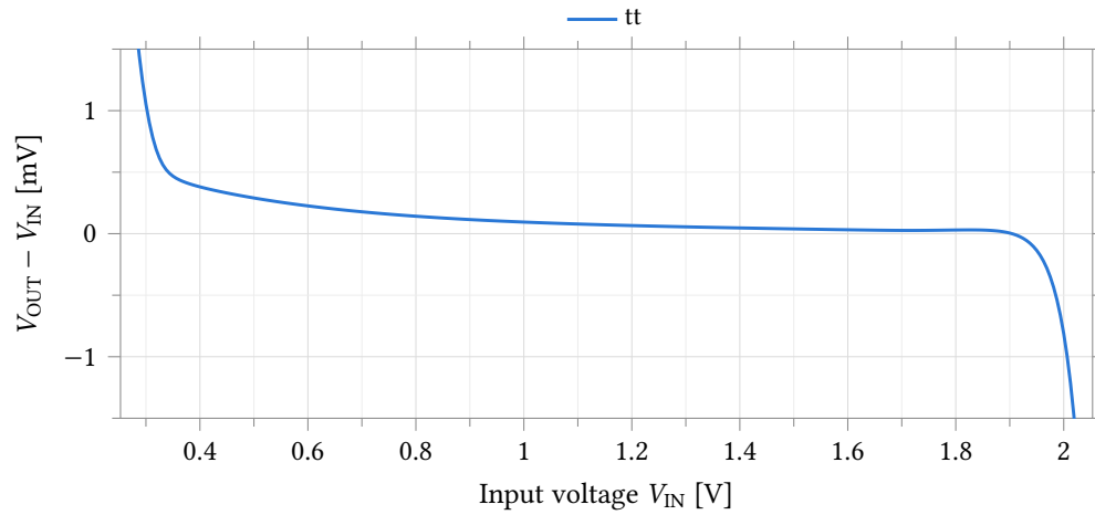
Figure 19: Unity-gain tracking error against input voltage. Inside the window 0.30 V to 2.01 V the error stays under 1 mV, passing through 61 \mu V at mid-supply; the curve leaves the frame at both ends, where the PMOS tail runs out of headroom near the supply and the output stage reaches its low limit near v_{ss} !. The vertical scale is clipped to \pm 1.5 mV so the in-range behaviour is visible at all – the error reaches 97 mV at 0 V and -382 mV at 2.5 V.
