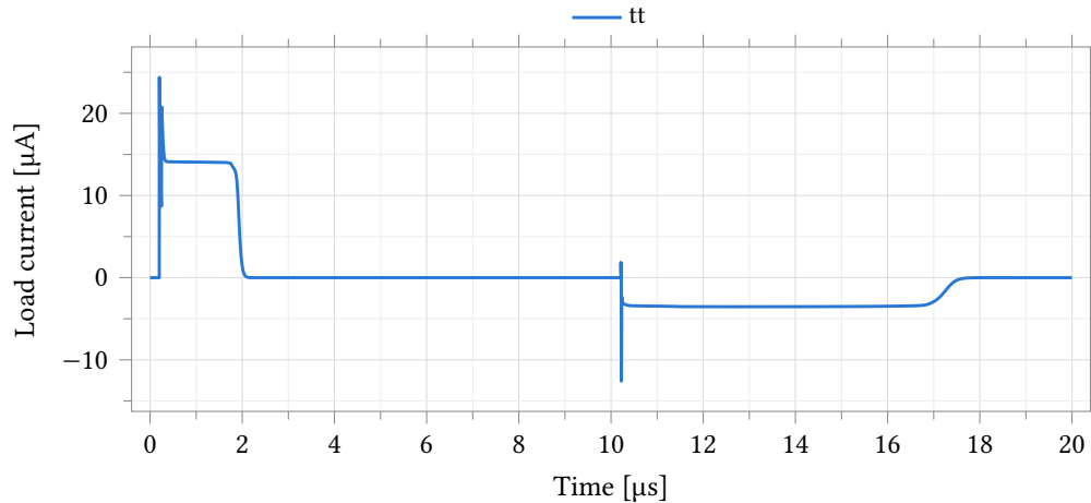
Figure 22: Current delivered into the 10 pF load during the same step, positive out of the amplifier. The asymmetry is plain: while the output slews up the cascoded PMOS mirror holds a flat 14.1 \mu\text{A} , and while it slews down the output pulls only 3.5 \mu\text{A} . The narrow spikes at each edge — 24.4 \mu\text{A} and 12.6 \mu\text{A} — last well under a microsecond; it is the flat sections that set the slew rate. These are slewing currents with the input pair overdriven past its common-mode range, so read them as the shape of the asymmetry rather than as a drive rating; see the discussion following Table 19.
