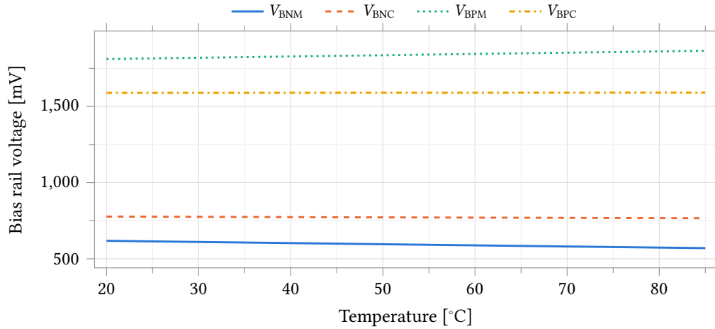
Figure 8: The four local bias rails against temperature at the typical corner. V_{\text{BNM}} and V_{\text{BNC}} are referred to v_{\text{ss}} !; V_{\text{BPM}} and V_{\text{BPC}} sit near the supply.
