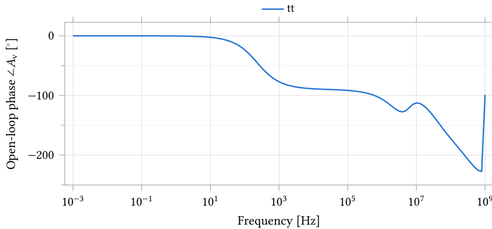
Figure 18: Open-loop phase against frequency, same conditions as Figure 17. The phase passes through -115.7^\circ at the unity-gain frequency, so the non-dominant poles have taken only about 26^\circ by the time the gain reaches unity. The step at the extreme right is an unwrapping artefact: at ten points per decade the phase moves by more than 180^\circ between the last two samples and the unwrapper cannot follow it. It is above 500 MHz, three decades past unity gain, and does not affect the margins in Table 16.
