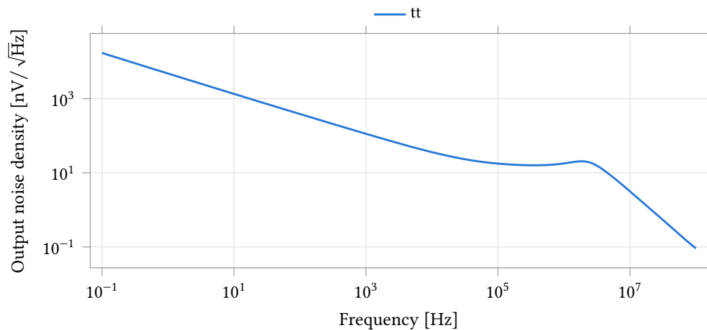
Figure 23: Output-referred noise density of the amplifier in unity-gain feedback, including the noise of the local bias generator. Flicker noise dominates below the 34 kHz corner and reaches 4.77 \mu\text{V}/\sqrt{\text{Hz}} at 1 Hz; the broadband floor is 16.0 \text{ nV}/\sqrt{\text{Hz}} , and the fall above about 2 MHz is the closed-loop bandwidth rolling the noise off, not a reduction in the noise generated.
