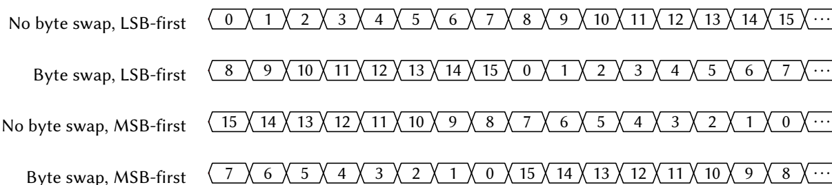
Figure 27: SPI Bit Ordering (16-bit transfer)
