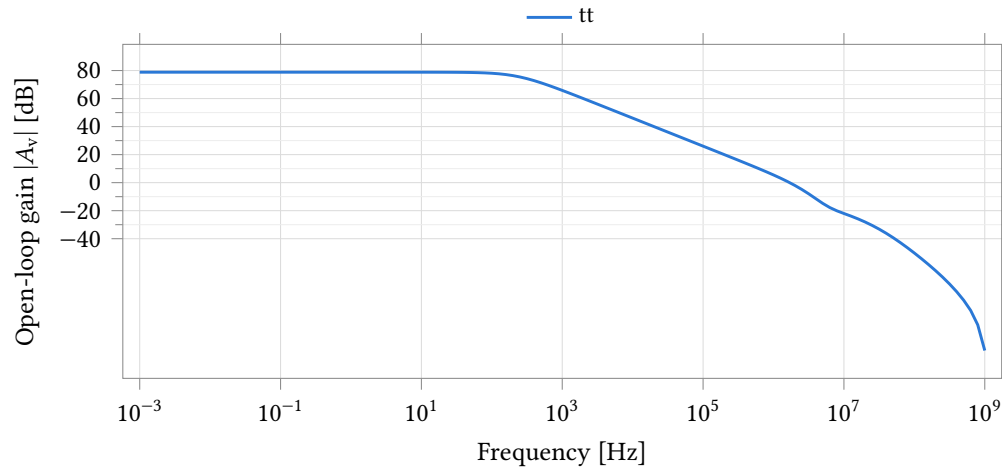
Figure 17: Open-loop gain of the control amplifier against frequency, driven differentially about 1.25 V into a 10 pF load. The gain is flat at 78.81 dB (8716) out to a dominant pole at 230 Hz and falls at 20 dB per decade to unity gain at 1.71 MHz; the single-pole roll-off across five decades is the signature of the uncompensated single-stage topology loaded only by C_L .
