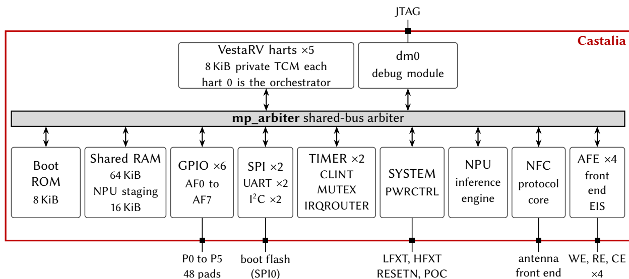
Figure 2.1: Castalia whole-chip diagram: the bus masters above the mp_arbiter bus, the memories and peripherals on one rank below it, and the package boundary in red.
