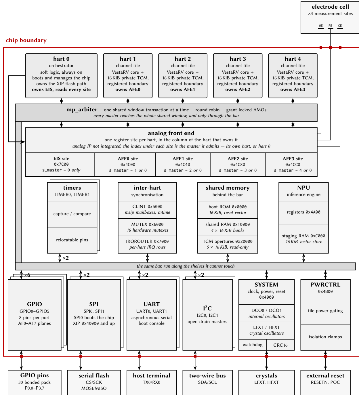
Figure 2: Castalia whole-chip diagram: the bus and the peripherals. One serializing shared-window bus reaches everything on the die, so the mp_arbiter is drawn as the grey bar every block taps — run down the margin and along the lower shelves, because one bar cannot touch three shelves without a tap crossing a box. Masters on top; the pin-facing shelf against the red package boundary, its outside world beyond it; an \times N badge is N instances of one peripheral, not one block. In the analog row the column is the ownership : a site sits under the hart that owns it, and what enforces that is the gate printed inside it — a comparison against the arbiter’s granted-master index, not a wire; hart 0’s margin arrow is the same comparison from the other side. Everything drawn is generated from this configuration.
