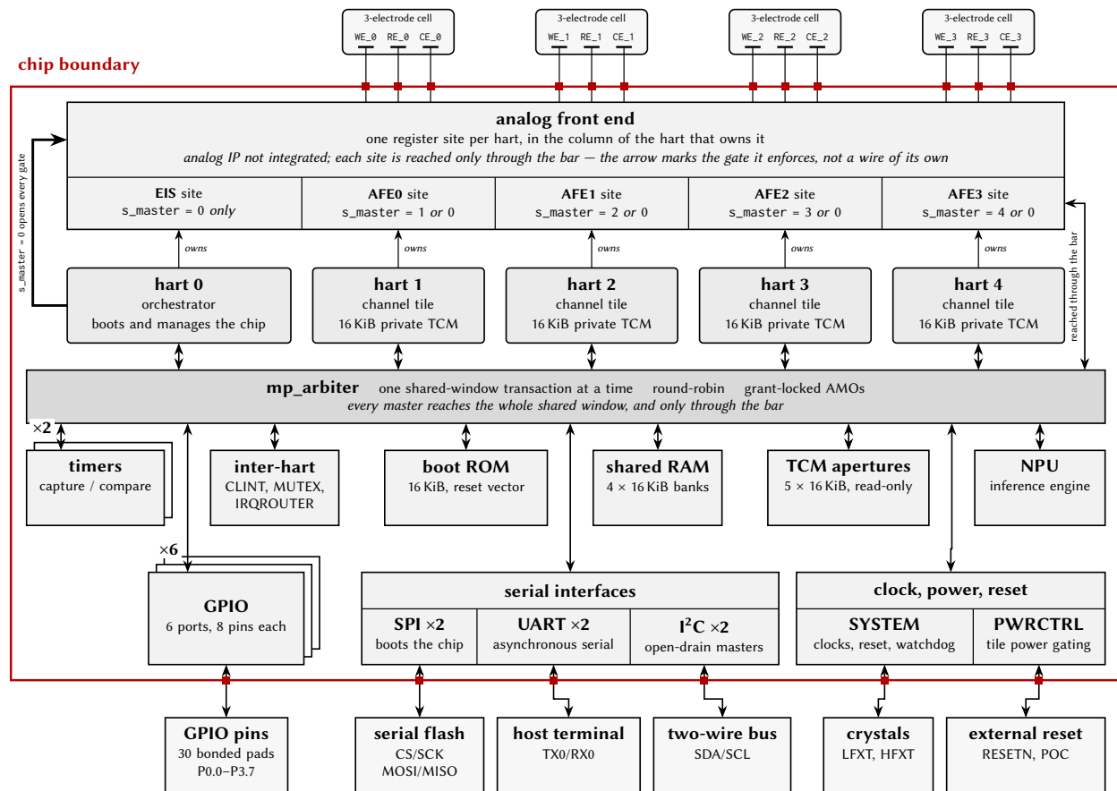
Figure 3: Castalia whole-chip diagram, flat companion to Figure 2: the same generated content on one bus bar. Every master taps the mp_arbiter bar from above and every peripheral from below — the rank against the red boundary reaches the same bar through the gaps between the rank above it, so there is one bus in this drawing and no second segment of it. Peripheral boxes carry a name and one line only; the addresses are in Section 3, and an \times N badge is N instances of one peripheral, not one block. The analog row is drawn above the harts here, each site in its owner's column with a thin owns arrow down to it: that arrow is the gate printed inside the site (a comparison against the arbiter's granted-master index), not a wire — the sites are arbiter slaves, and the drawing gives the whole row exactly one bus drop, out of its right-hand edge and down the lane beside the band. Hart 0's heavier arrow is the same comparison from the other side, over the whole row at once. Each channel brings out its own three-electrode cell across the boundary at the top. Everything drawn is generated from this configuration.
