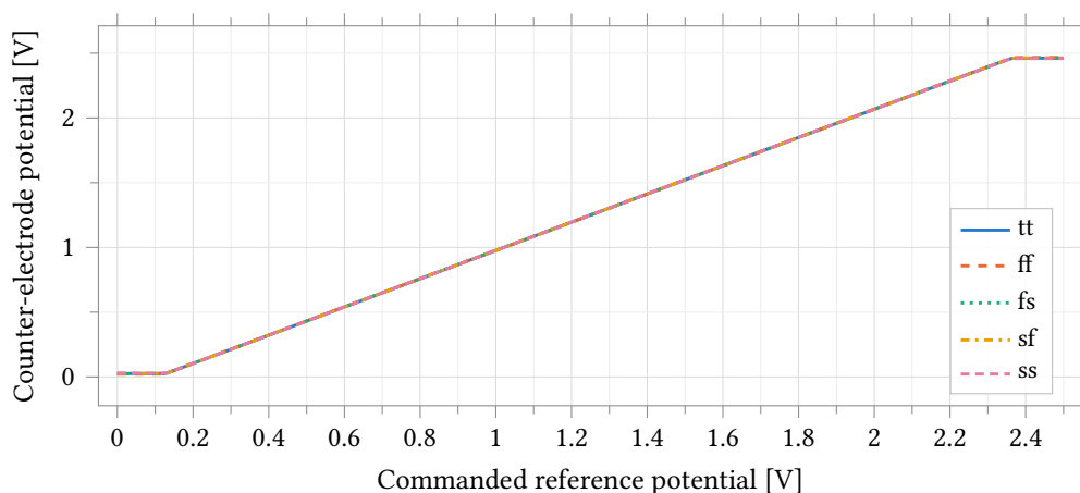
Figure 38: Counter-electrode potential against commanded reference potential over five process corners, cell-drive bench (Figure 37). The amplifier drives a Randles cell with R_{CE} = 1\text{ k}\Omega , R_u = 1\text{ k}\Omega , R_{ct} = 10\text{ k}\Omega , C_{dl} = 1\text{ }\mu\text{F} with the working electrode held at 1.25 V, C_L = 5\text{ pF} , C_c = 500\text{ fF} , 2.5 V supply; the typical point is at 37 °C and the four skew corners at 25 °C. The central segment rises with slope 12/11, the divider between the 1 k \Omega counter-electrode branch and the 11 k \Omega remainder of the cell; the flat ends are the amplifier against its rails, and their heights are the compliance limits tabulated in Table 41. Over the whole central segment the cell current is set by the cell resistance and the commanded potential, not by the amplifier.
