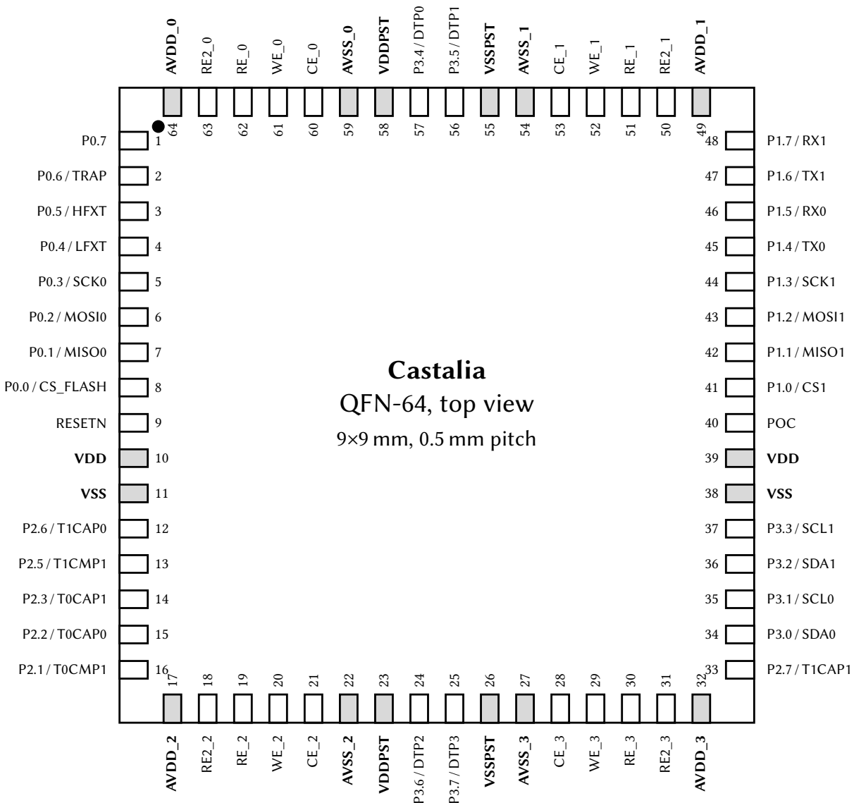
Figure 4: QFN-64 pinout, top view (9 × 9 mm, 0.5 mm pitch). Each pin is labeled with its pad name and, for GPIO pins, its AF0 (reset-selected) alternate function; power-rail pins are shaded and bold. The full per-pin alternate-function matrix is in Table 5.
