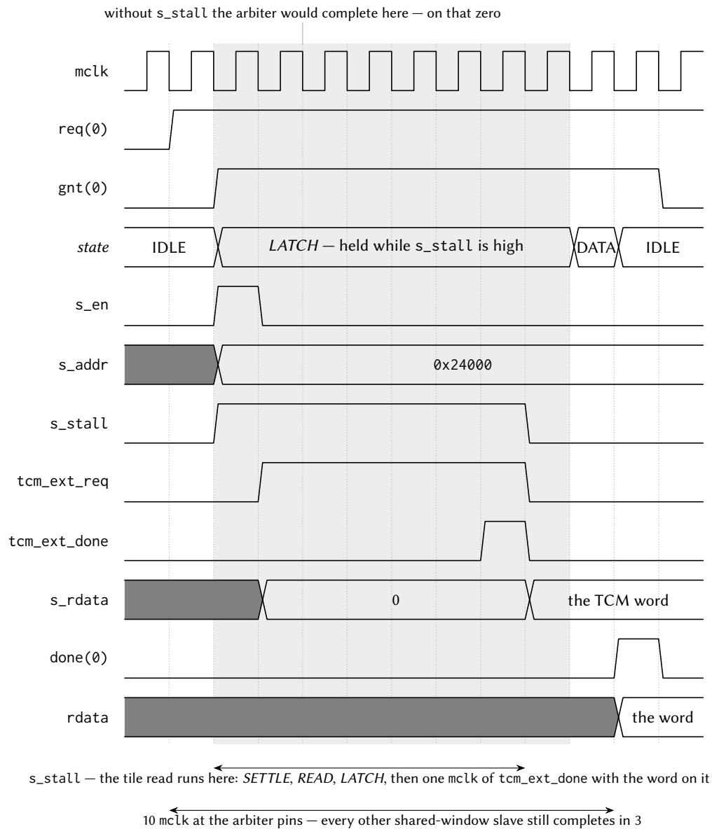
Figure 5: One stalled shared-window read: the management hart through a TCM aperture, at the same mp_arbiter pins as Figure 4. Up to the shaded region it is the ordinary walk — the grant, the one-cycle s_en strobe, the address presented. The aperture slave raises s_stall in that same cycle, and the arbiter stays in LATCH : grant pinned, address still presented, only the completion moves. Underneath, the tile's read port takes one SRAM read and returns the word on a single mclk of tcm_ext_done ; the slave captures it, drops s_stall , and the arbiter finishes the transaction it was holding. Without the stall it would have completed on the marked cycle, handing back the zero the slave had not filled in yet.
