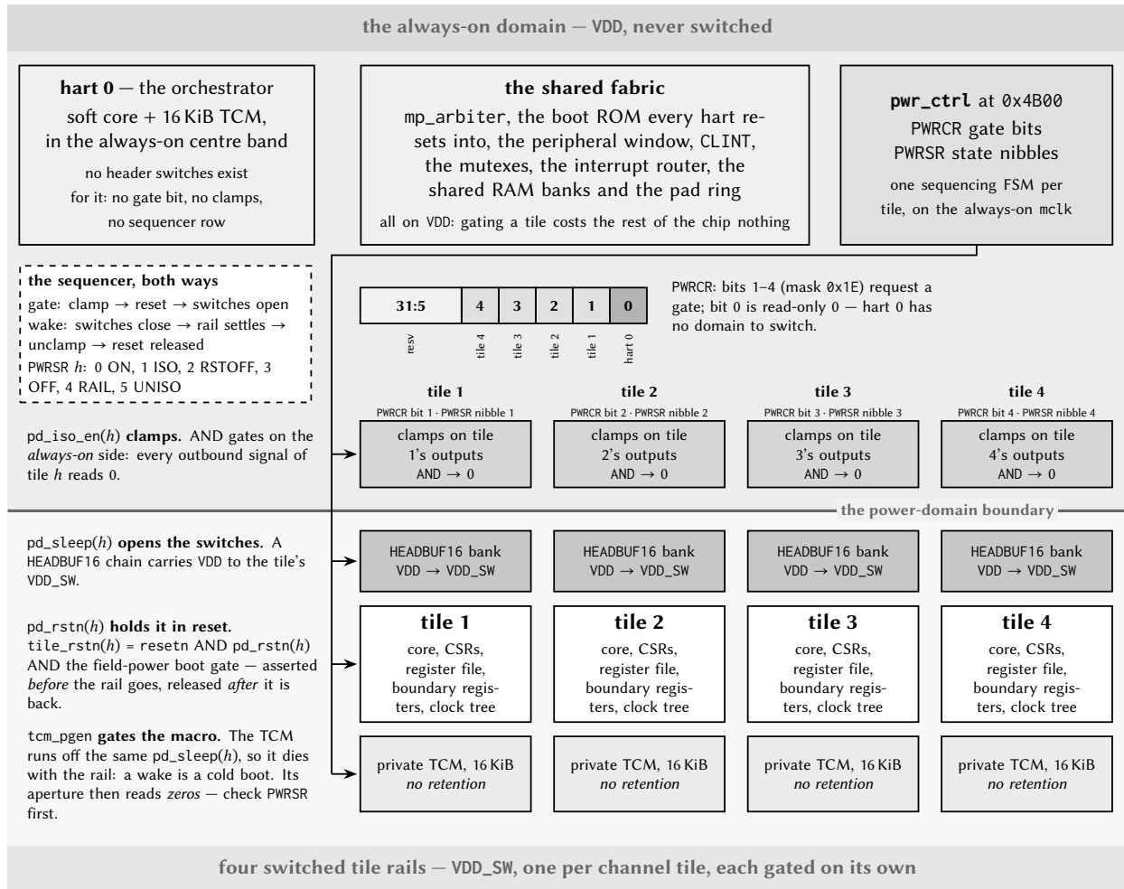
Figure 61: The chip's power domains. Everything the rest of the chip needs — the arbiter, the boot ROM, the peripherals, the shared RAM, the pad ring and hart 0 — sits on the unswitched VDD rail; each channel tile has a rail of its own. Setting PWRCR bit h walks the four layers of tile h downwards: the clamps assert on the always-on side of the boundary, the tile is held in reset, and only then do the header switches open. Clearing the bit walks them back up, and because nothing in the tile retains state, what comes back up is a cold boot.
