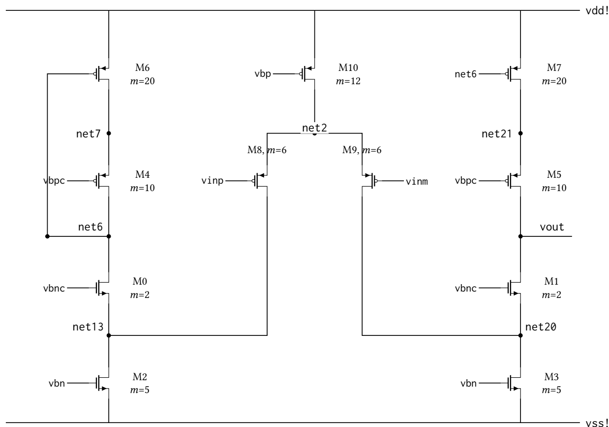
Figure 17: Control amplifier anatop_controlamp : a single-stage folded cascode with a PMOS input pair. M10 is the tail; the pair M8/M9 steers its current into the folding nodes net13 and net20 , where the NMOS sources M2/M3 sink a fixed bias current. The difference passes up through the NMOS cascodes M0/M1 into the cascoded PMOS mirror M6/M4 (diode side, gate node net6 ) and M7/M5 (output side). Output and load current are summed at vout , the single high-impedance node, so there is no internal compensation capacitor — the load capacitance sets the dominant pole. The mirror gate is drawn as a wire inside its own branch and identified by name on M7, rather than as a drawn bus. Every device is L = 700 nm, W = 6 \mu m; m is the multiplicity. Node names are the netlist's. vbn , vbnc , vbp and vbpc come from the local bias generator of Section 5.1. Omitted : the 22 ModgenDummy matched-layout dummy devices (6 NMOS, 16 PMOS), whose terminals are tied to vss! or to a folding node and which carry no signal current.
