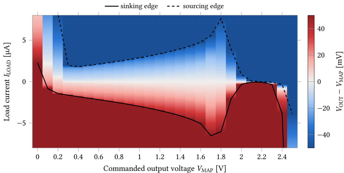
Figure 21: DC drive compliance of the control amplifier at the typical corner, as a map of the unity-gain tracking error over commanded output voltage and load current. Positive I_{LOAD} draws current out of the output, so the amplifier sources ; negative I_{LOAD} injects, so it sinks . The colour scale is clipped at \pm 50 mV, the compliance criterion: inside the envelope the error is the smooth I_{LOAD}R_O gradient, and outside it the output has hit a rail, so everything beyond the envelope saturates to solid colour. The two black curves are the |V_{OUT} - V_{MAP}| = 50 mV edges, interpolated on the 50 nA sweep at each of the 26 commanded voltages. The vertical axis is cropped to \pm 8 \mu A. Numerical values are in Table 20.
