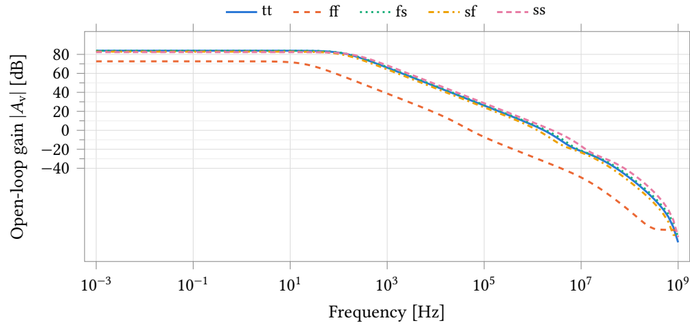
Figure 18: Open-loop gain of the control amplifier against frequency, driven differentially about 1.25 V into a 10 pF load, over all five process corners. The single-pole roll-off across five decades is the signature of the uncompensated single-stage topology loaded only by C_L ; Table 15 gives the DC gain, dominant pole and unity-gain frequency.
