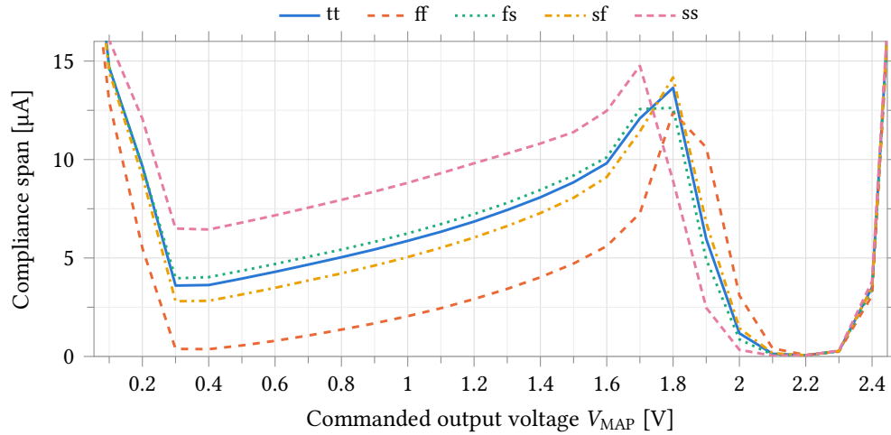
Figure 22: Width of the \pm 50 mV compliance envelope against commanded output voltage, over all five process corners. The shape is the same in every corner: pinched at both ends of the output range and widest around 1.8 V. The vertical scale is clipped at 16 \mu\text{A} ; outside roughly 0.3 V to 1.9 V the buffer no longer tracks its input at zero load, and the span plotted there is the current that forces the output onto the commanded value.
