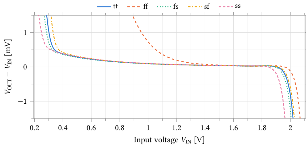
Figure 19: Unity-gain tracking error against input voltage. Inside the window 0.30 V to 2.01 V the error stays under 1 mV, passing through 61 \mu\text{V} at mid-supply; the curve leaves the frame at both ends, where the PMOS tail runs out of headroom near the supply and the output stage reaches its low limit near v_{ss} !. The vertical scale is clipped to \pm 1.5\text{ mV} so the in-range behaviour is visible at all – the error reaches 97 mV at 0 V and -382\text{ mV} at 2.5 V.
