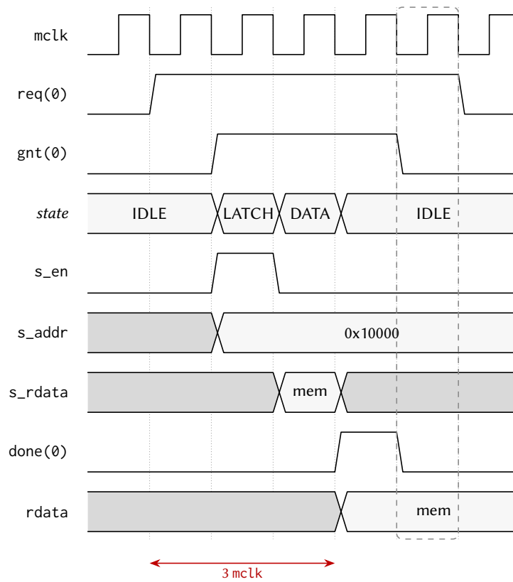
Figure 5.2: Timing diagram of one uncontended shared-window read at the mp_arbiter pins; in the dashed ghost window req is stale-high for one cycle after done and is masked by need_release.
