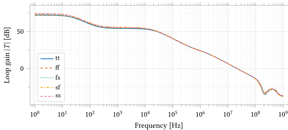
Figure 52: Potentiostat control-loop gain over five process corners, measured through the 0 \text{ V} probe IPRB1 in the RE feedback path (Figure 49). R_f = 35 \text{ k}\Omega , cell R_{ce} = R_u = 1 \text{ k}\Omega , R_{ct} = 10 \text{ k}\Omega , C_{dl} = 100 \text{ nF} , 2.5 \text{ V} supply. This is the full loop – A1, A2, both feedback networks and the electrode together – and is not the open-loop amplifier gain of Section 8.4. tt is at 37^\circ\text{C} , the four skew corners at 25^\circ\text{C} . The corner separation drawn here is a lower bound: the corner set holds the passive model rows at typical (pinned-passive caveat, page 69).
