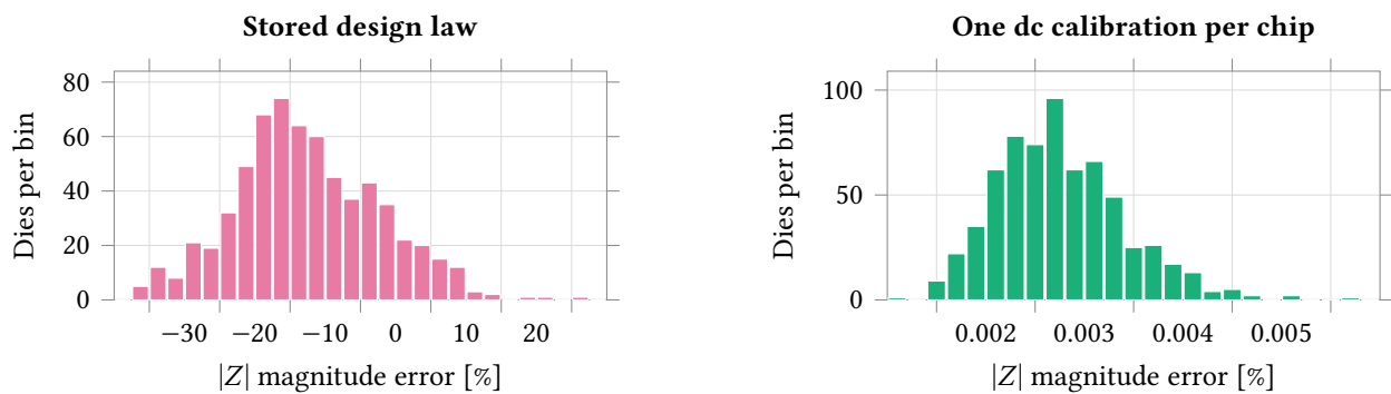
Figure 60: Impedance-magnitude error over 649 Monte Carlo dies at 0.1\text{ Hz} on the typical electrode at gain code 0, with process and mismatch together at the nominal corner and 37^\circ\text{C} , under two calibration policies: a stored 18\text{ k}\Omega + 6\text{ k}\Omega N design law (left) and one dc measurement of the feedback resistance per chip (right). \sigma falls from 10.24\% (95% interval 9.71 to 10.83 ) to 0.00065\% ( 0.00061 to 0.00068 ), a factor of 1.6 \times 10^4 , and the right panel is indistinguishable from measuring the current at every frequency — the bound, which needs a current reference the die does not carry. The two x-axes are independent and are not to be compared by eye: the left spans 70\% and the right 0.005\% , and both are the same 649 dies, load, gain code and run. The plotted range is that run's own, -32.1\% to +30.6\% , and not a union over the campaign; no sample is censored. The statistical model section holds the capacitor family at typical, so the 22\text{ pF} feedback capacitor does not vary here and the figure bounds the feedback resistance rather than the pole — which matters because 0.1\text{ Hz} is below that pole, and above it a dc calibration stops working at all.
