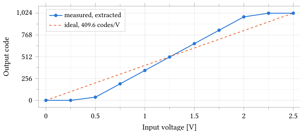
Figure 63: Output code against input voltage for the extracted anatop_pixel_adc, nominal corner, 37 °C, 2.5 V analog and 1.0 V digital supplies, with the ideal 409.6 codes/V line overlaid. The transfer is monotonic and reaches both code limits, but its slope is 628.64 codes/V — 1.535 times ideal — so the flat segments below 0.44 V and above 2.07 V are the code limits, not the ends of the sweep. Markers are the eleven simulated points; the 0.25 V step is 157 codes, so the curve between them is interpolation and carries no linearity information.
