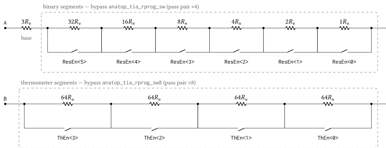
Figure 67: Segment and bypass-switch structure of anatop_tia_rprog , transcribed from the executed spec-run netlist. The unit R_u is one series poly resistor; from terminal A the chain runs through the never-switched three-unit base, the six binary-weighted segments of 32 down to 1 unit, and the four identical 64-unit thermometer segments to terminal B. Each switched segment is shunted by a CMOS transmission gate with a local inverter: the control pin EnBar is the ResEn/ThEn bit itself and drives the PMOS pass gate directly and the NMOS pass gate through the inverter, so a bit at 1 turns both pass devices off and inserts the segment. The pass pair has multiplicity 4 in the binary switch ( _sw ) and 8 in the thermometer switch ( _sw8 ), which halves the thermometer gates' on-resistance where up to six binary gates close at a seam. Three grounded dummy units accompany the 322 active units for matching.
