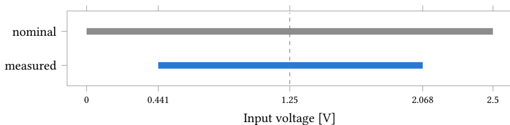
Figure 65: Usable input window of the converter against the nominal 0 V to 2.5 V supply span. The measured window runs 0.441 V to 2.068 V, 1.627 V wide, so 34.9 % of the nominal span is unreachable — 0.441 V at the bottom and 0.432 V at the top, near enough symmetric about the 1.25 V common mode (dashed). Outside that window the output sits at a code rail, so a transimpedance swing wider than \pm 0.81 V about V_{CM} is truncated rather than digitised.
