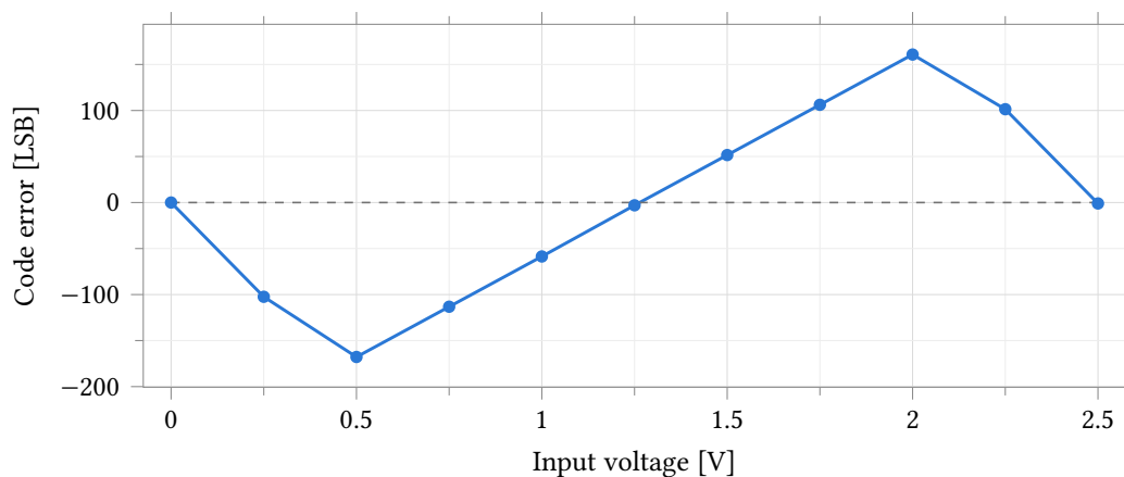
Figure 64: Code error against input voltage — measured code minus the ideal 409.6 codes/V line — from the same run as Figure 63. The error is the 1.535 slope ratio, not nonlinearity: it reaches -167.8 LSB at 0.5 V and 160.8 LSB at 2.0 V, crossing zero near the 1.25 V common mode where the measured and ideal lines intersect. It also returns near zero at 0 V and 2.5 V, where the clipped output coincides with the ideal endpoints; those two points are not accuracy. Referred to the fitted line instead, the residual over 0.5 V to 2.0 V is at most 0.52 LSB.
