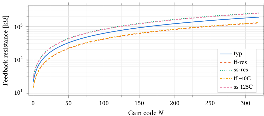
Figure 68: Measured resistance against gain code at all five corners, 500 nA forced through the A–B terminals with B held at V_{CM} = 1.25 V. The law is R = 18 \text{ k}\Omega + 6 \text{ k}\Omega \cdot N with N the binary value of ResEn<5:0> plus 64 per set ThEn<3:0> thermometer bit; every corner is strictly monotonic over all 320 codes, including the four thermometer seams. The corner families move the absolute value by -33 to +35 %, which is the poly sheet-resistance tolerance and must be absorbed by gain calibration, not by code choice.
