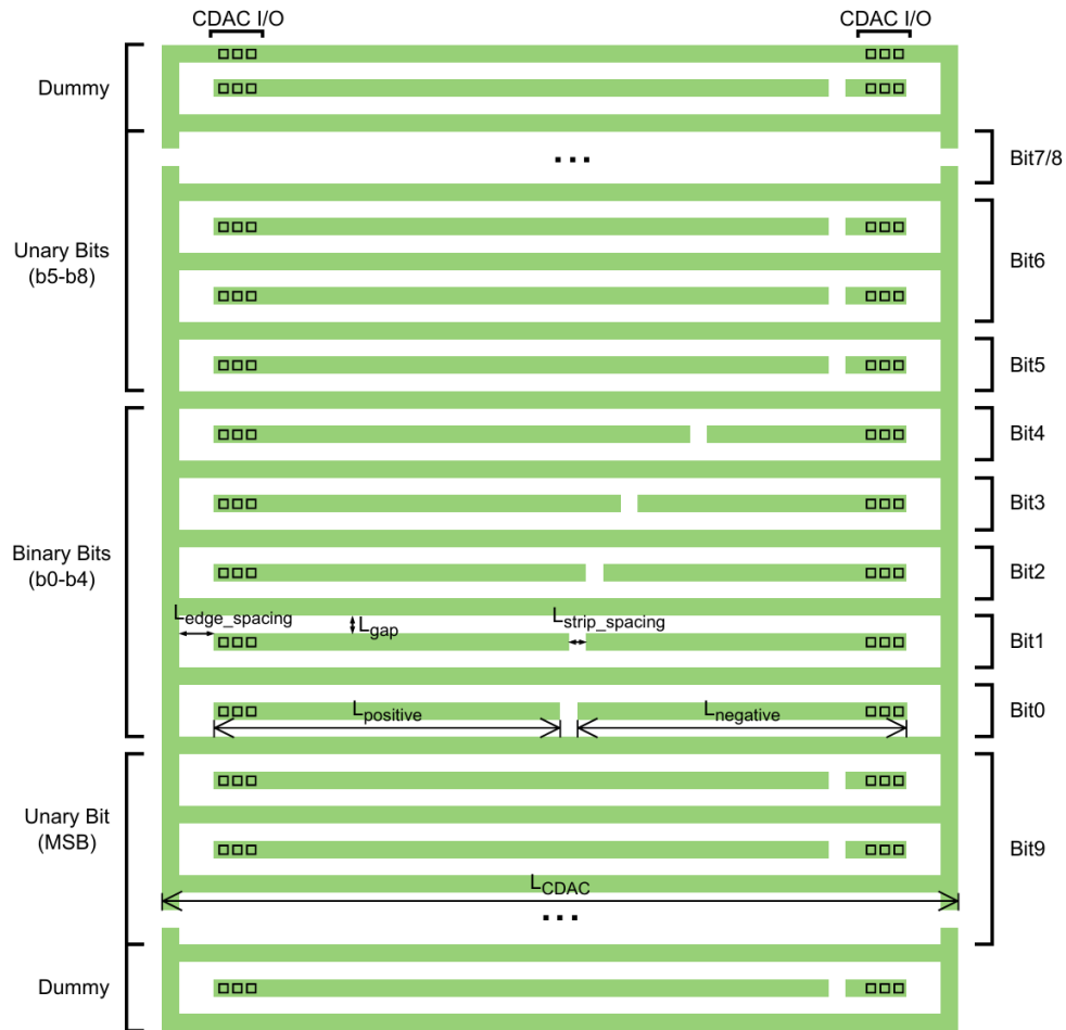
Figure 62: Floor plan of the 10-bit segmented capacitor array of anatop_pixel_adc . The five lower bits b0–b4 are binary-weighted within single strips, each strip split into a positive and a negative section whose boundary sets the weight; the upper bits b5–b8 and the MSB b9 are unary, built from repeated identical strips, and every row terminates in CDAC I/O at both ends. Unary segmentation of the large weights makes their ratio a count of identical unit strips rather than the dimension of one large device, so it is set by matching; the dummy rows at the top and bottom of the array give the outermost active strips the same local surroundings as interior ones. The array exists only in layout, which is why this section’s data is taken from an extracted netlist.
