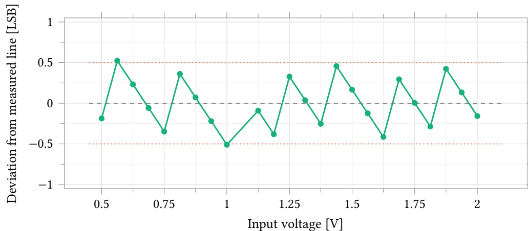
Figure 66: Deviation of each measured code from the converter's own best-fit line, 628.64 codes/V, over a 0.0625 V sweep of the unclipped window. Referred to its own scale rather than the nominal one the converter is straight to 0.523 LSB worst case and 0.294 LSB rms, so the 168 LSB of Figure 64 is gain error alone and carries no linearity information. The worst point sits just outside the \pm 0.5 LSB dotted guides. Twenty-four points 39 codes apart bound the deviation at the sampled inputs; a DNL or INL measurement needs every code and this grid does not provide one. A twenty-fifth point at 1.0625 V is absent because its simulation returned an error.
