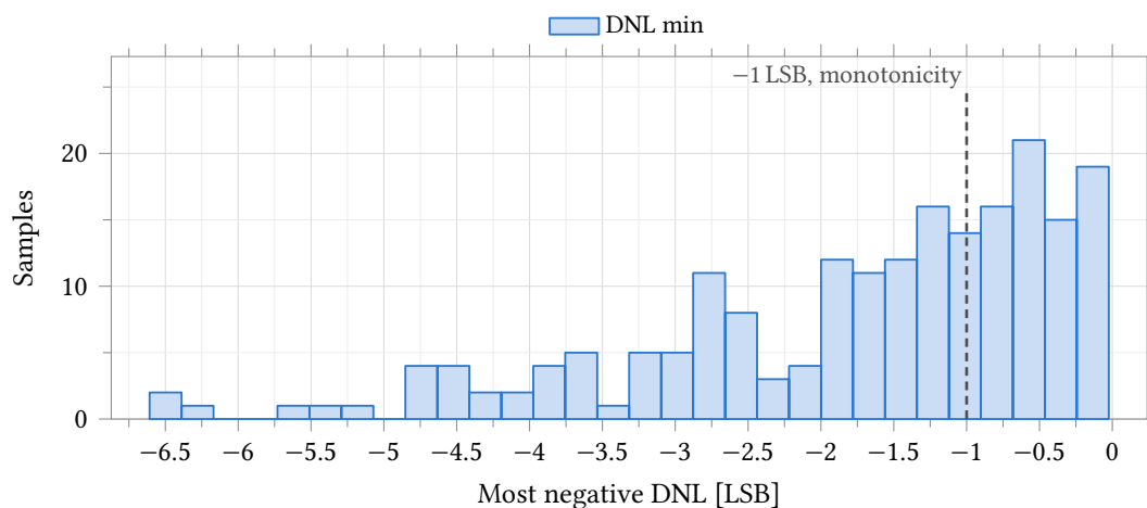
Figure 80: Worst negative differential nonlinearity, same bench, samples and conditions as Figure 79. The dashed rule at -1 LSB is the monotonicity limit entered on the test: 80 of 200 samples clear it, so 40 % of channels are monotonic and 0.40^4 = 2.6 % of four-channel chips are monotonic on all four. The distribution is left-skewed (skew -1.11 ) with a tail to -6.608 LSB, so the median -1.318 LSB and the percentiles of Table 79 describe it and \text{mean} \pm 3\sigma does not.
