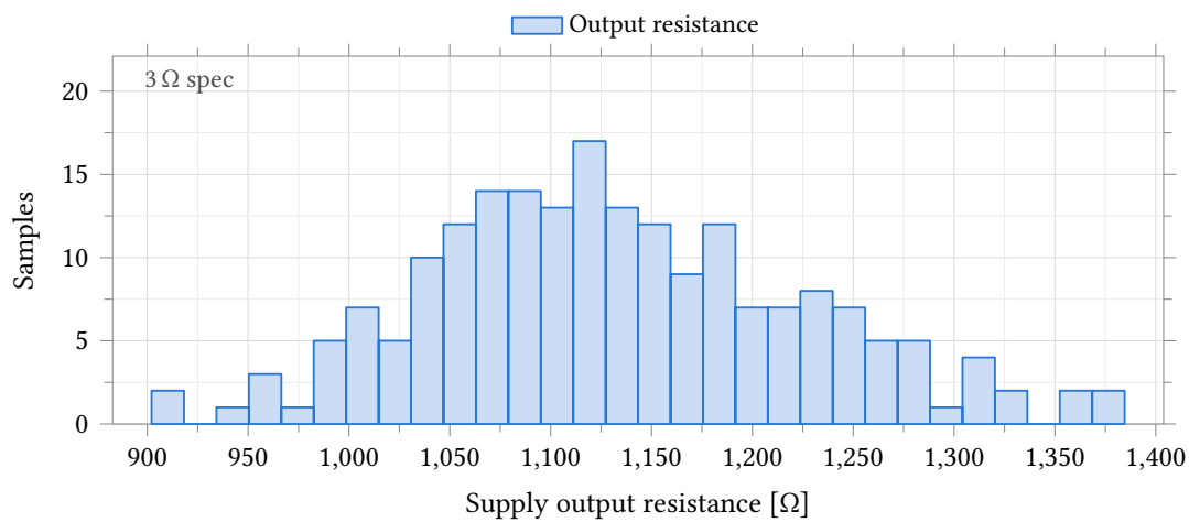
Figure 83: Output resistance of the DAC supply block, taken as the chord \Delta V / \Delta I over a 0 \mu A to 100 \mu A load sweep on VddDac. Process and mismatch , castalia_pm_25, 200 samples, 27 °C. The 3 \Omega limit entered on the test is two orders of magnitude below the data and is annotated at the left axis edge rather than drawn; no sample meets it. This is not a second defect: the reference movement of Figure 81 is this impedance multiplied by the ladder’s own code-dependent reference current.
