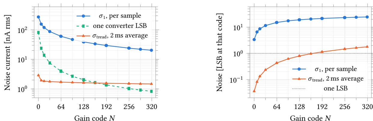
Figure 59: Input-referred current noise of the assembled channel against gain code, at the nominal electrode ( C_{\text{dl}} = 100 \text{ nF} , R_{\text{ct}} = 1 \text{ M}\Omega ), nominal process point, 37^\circ\text{C} , integrated from 0.1 Hz to 10 MHz and referred by the measured in-loop transimpedance. \sigma_1 is one converter sample; \sigma_{\text{tread}} is the average of the 1738 samples taken inside one 2 ms staircase tread, by the exact Dirichlet integral of the same spectrum — not \sigma_1/\sqrt{N} , which the transient-noise measurement of Section 8.6.6 finds wrong by up to 6.7 \times . Left, in current: the averaged floor is 1.5 nA to 2.9 nA and barely moves with gain, while one LSB falls 98 \times , so the two cross at N \approx 165 and every code above it is noise- rather than quantisation-limited. Right, the same referred to the LSB at each code; a single sample is never better than 3.4 LSB, which is why the readout average is part of the specification and not an option. The feedback capacitor does not appear here: it divides output noise and transimpedance by the same factor and leaves the input-referred quantity unchanged to four digits.
